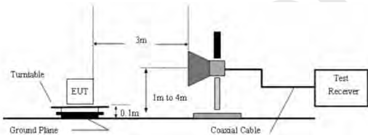
Figure 3. Above 1 GHz
