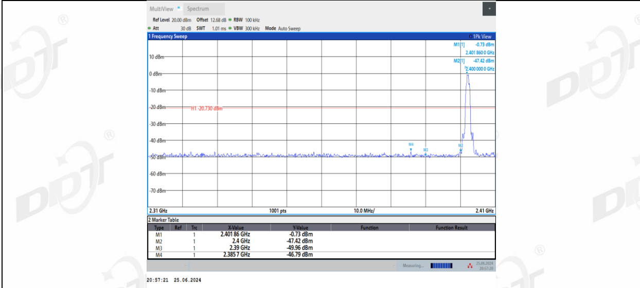
3DH5_Left side_Low_2402
