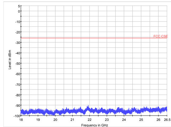
802.11g CH11 18GHz to 26.5GHz
