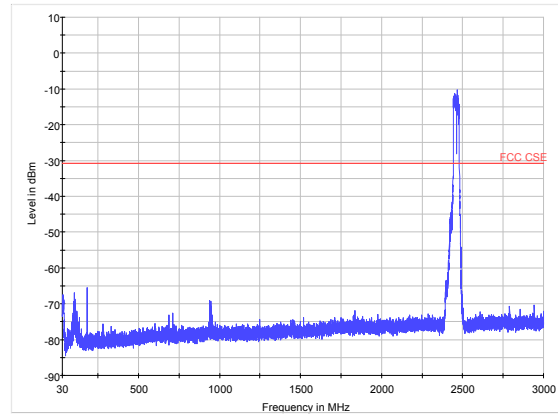
802.11n (HT40) CH9 30MHz to 3GHz
