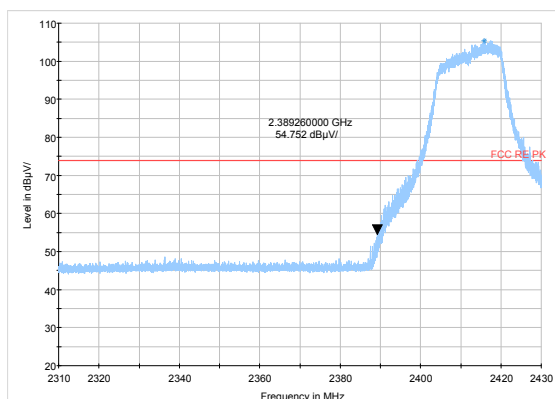
802.11g-Channel 1: Peak
