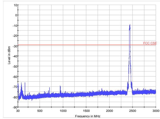
802.11n (HT20) CH6 30MHz to 3GHz
