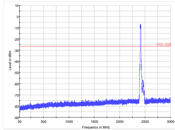
802.11g CH1 30MHz to 3GHz
