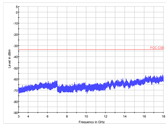
802.11n (HT40) CH3 3GHz to 18GHz
