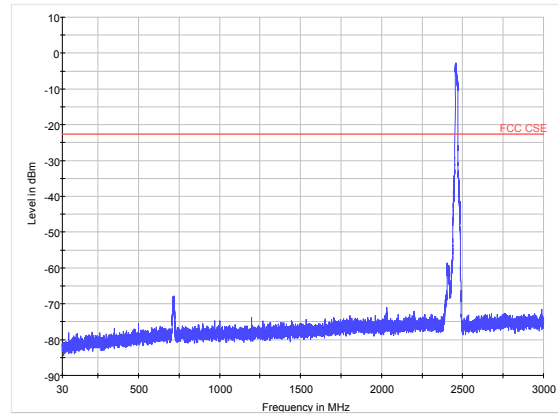
802.11g CH11 30MHz to 3GHz
