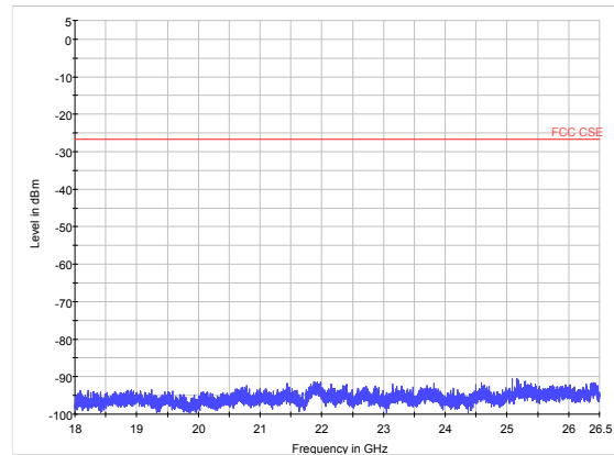
802.11g CH1 18GHz to 26.5GHz
