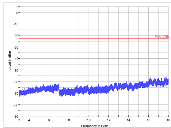
802.11g CH11 3GHz to 18GHz
