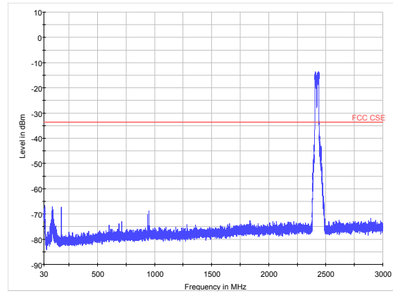
802.11n (HT40) CH3 30MHz to 3GHz
