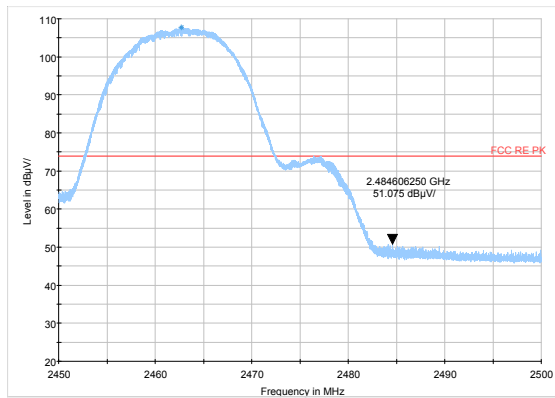
802.11b-Channel 11: Peak
