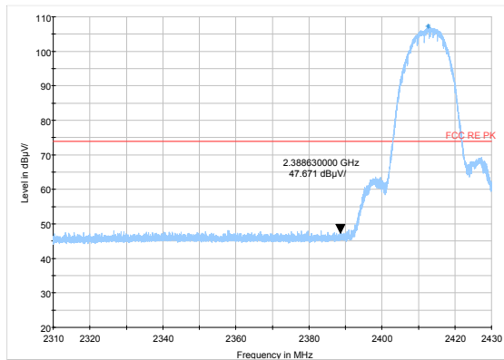
802.11b-Channel 1: Peak
