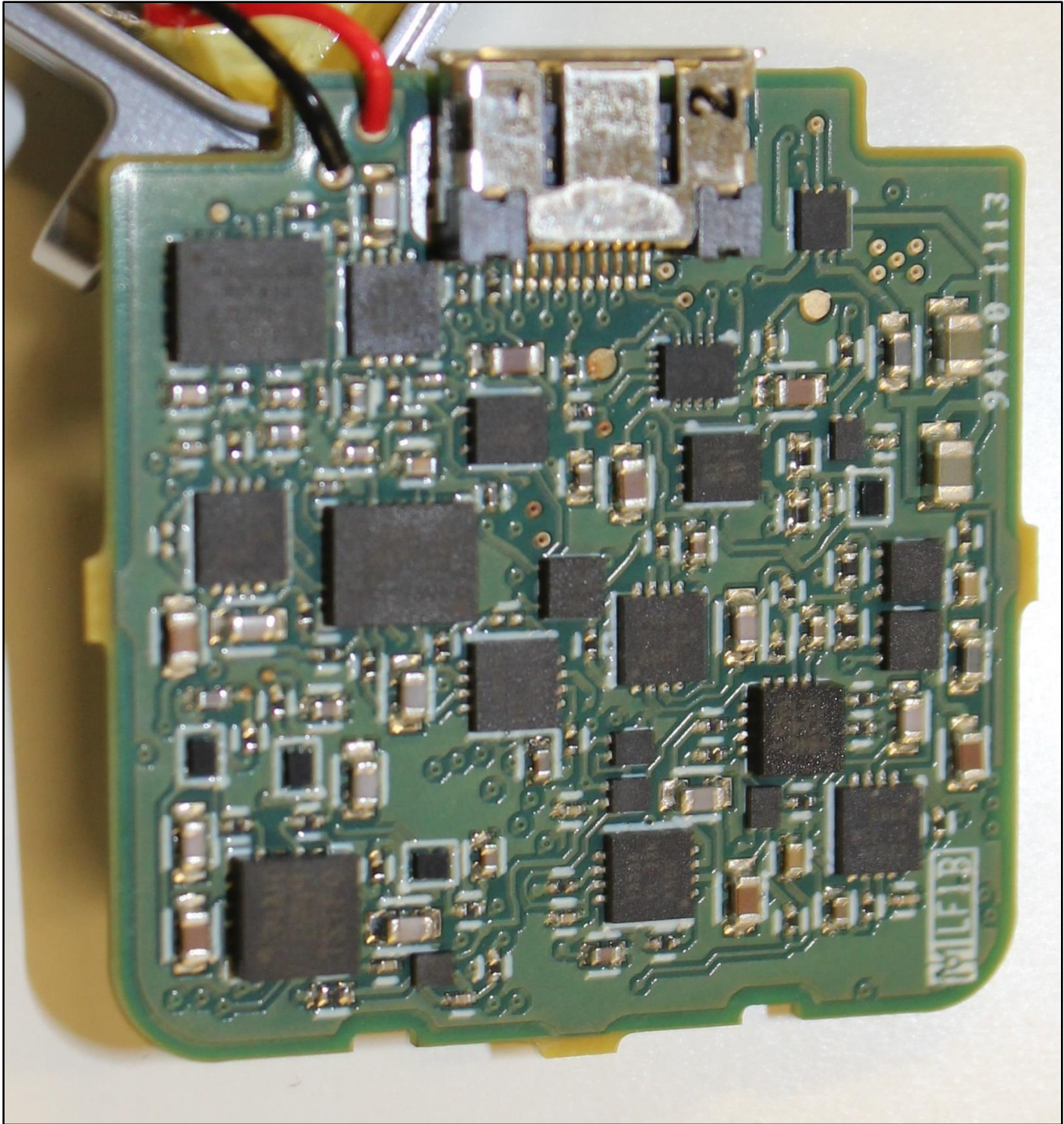
Figure 2: OPAL-V1 bottom of PCBA
