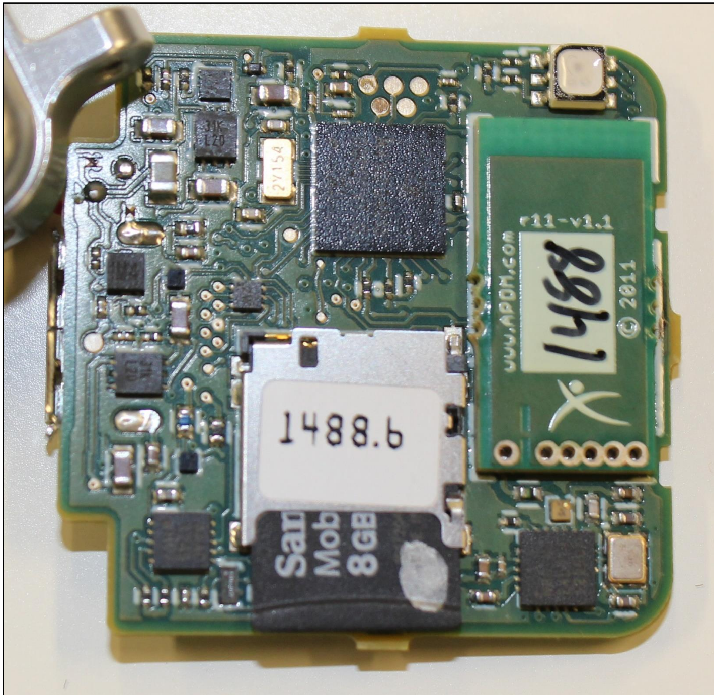
Figure 1: OPAL-V1 top of PCBA
