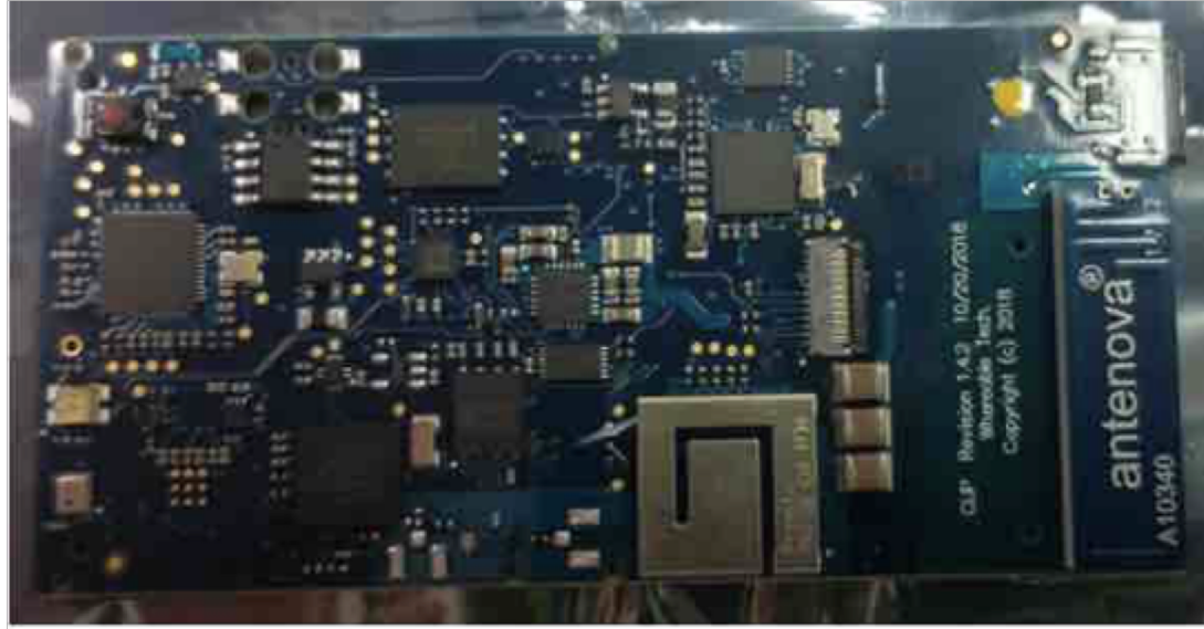
RB Clip Inside Image PCBA Topside
