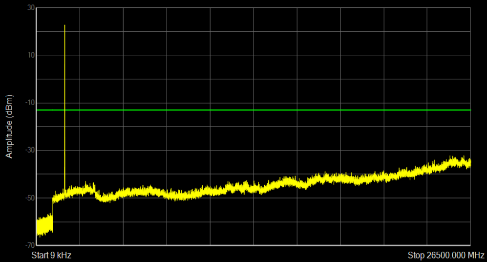
Band66 QAM16 BW=5MHz Channel=132322 RB Size=25 Position=#0
