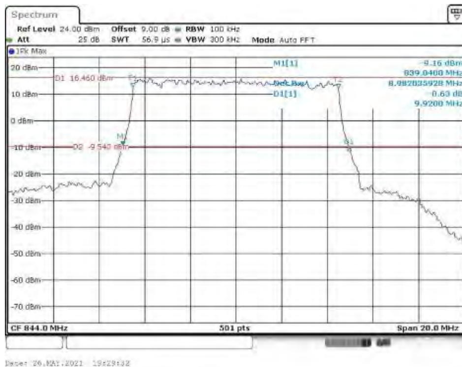
Band 5(Band 26) 10 MHz High 16QAM RB50#0
