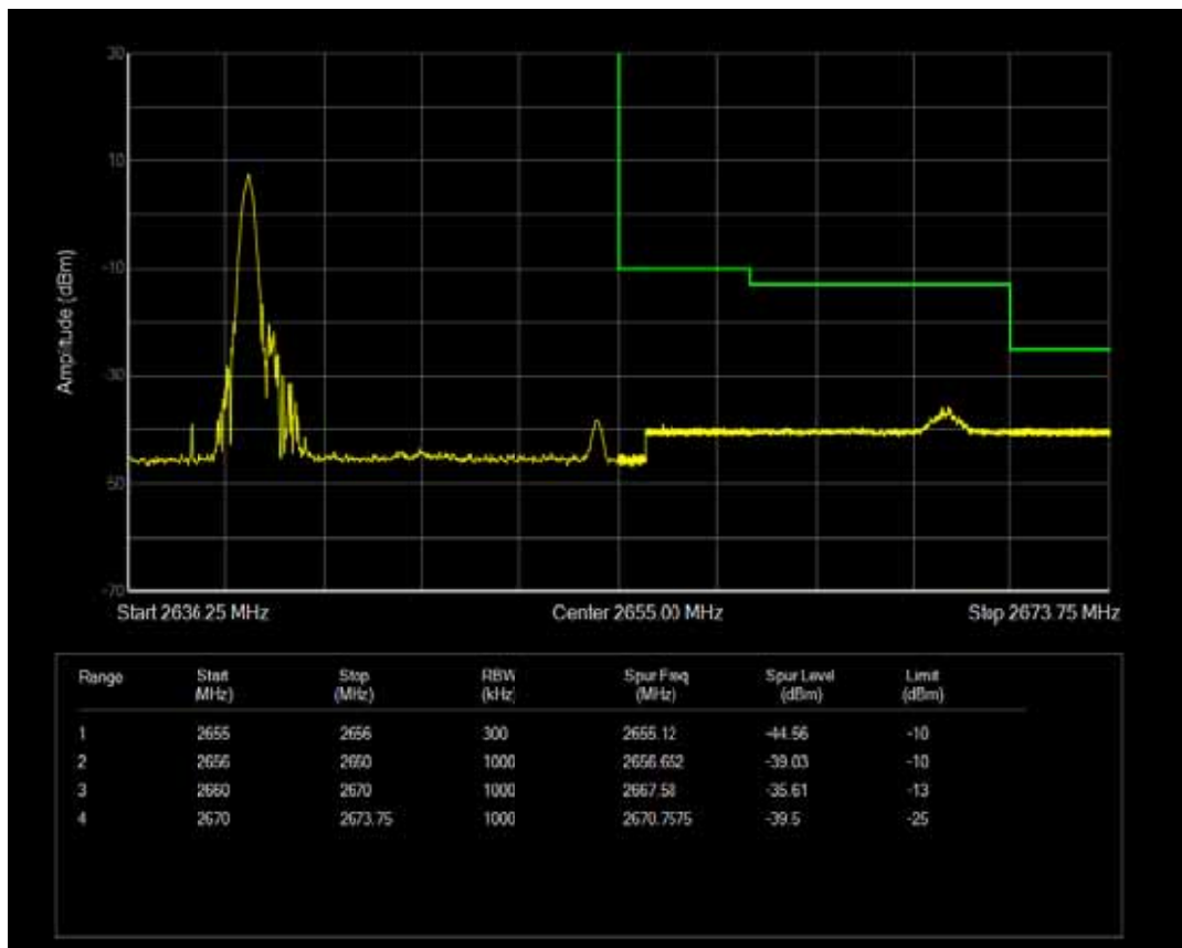
Band41 QAM16 BW=15MHz Channel=41165 RB Size=1 Position=#Max
