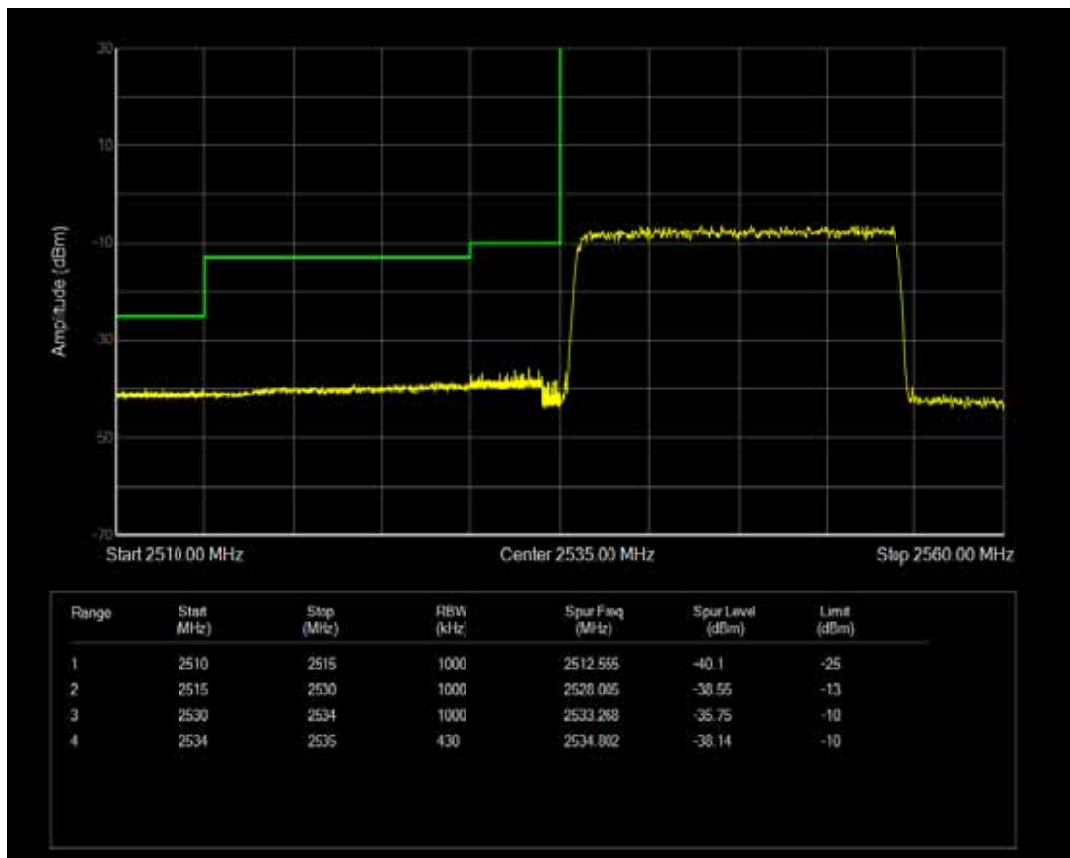
Band41 QPSK BW=20MHz Channel=40140 RB Size=1 Position=#Max
