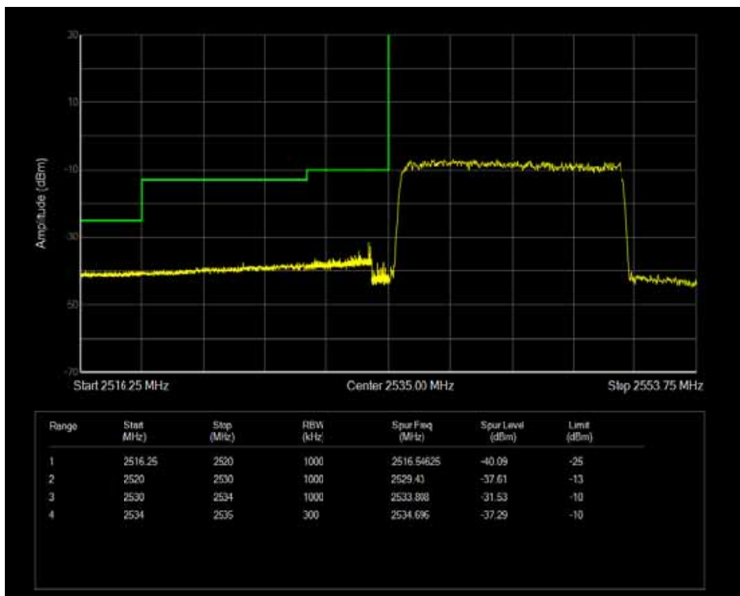
Band41 QAM16 BW=15MHz Channel=40115 RB Size=1 Position=#Max
