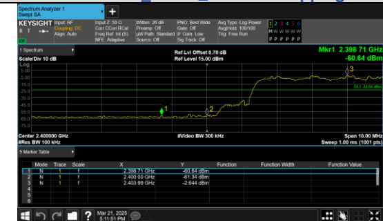
Out Of Band Emission(Left) π/4DQPSK_2-DH5_Channel Hopping
