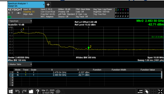
Out Of Band Emission(Right) π/4DQPSK_2-DH5_Channel Hopping
