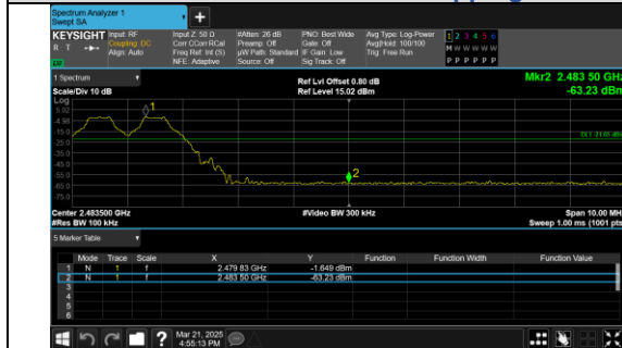
Out Of Band Emission(Right) GFSK_DH5_Channel Hopping
