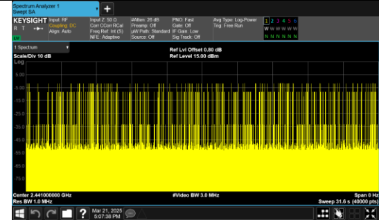
Number of Pulses in 31.6 seconds \pi/4 DQPSK_2-DH5
