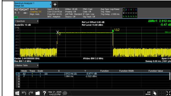
Pulse Width GFSK_DH5
