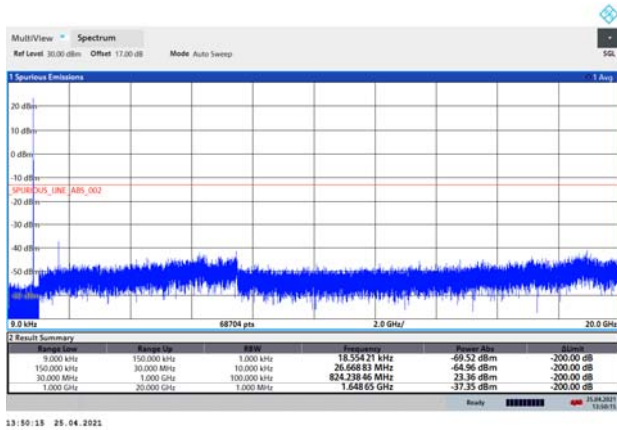
LTE Band 5 1.4MHz CH-Middle 9kHz~20GHz
