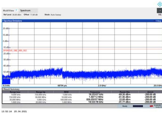
LTE Band 5 1.4MHz CH-High 9kHz~20GHz
