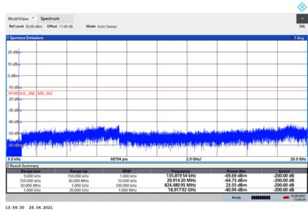
LTE Band 5 3MHz CH-Middle 9kHz~20GHz
