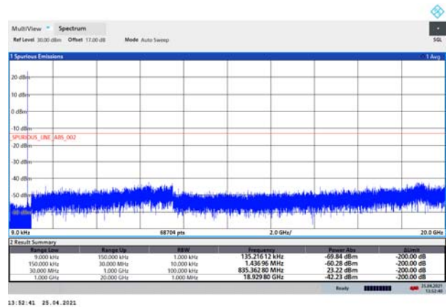
LTE Band 5 3MHz CH-High 9kHz~20GHz
