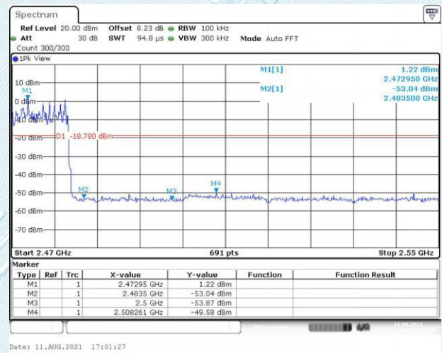
3DH5(2480)-Hopping on
