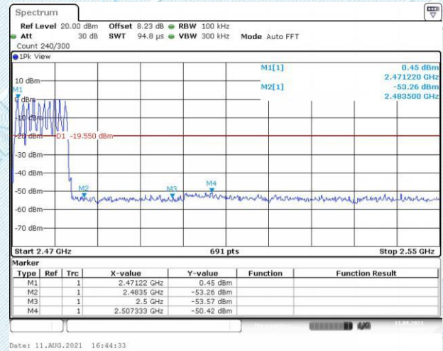
2DH5(2480)-Hopping on
