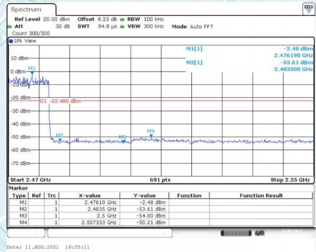
3DH5(2480)-Hopping on
