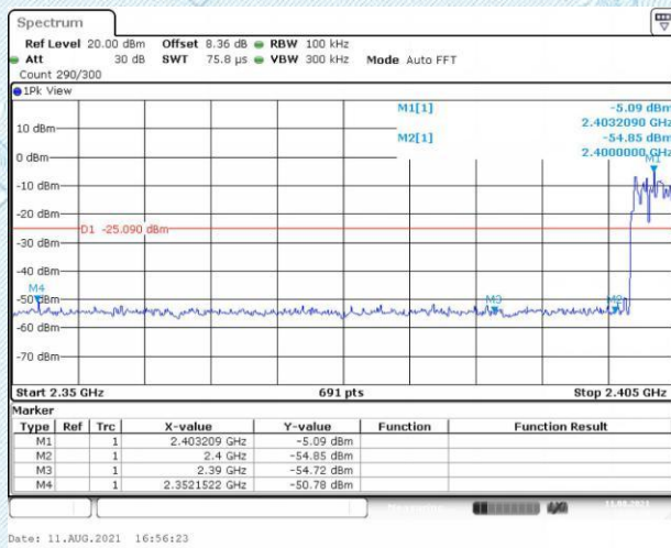
3DH5(2402)-Hopping on
