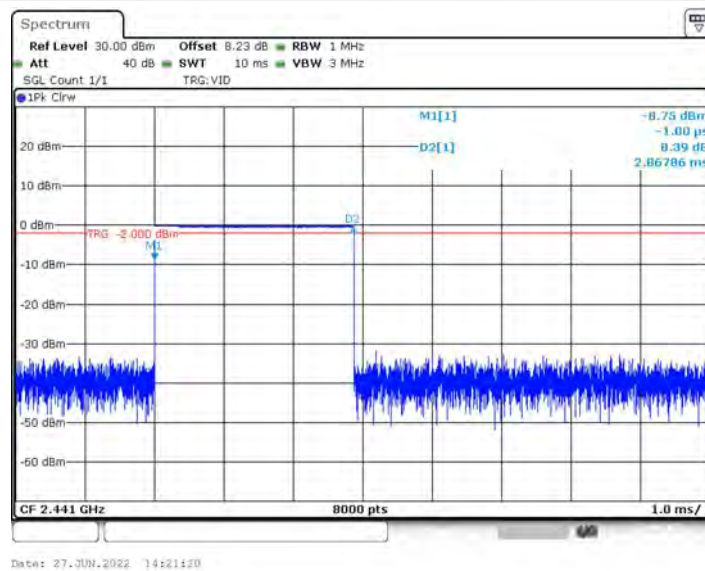
GFSK mode-DH5
