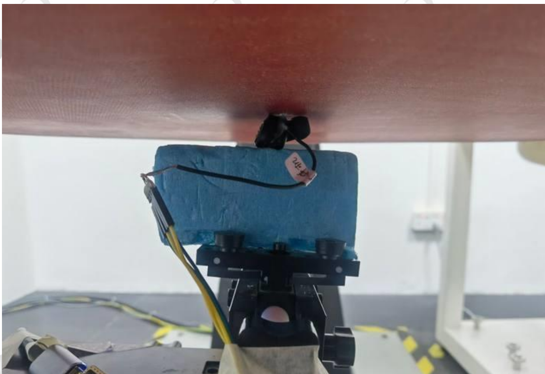
Right Side-0mm
