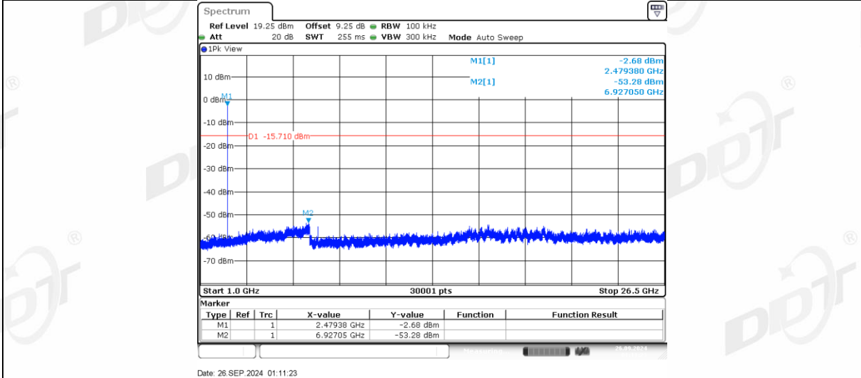
2DH5_Ant2_R_2480_0~Reference
