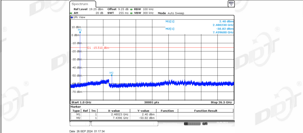
3DH5_Ant2_R_2480_0~Reference
