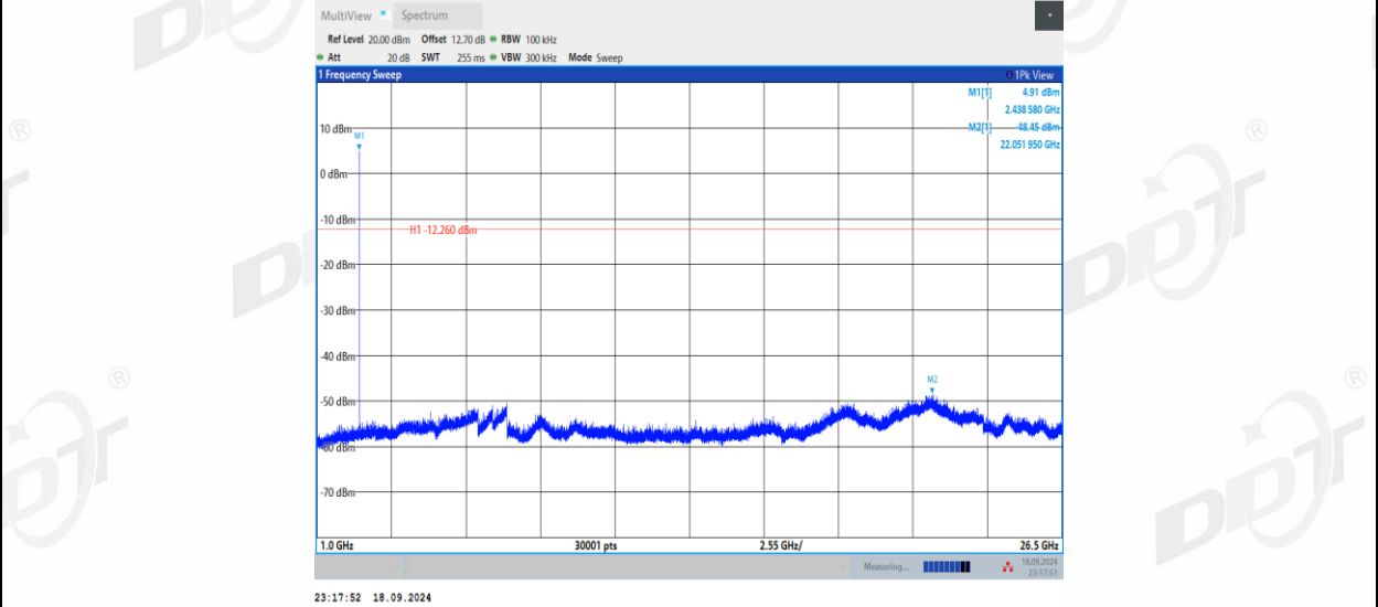
SRD_Ant1_2479_0~Reference
