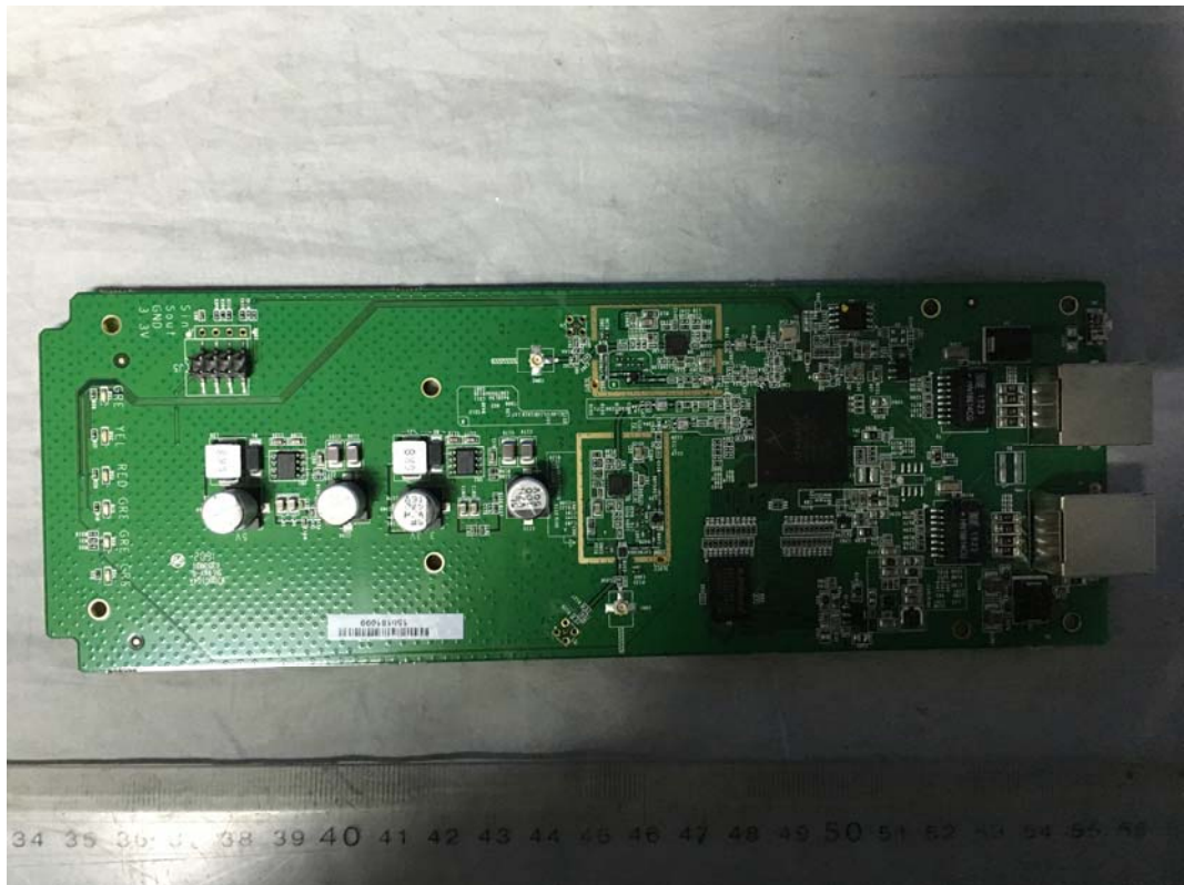
FIGURE 7 INTELLIGENT WIRELESS TRANSMISSION EQUIPMENT (M/N: TB5E) RF CIRCUIT ON MAINBOARD
