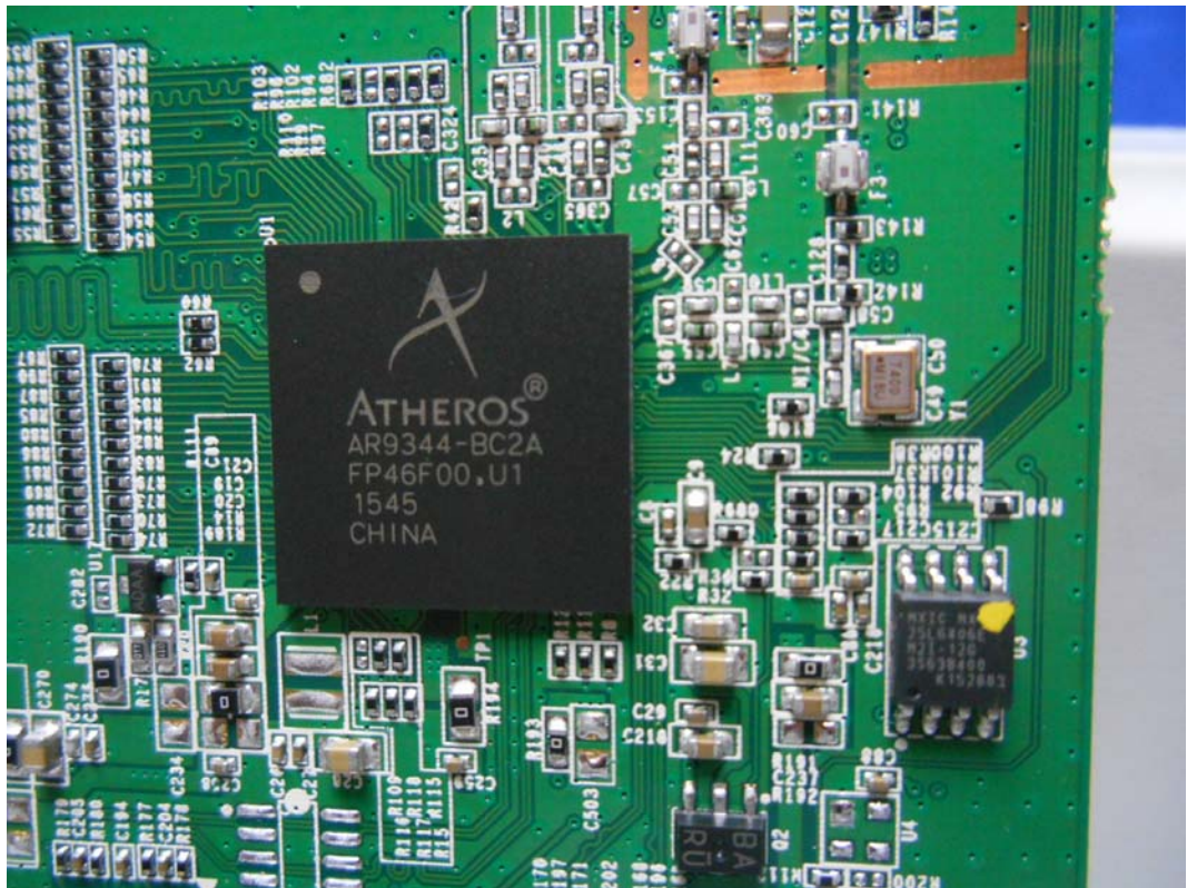
FIGURE 8 INTELLIGENT WIRELESS TRANSMISSION EQUIPMENT (M/N: TB5E) CHIP & CRYSTAL ON MAIN BOARD
