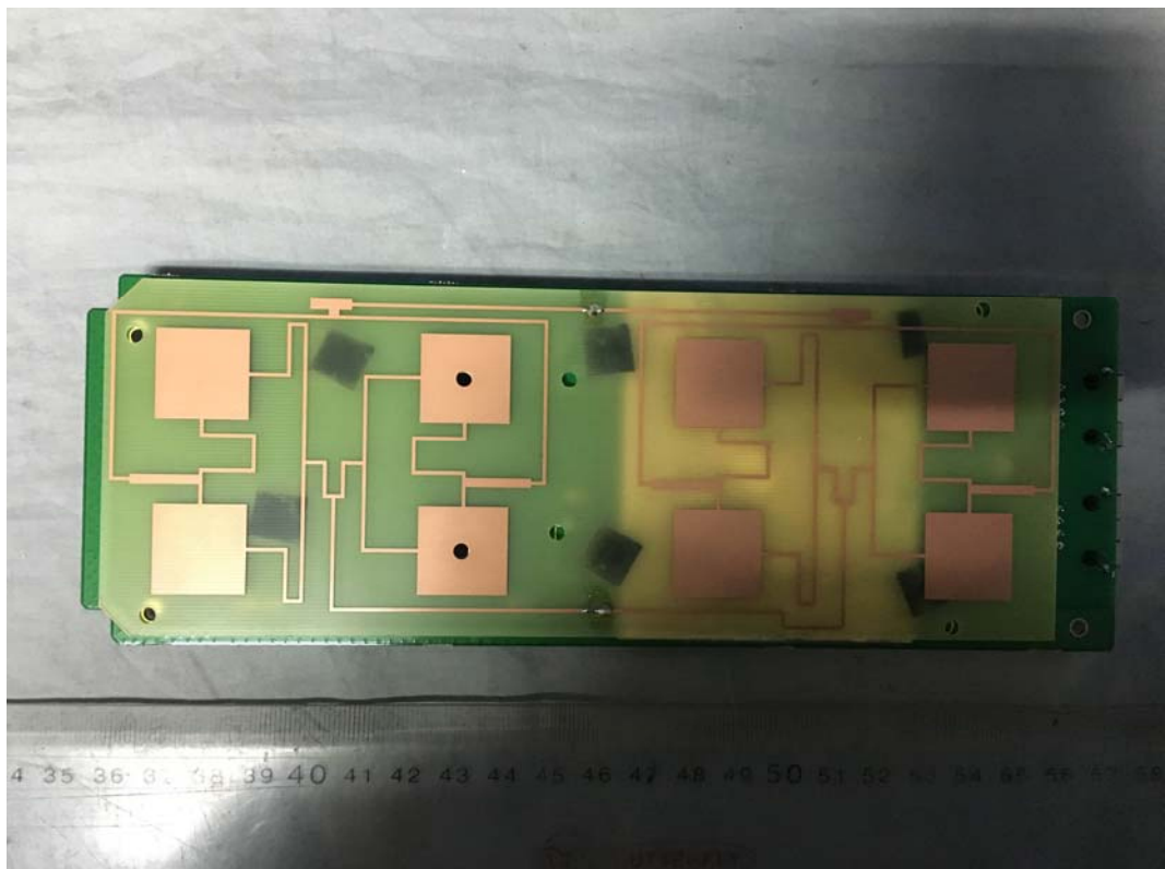
FIGURE 9 INTELLIGENT WIRELESS TRANSMISSION EQUIPMENT (M/N: TB5E) ANTENNA
