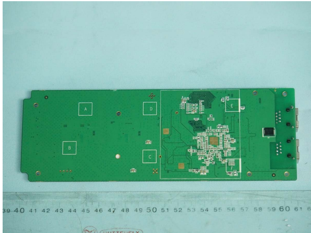
FIGURE 10 INTELLIGENT WIRELESS TRANSMISSION EQUIPMENT (M/N: TB5E) MAIN BOARD (SOLDERED SIDE), ANTENNA REMOVED
