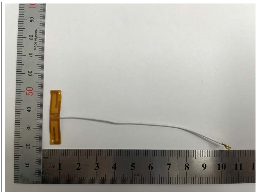
<FPCB Antenna>
