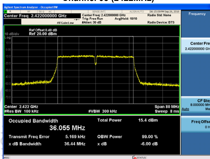
Channel 03 (2422MHz)
