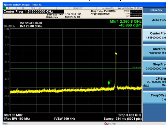
Channel 03 (2422MHz)
