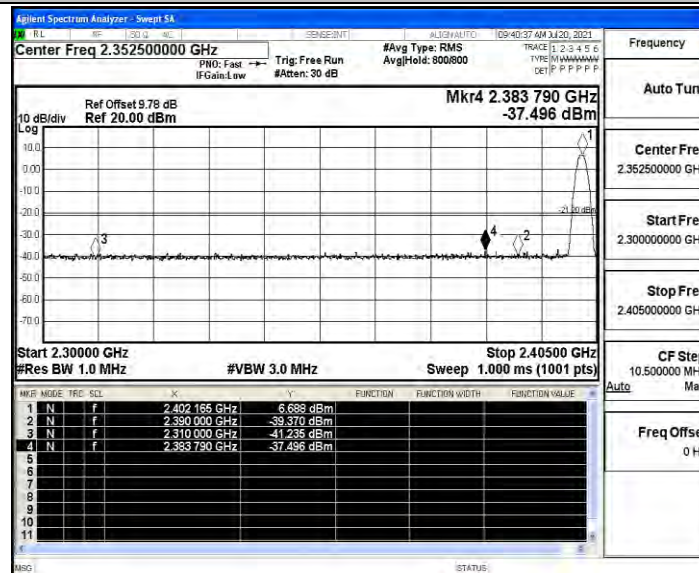
2DH5_Ant1_Low_2402_Peak
