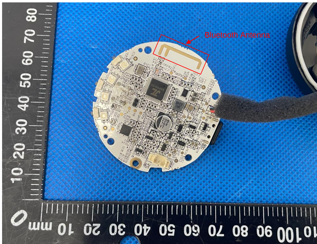
Fig. 4. PCB view -2
