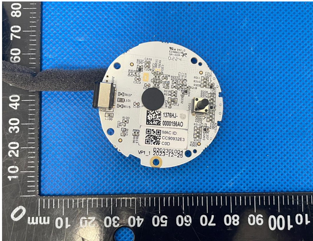
Fig. 3. PCB view -1
