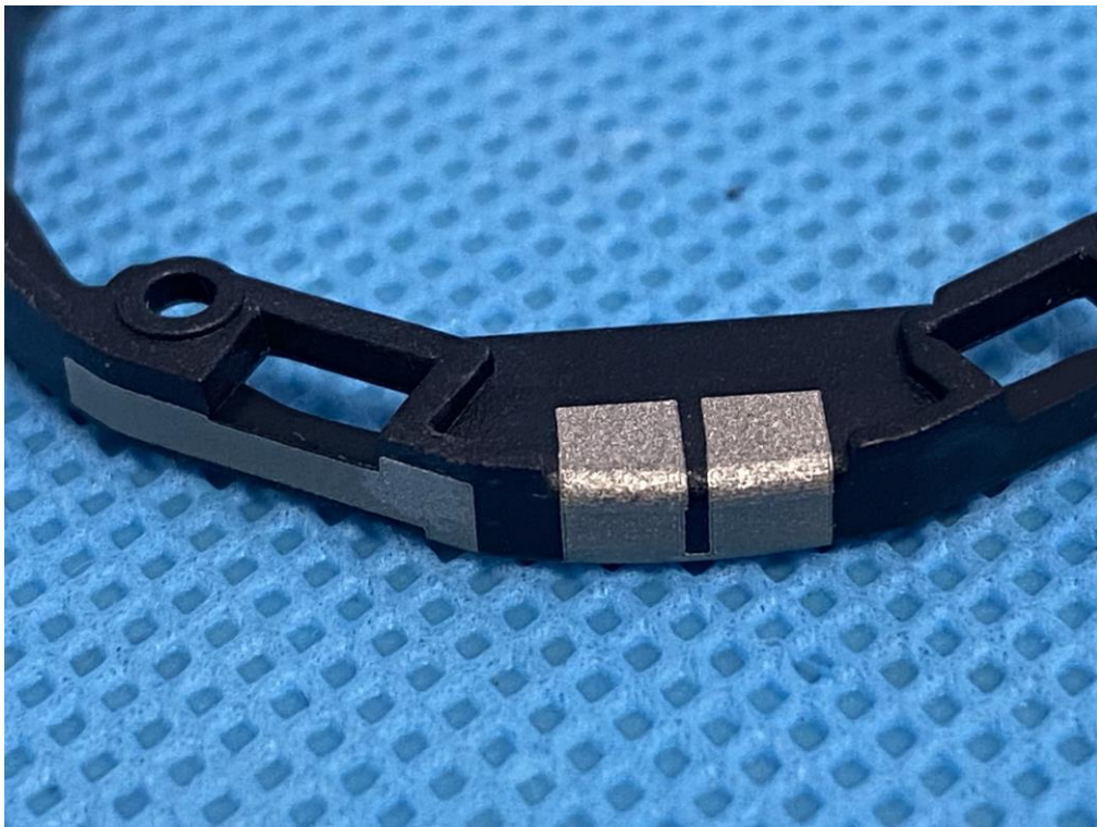
INTERNAL VIEW-2 OF EUT(BT Antenna)
