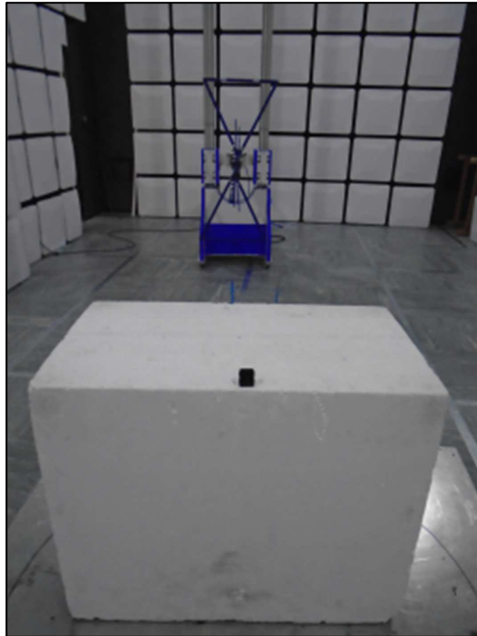
Figure 2 – Radiated Emissions 30 MHz to 1 GHz – Y Axis
