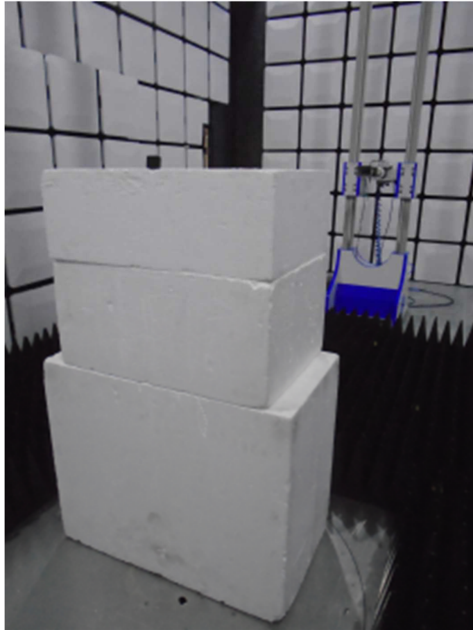
Figure 6 – Radiated Emissions 1 GHz to 18 GHz – Z Axis
