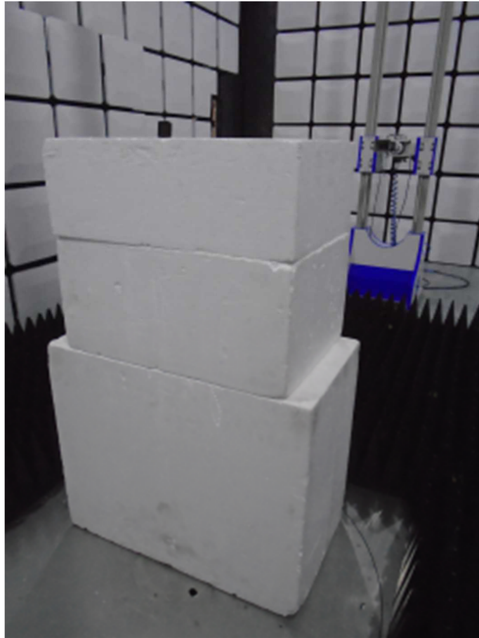
Figure 4 – Radiated Emissions 1 GHz to 18 GHz – X Axis
