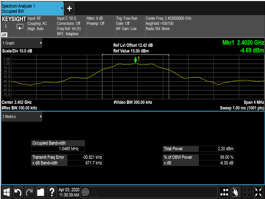
Figure 65 - 2402 MHz – 6 dB and 99% Occupied Bandwidth
