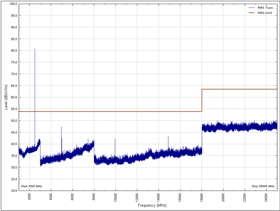
Figure 48 - 2480 MHz , 1 GHz to 25 GHz, Horizontal, X Orientation, Average
