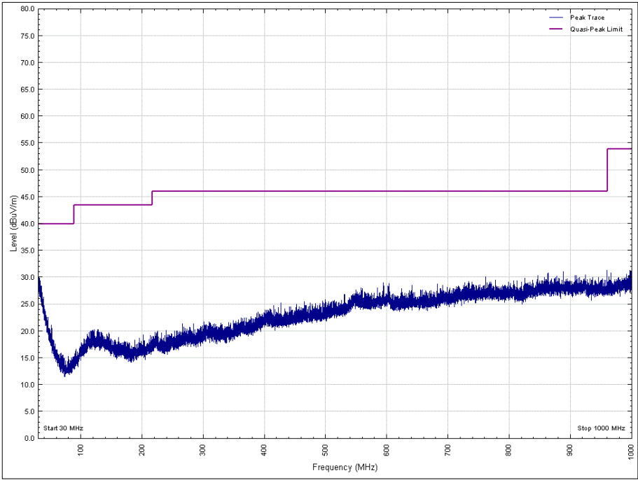
Figure 4 - 2402 MHz, 30 MHz to 1 GHz, Horizontal, X Orientation
