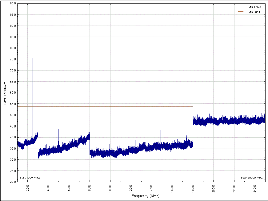
Figure 46 - 2480 MHz, 1 GHz to 25 GHz, Vertical, X Orientation, Average
