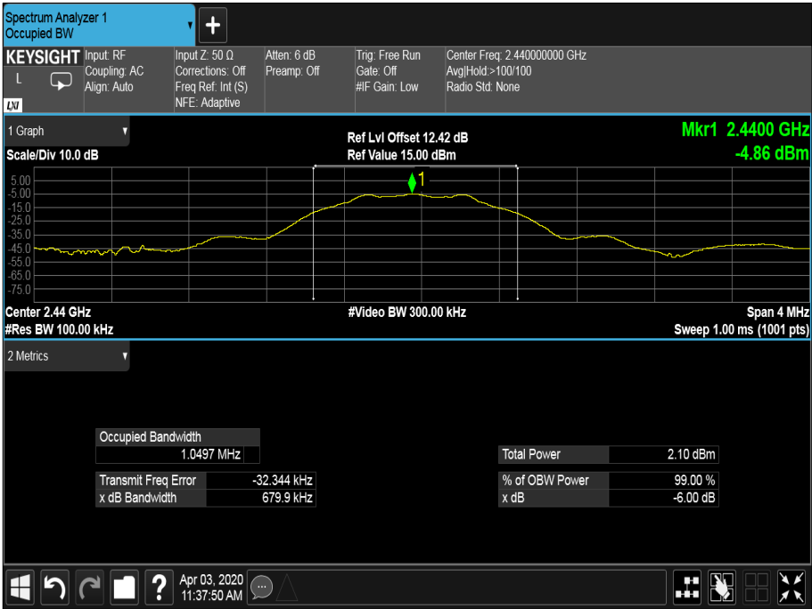
Figure 66 - 2440 MHz – 6 dB and 99% Occupied Bandwidth
