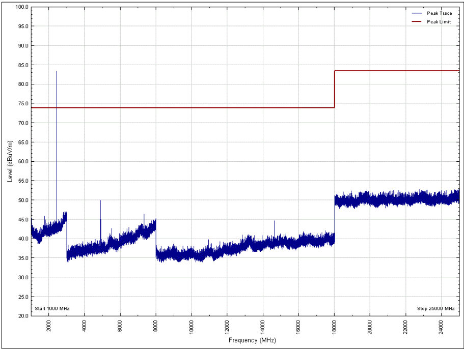
Figure 35 - 2440 MHz, 1 GHz to 25 GHz, Vertical, Z Orientation, Peak
