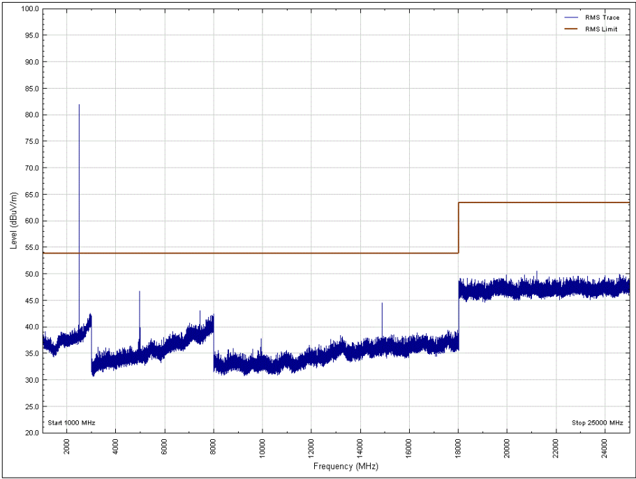
Figure 54 - 2480 MHz, 1 GHz to 25 GHz, Vertical, Z Orientation, Average
