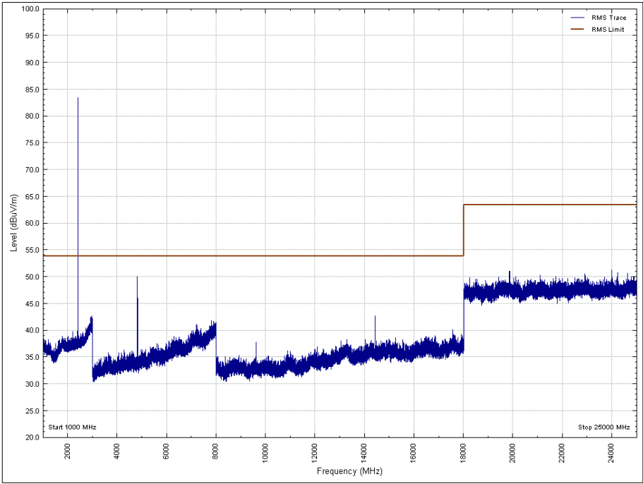
Figure 12 - 2402 MHz , 1 GHz to 25 GHz, Horizontal, X Orientation, Average
