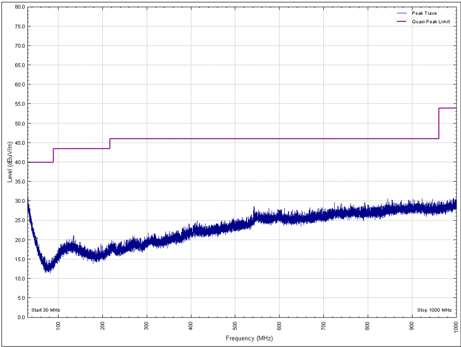
Figure 7 - 2402 MHz, 30 MHz to 1 GHz, Vertical, Z Orientation
