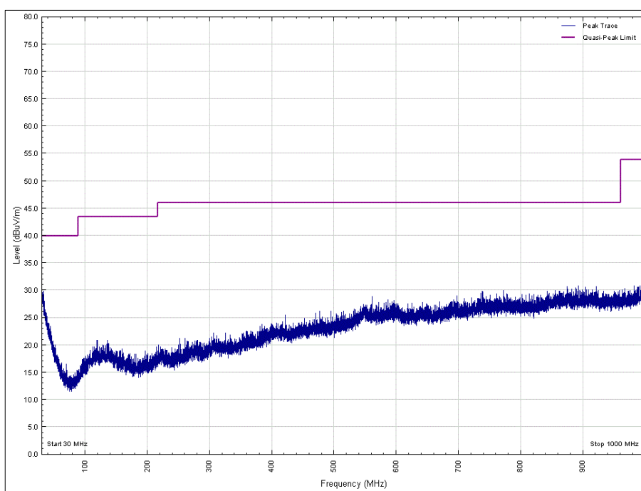
Figure 40 – 2480 MHz, 30 MHz to 1 GHz, Horizontal, X Orientation
