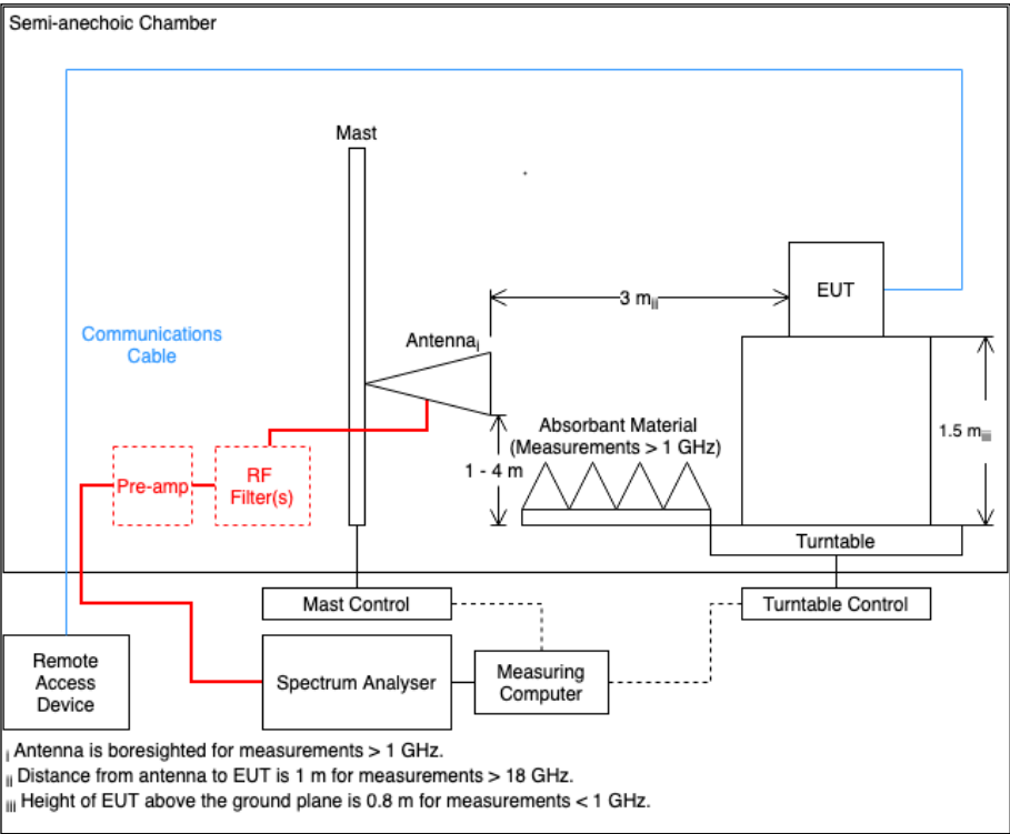
Figure 2 - Test Setup Diagram
