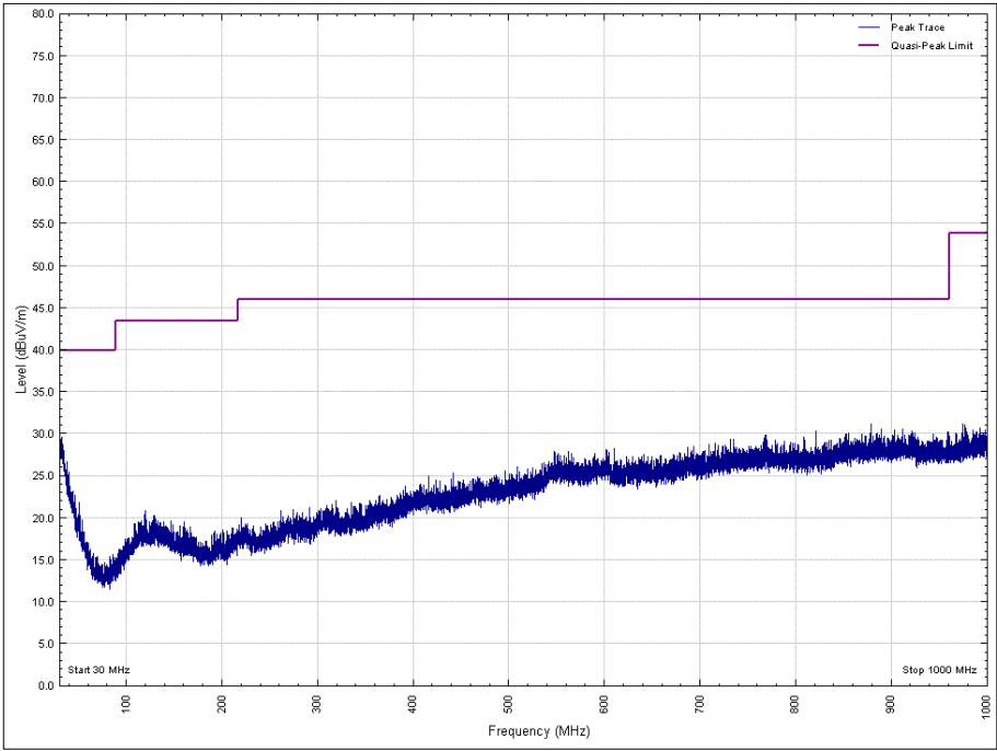
Figure 42 – 2480 MHz, 30 MHz to 1 GHz, Horizontal, Y Orientation
