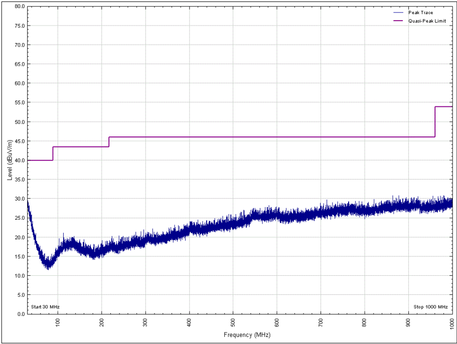
Figure 44 – 2480 MHz, 30 MHz to 1 GHz, Horizontal, Z Orientation
