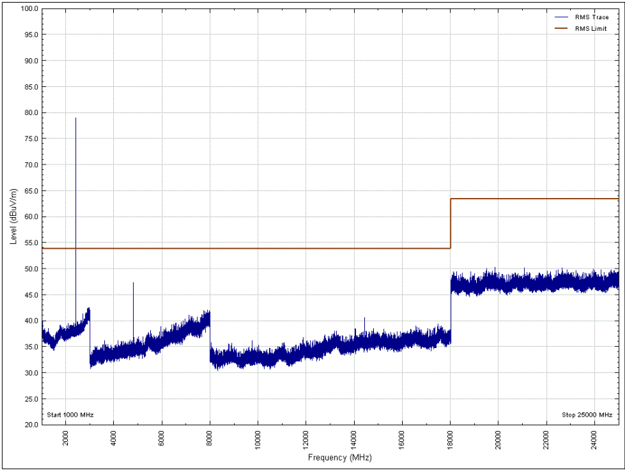
Figure 14 - 2402 MHz , 1 GHz to 25 GHz, Vertical, Y Orientation, Average
