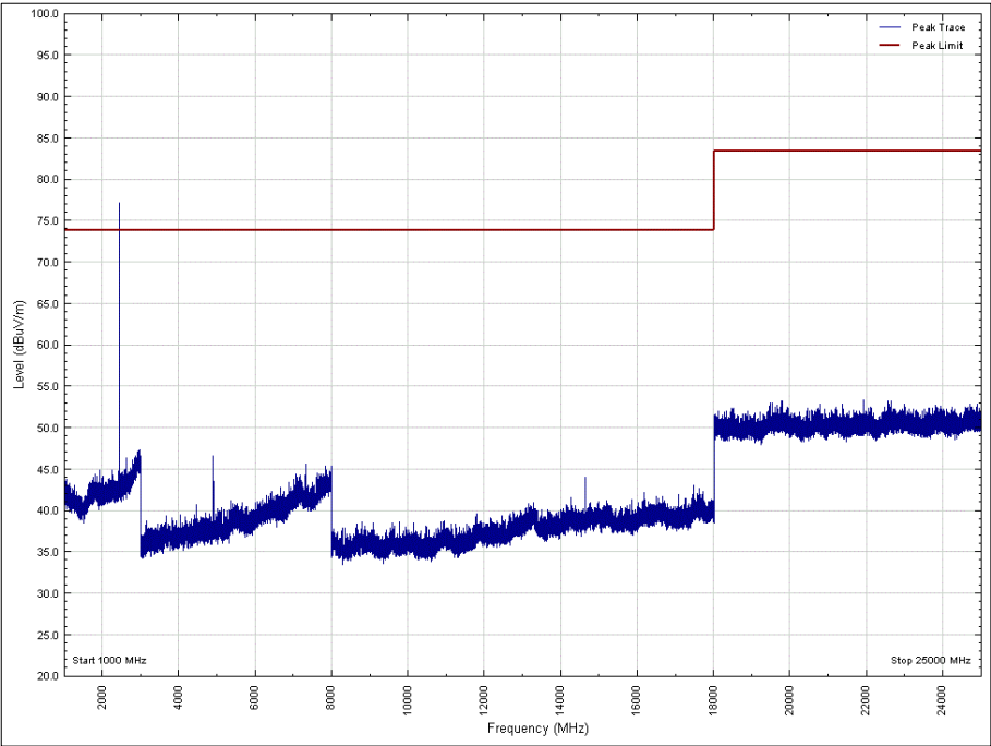
Figure 27 - 2440 MHz, 1 GHz to 25 GHz, Vertical, X Orientation, Peak
