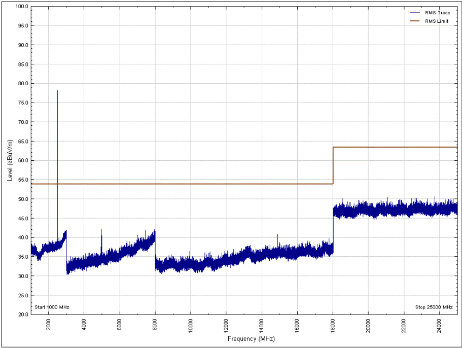
Figure 52 - 2480 MHz, 1 GHz to 25 GHz, Horizontal, Y Orientation, Average
