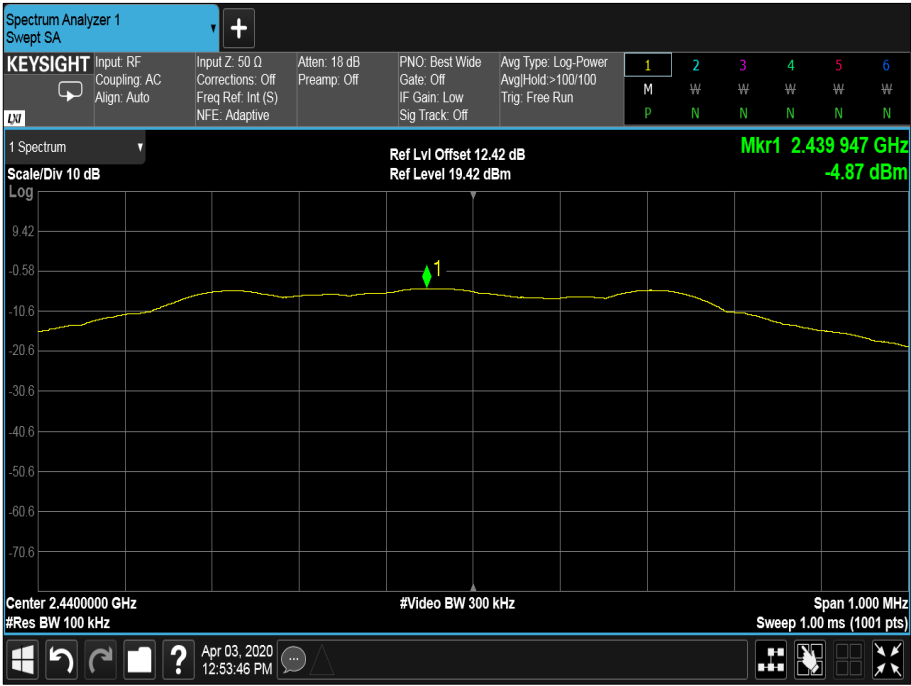
Figure 69 - 2440 MHz
