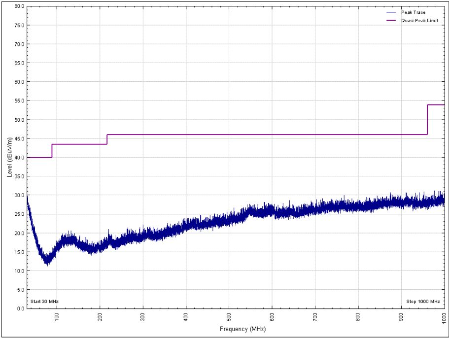
Figure 6 - 2402 MHz, 30 MHz to 1 GHz, Horizontal, Y Orientation
