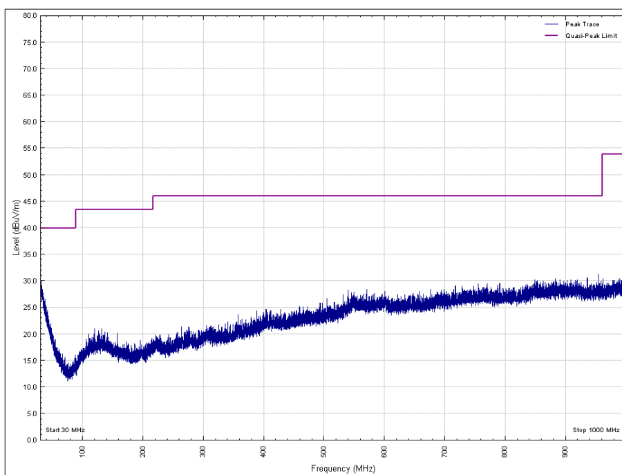
Figure 21 - 2440 MHz, 30 MHz to 1 GHz, Vertical, X Orientation
