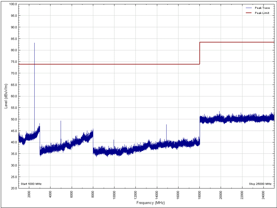
Figure 53 - 2480 MHz, 1 GHz to 25 GHz, Vertical, Z Orientation, Peak
