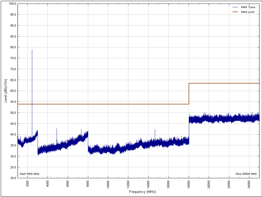
Figure 34 - 2440 MHz, 1 GHz to 25 GHz, Horizontal, Y Orientation, Average
