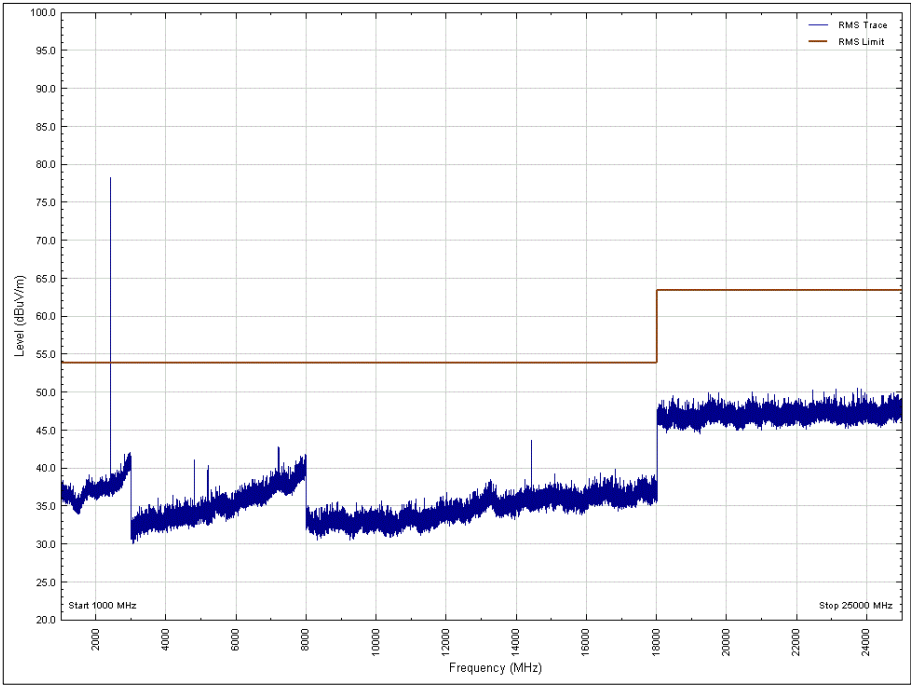
Figure 20 - 2402 MHz , 1 GHz to 25 GHz, Horizontal, Z Orientation, Average
