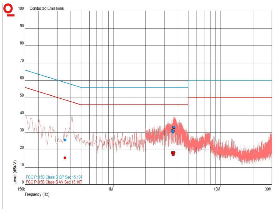
Figure 63 - Neutral Line - 150 kHz to 30 MHz
