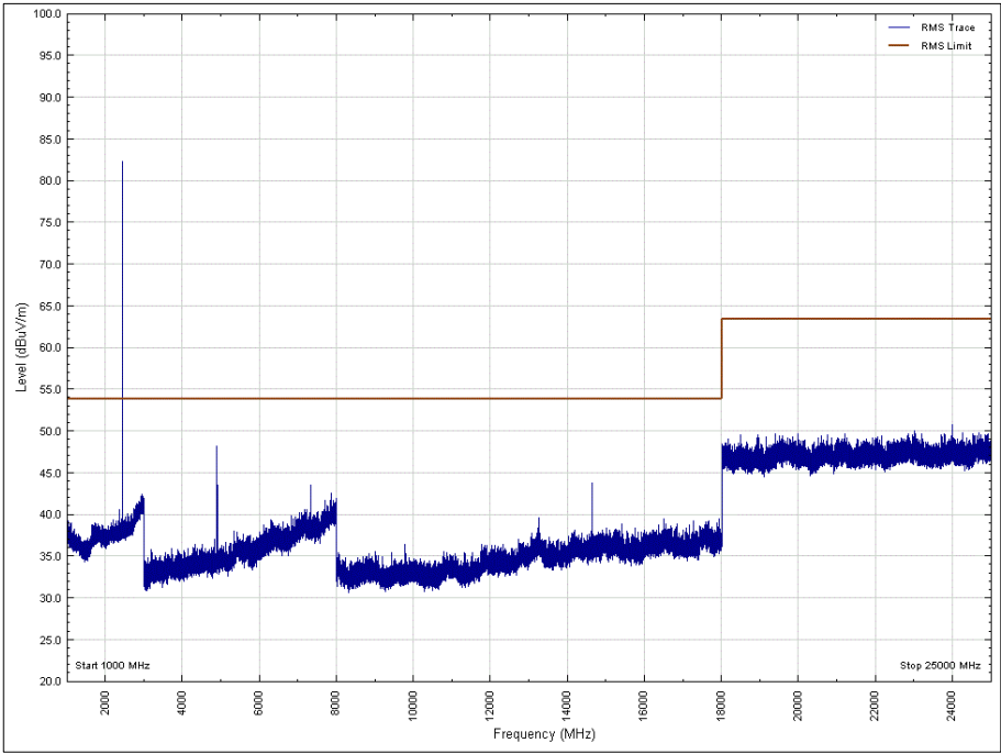
Figure 36 - 2440 MHz, 1 GHz to 25 GHz, Vertical, Z Orientation, Average
