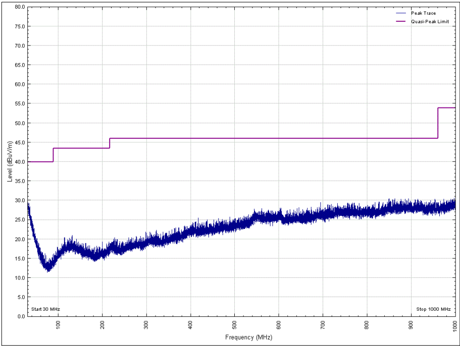
Figure 41 – 2480 MHz, 30 MHz to 1 GHz, Vertical, Y Orientation
