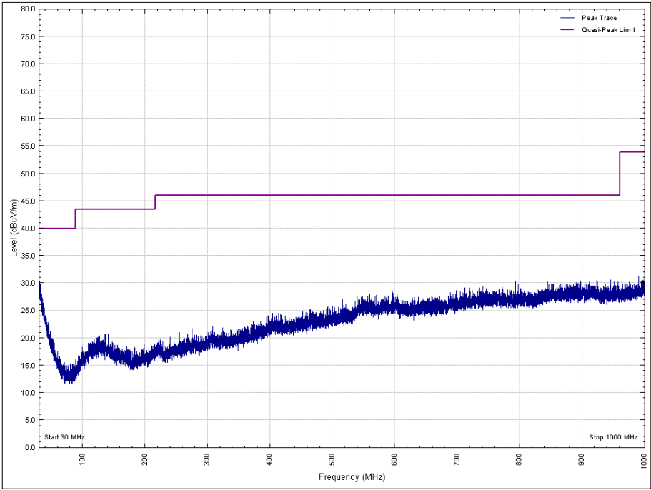
Figure 8 - 2402 MHz, 30 MHz to 1 GHz, Horizontal, Z Orientation
