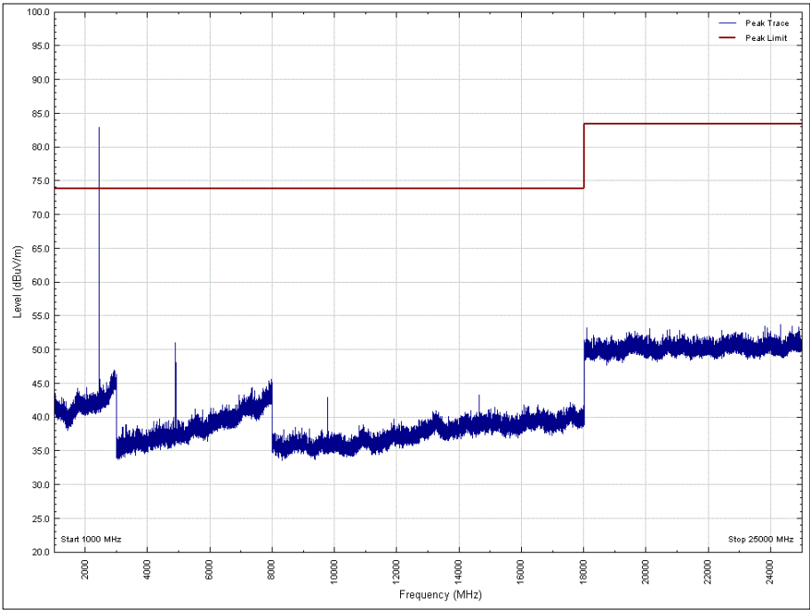
Figure 29 - 2440 MHz, 1 GHz to 25 GHz, Horizontal, X Orientation, Peak
