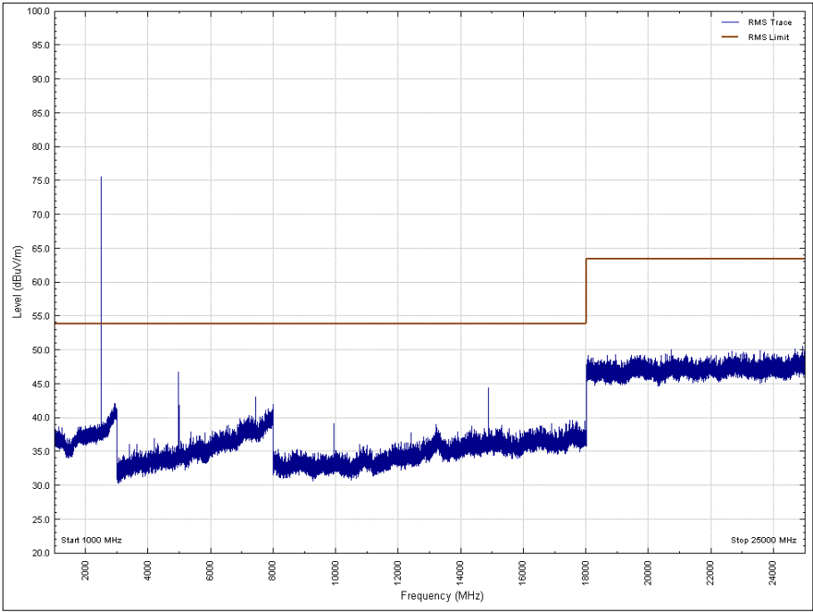
Figure 56 - 2480 MHz, 1 GHz to 25 GHz, Horizontal, Z Orientation, Average
