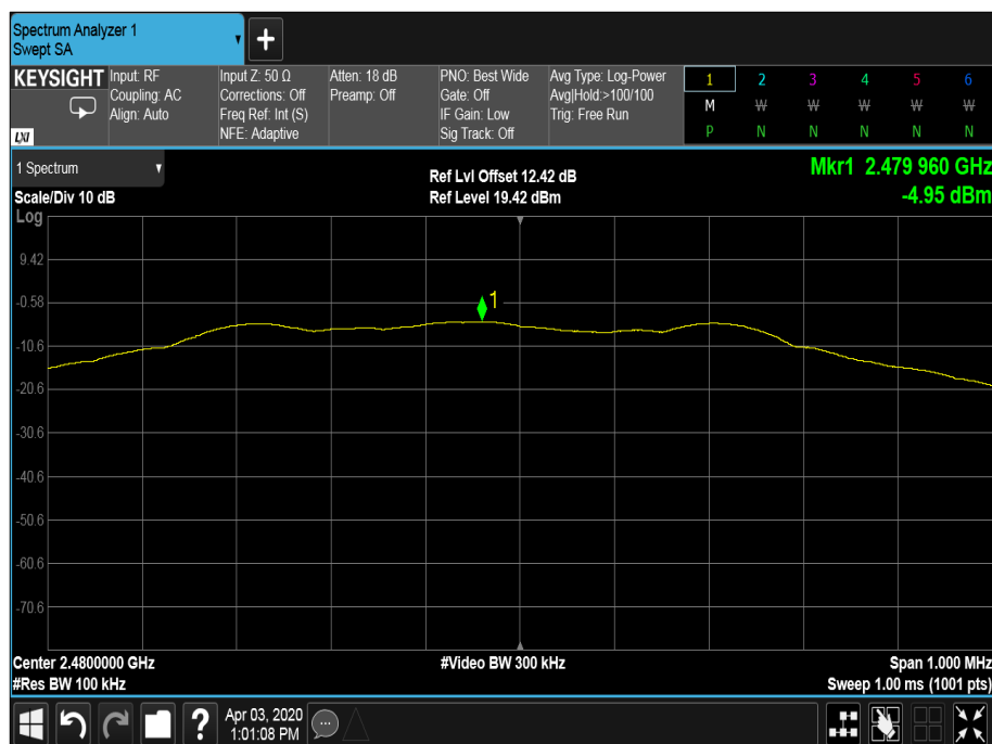
Figure 70 - 2480 MHz
