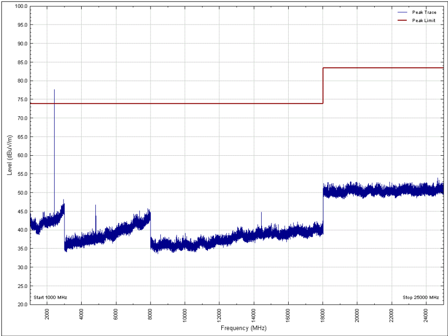
Figure 9 - 2402 MHz, 1 GHz to 25 GHz, Vertical, X Orientation, Peak
