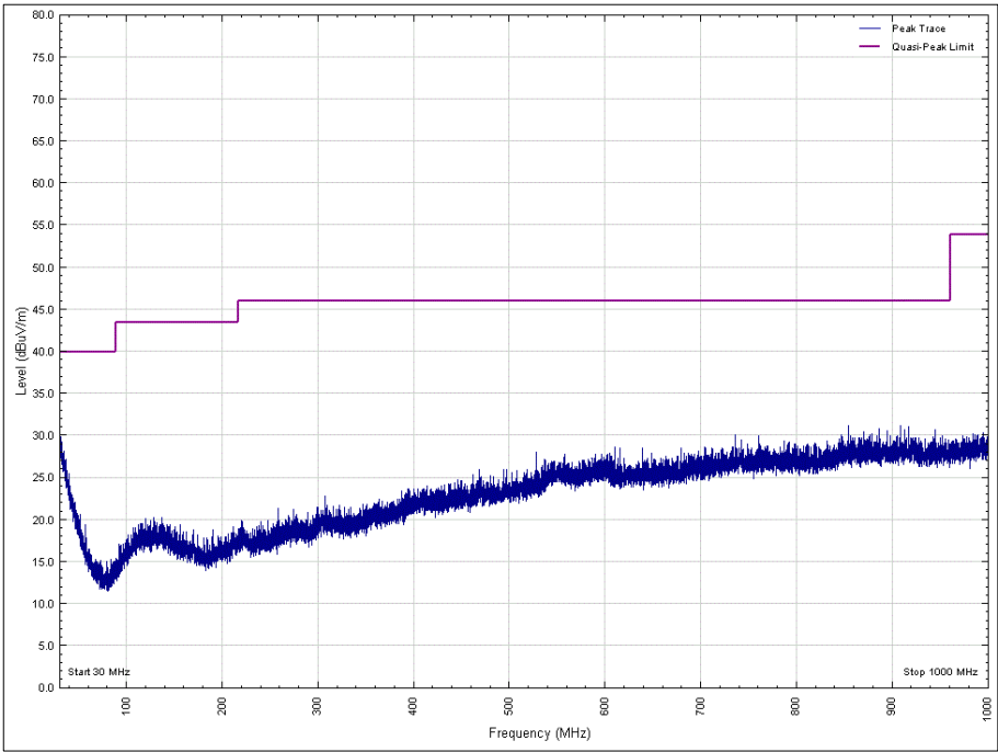
Figure 3 - 2402 MHz, 30 MHz to 1 GHz, Vertical, X Orientation
