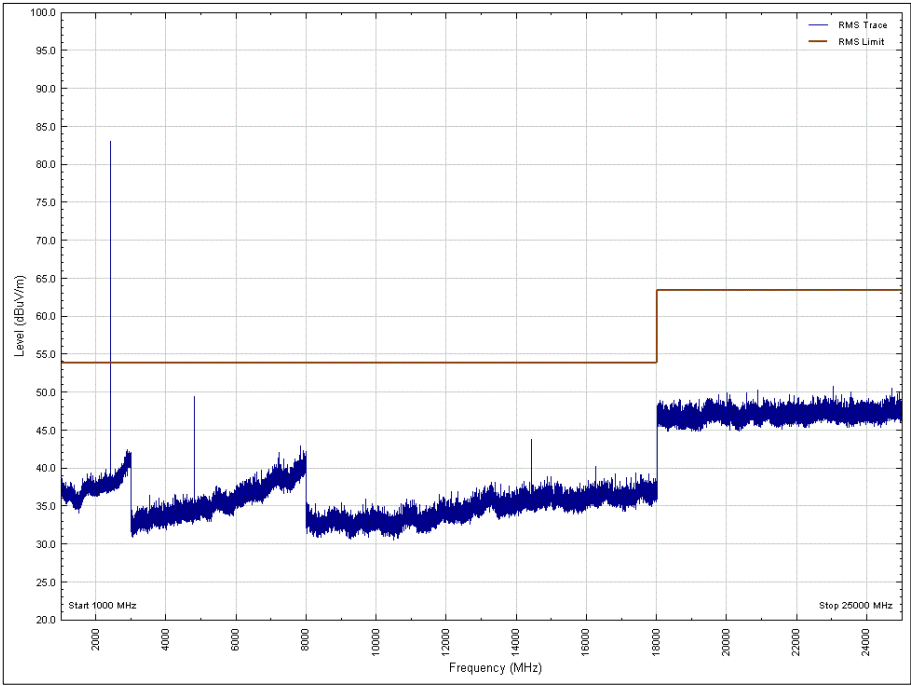
Figure 18 - 2402 MHz , 1 GHz to 25 GHz, Vertical, Z Orientation, Average
