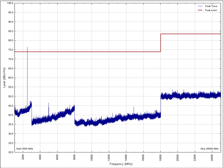
Figure 45 - 2480 MHz, 1 GHz to 25 GHz, Vertical, X Orientation, Peak
