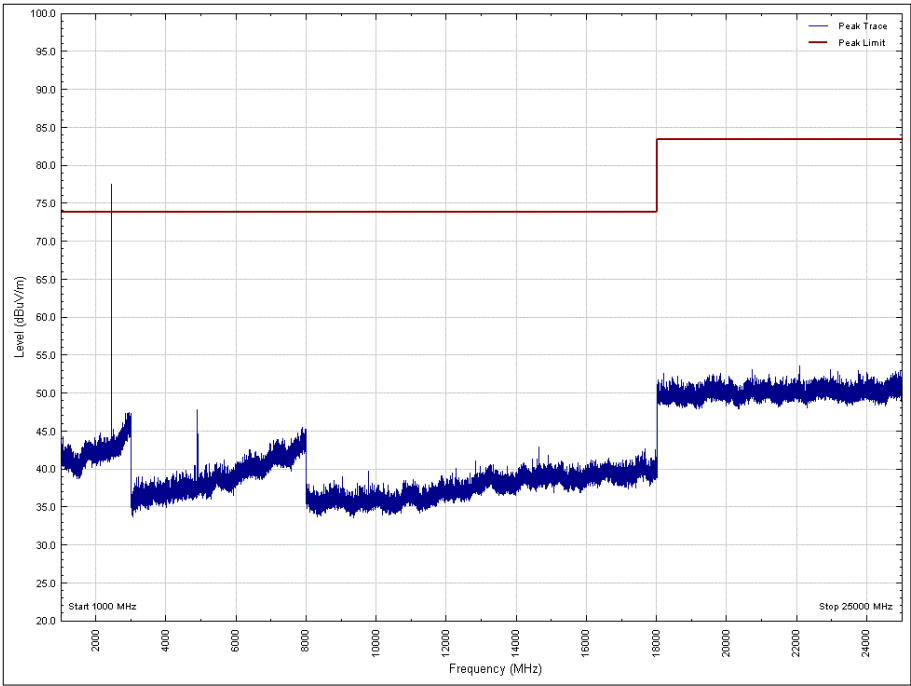
Figure 31 - 2440 MHz, 1 GHz to 25 GHz, Vertical, Y Orientation, Peak
