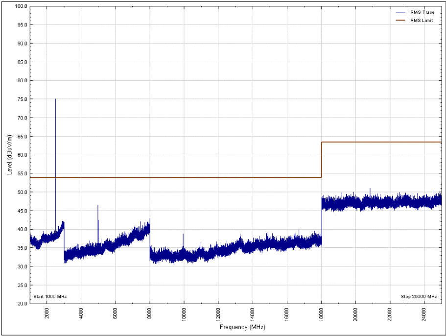
Figure 50 - 2480 MHz, 1 GHz to 25 GHz, Vertical, Y Orientation, Average
