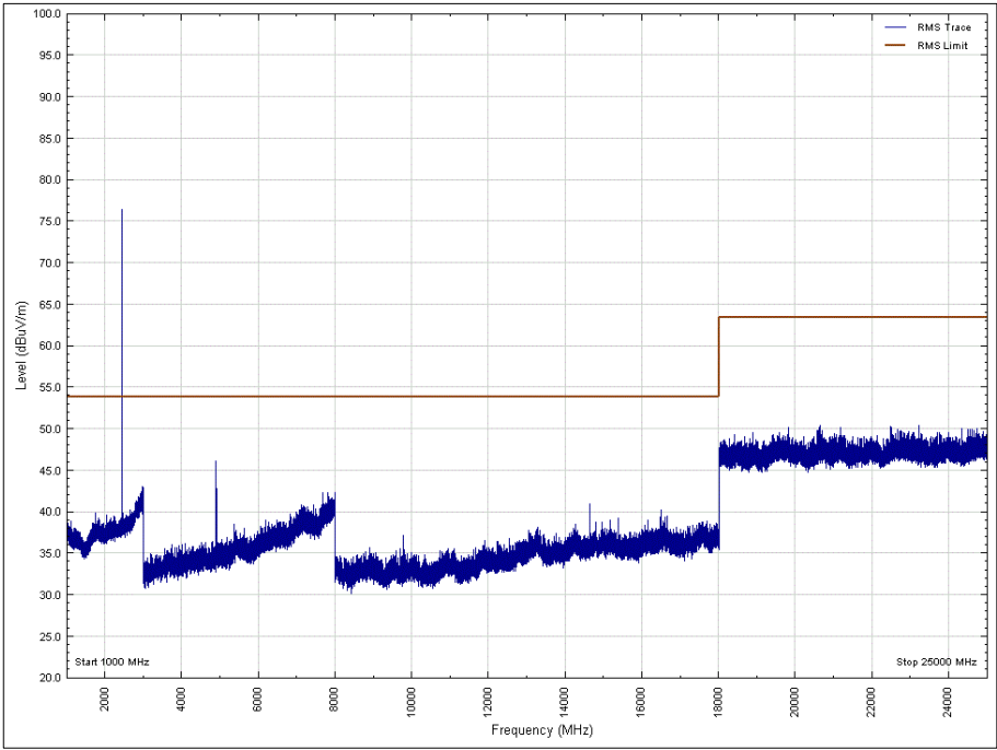
Figure 32 - 2440 MHz, 1 GHz to 25 GHz, Vertical, Y Orientation, Average
