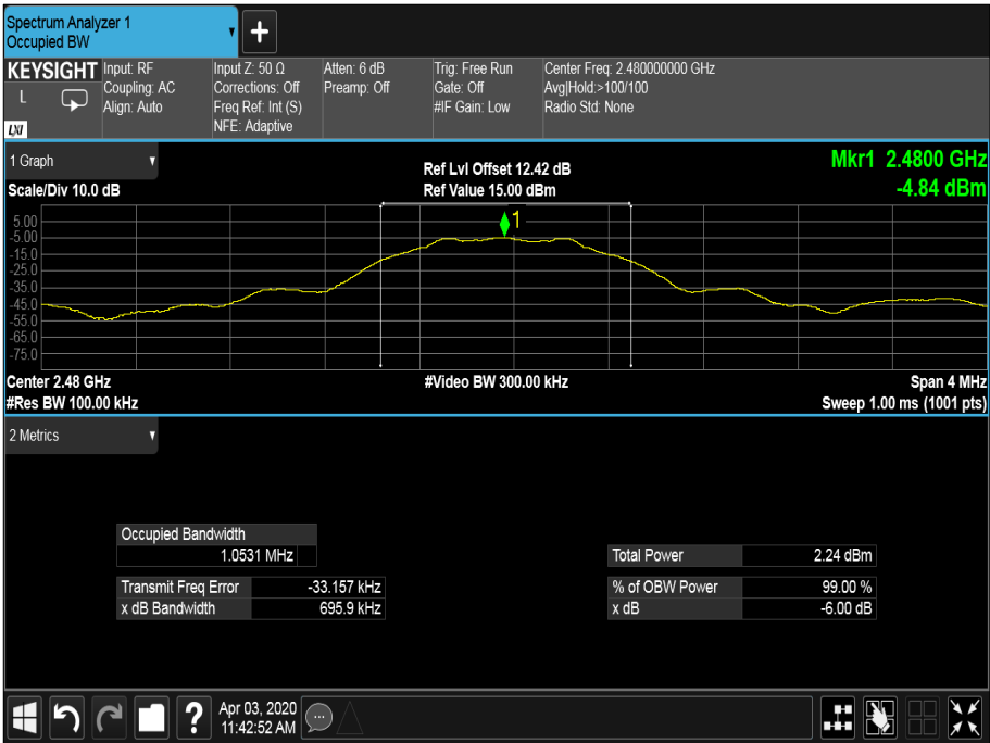
Figure 67 - 2480 MHz – 6 dB and 99% Occupied Bandwidth
