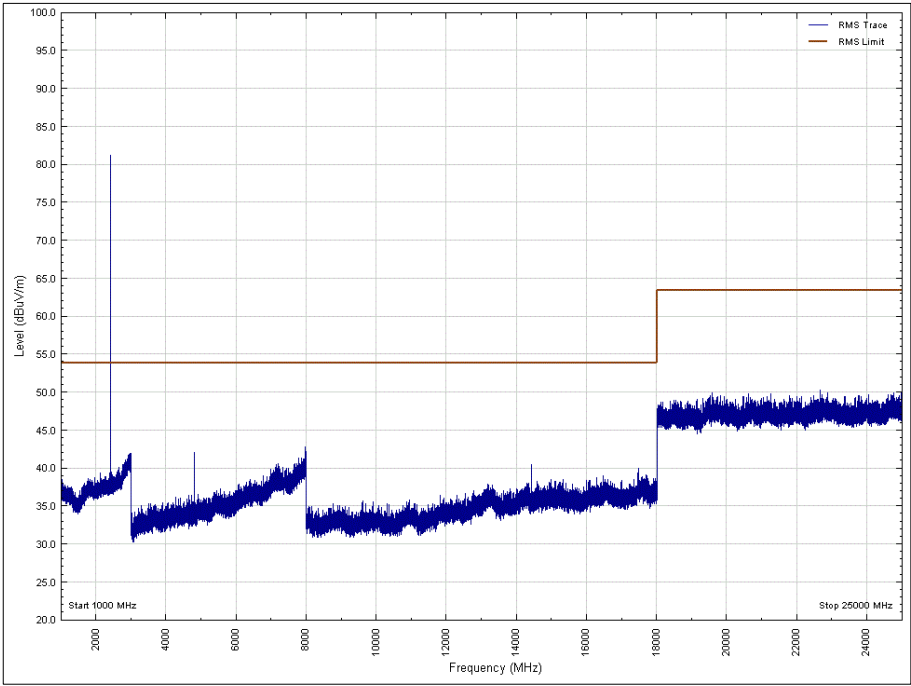
Figure 16 - 2402 MHz , 1 GHz to 25 GHz, Horizontal, Y Orientation, Average
