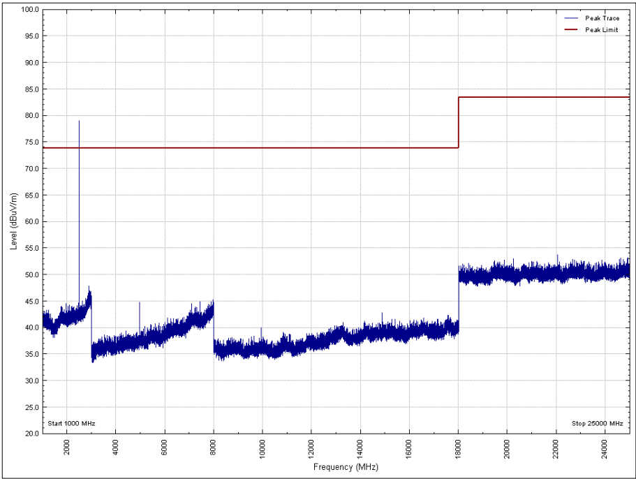
Figure 51 - 2480 MHz, 1 GHz to 25 GHz, Horizontal, Y Orientation, Peak
