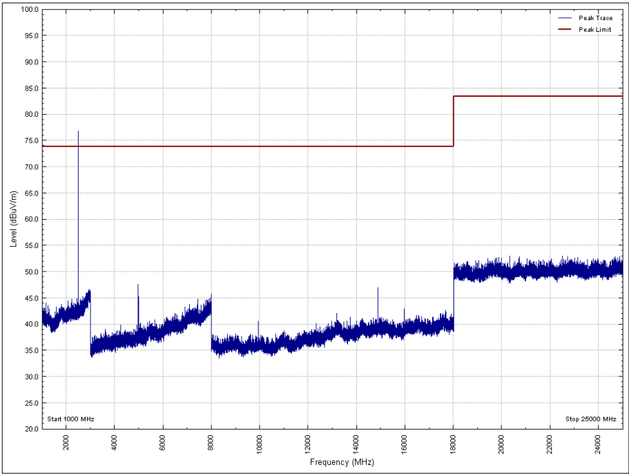
Figure 55 - 2480 MHz, 1 GHz to 25 GHz, Horizontal, Z Orientation, Peak
