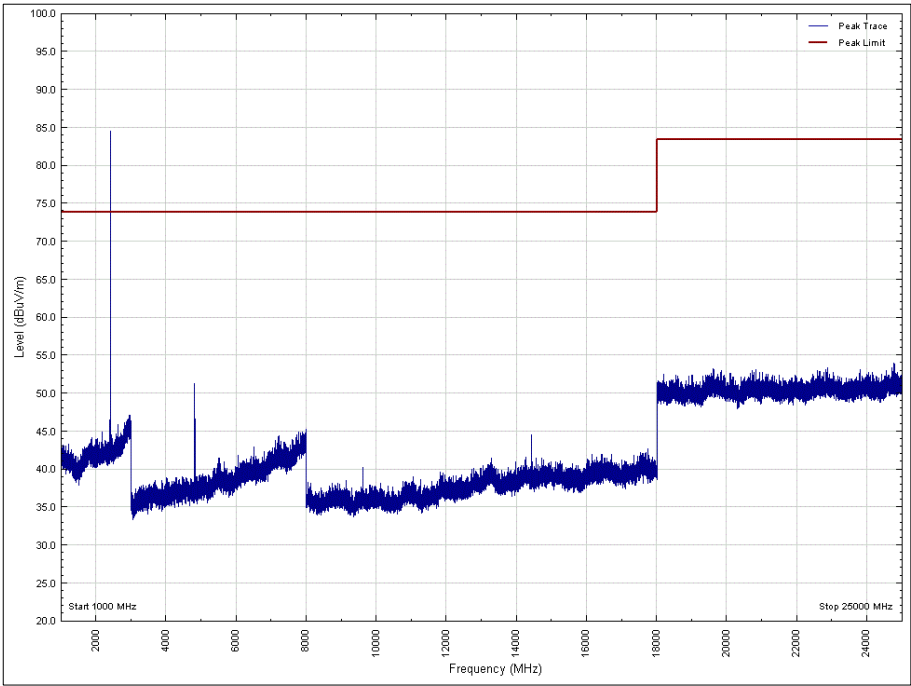
Figure 11 - 2402 MHz , 1 GHz to 25 GHz, Horizontal, X Orientation, Peak
