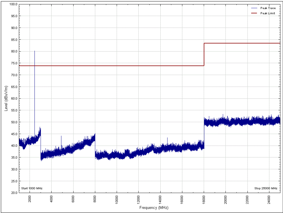
Figure 33 - 2440 MHz, 1 GHz to 25 GHz, Horizontal, Y Orientation, Peak
