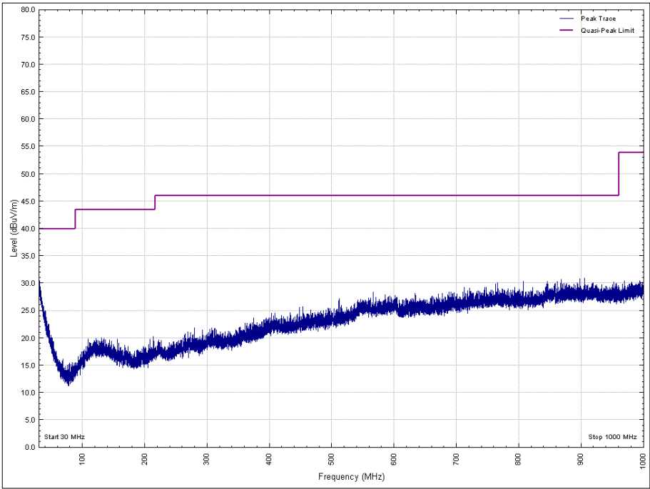
Figure 5 - 2402 MHz, 30 MHz to 1 GHz, Vertical, Y Orientation
