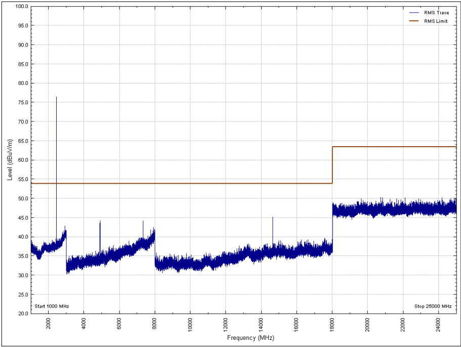
Figure 38 - 2440 MHz, 1 GHz to 25 GHz, Horizontal, Z Orientation, Average
