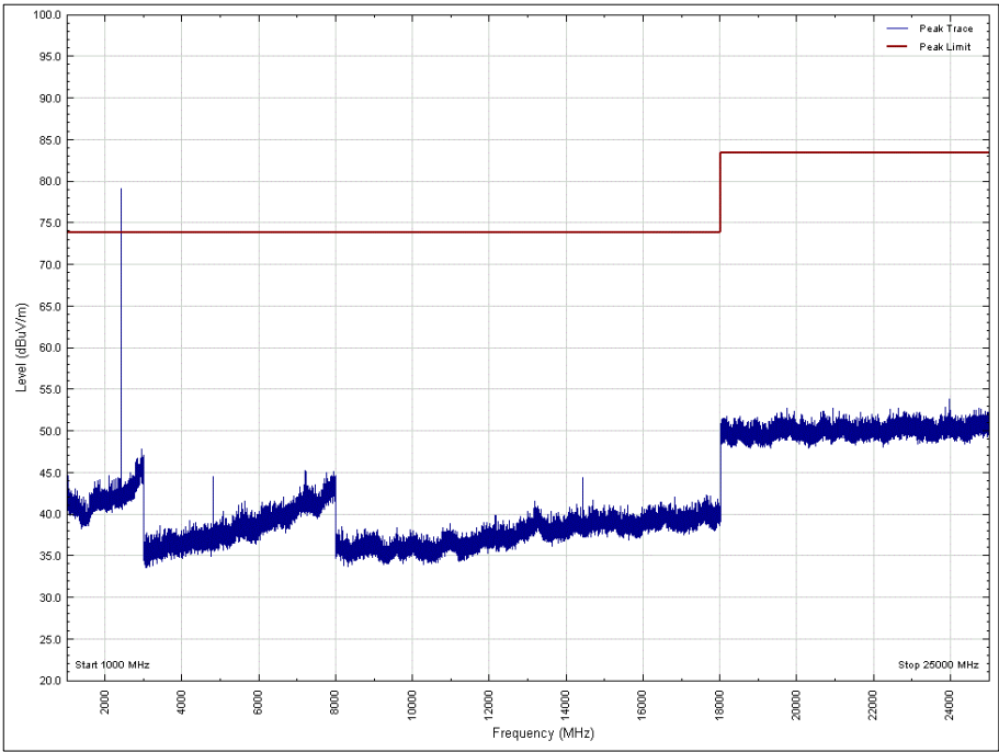
Figure 19 - 2402 MHz , 1 GHz to 25 GHz, Horizontal, Z Orientation, Peak
