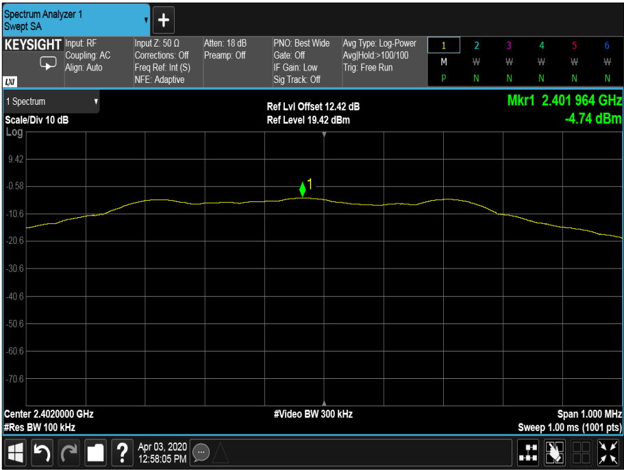
Figure 68 - 2402 MHz
