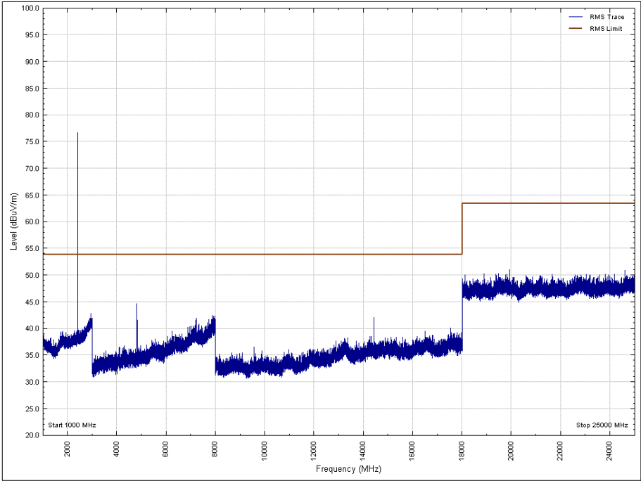
Figure 10 - 2402 MHz, 1 GHz to 25 GHz, Vertical, X Orientation, Average
