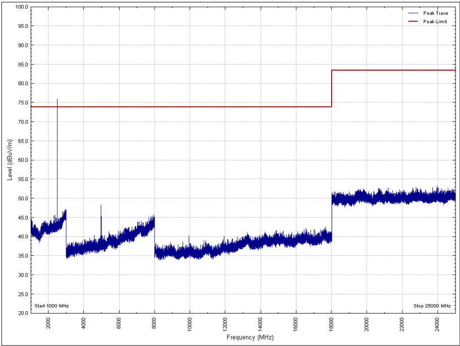
Figure 49 - 2480 MHz, 1 GHz to 25 GHz, Vertical, Y Orientation, Peak
