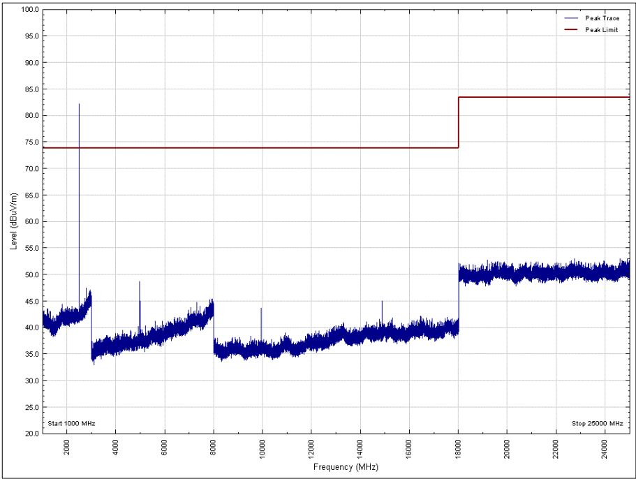
Figure 47 - 2480 MHz, 1 GHz to 25 GHz, Horizontal, X Orientation, Peak
