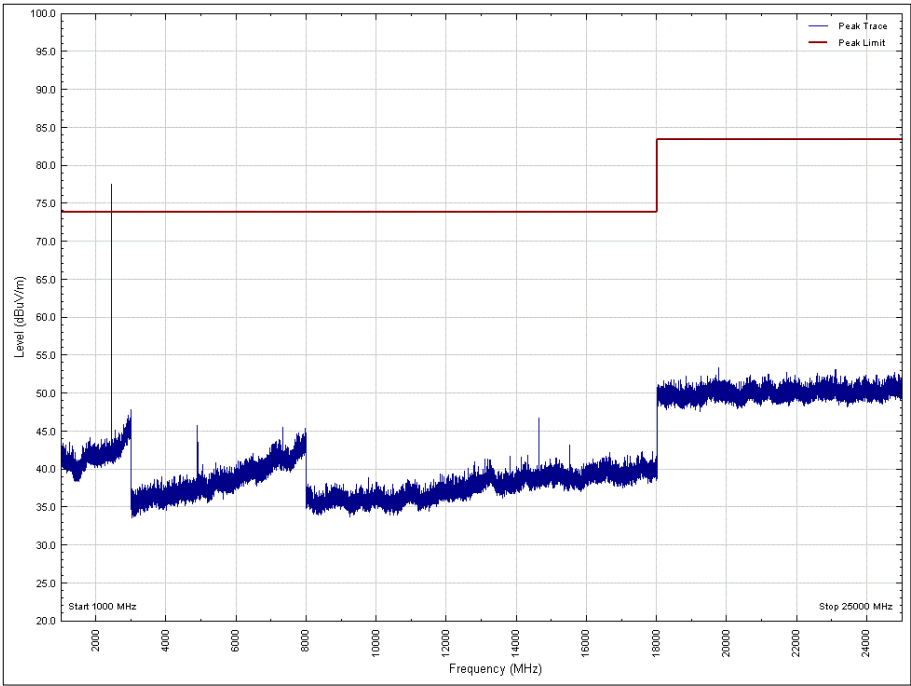
Figure 37 - 2440 MHz, 1 GHz to 25 GHz, Horizontal, Z Orientation, Peak
