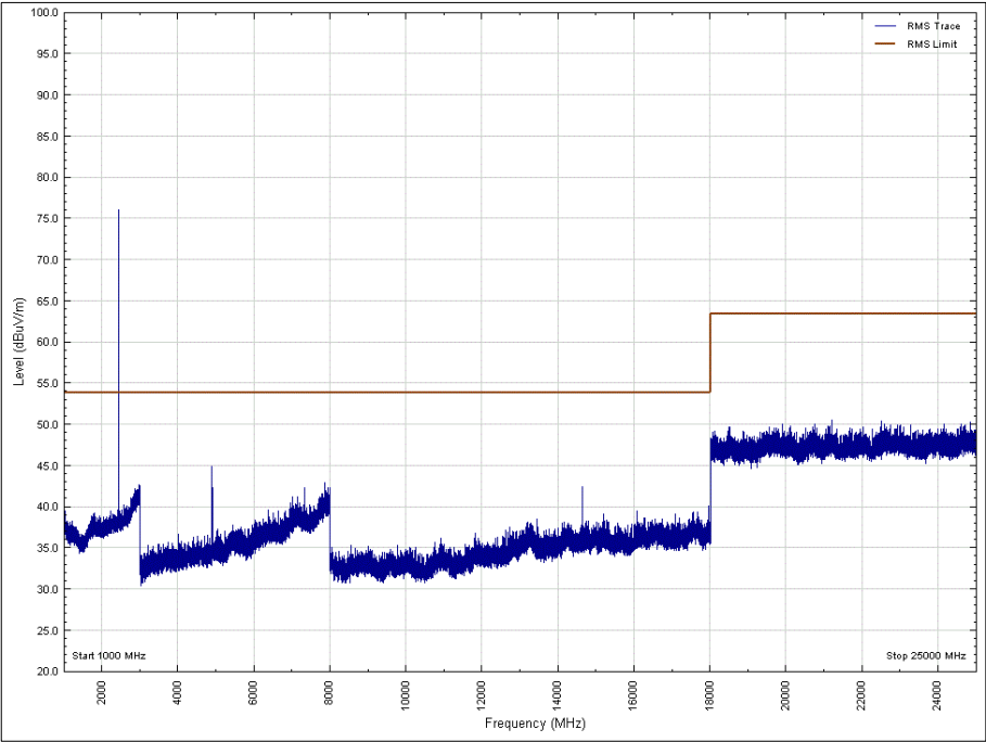
Figure 28 - 2440 MHz, 1 GHz to 25 GHz, Vertical, X Orientation, Average
