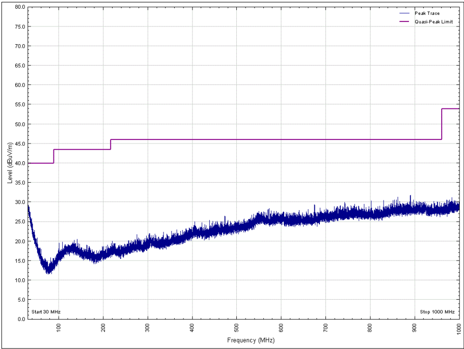
Figure 25 - 2440 MHz, 30 MHz to 1 GHz, Vertical, Z Orientation
