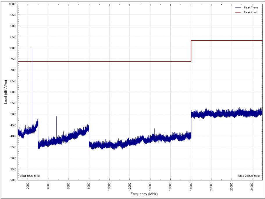
Figure 13 - 2402 MHz , 1 GHz to 25 GHz, Vertical, Y Orientation, Peak
