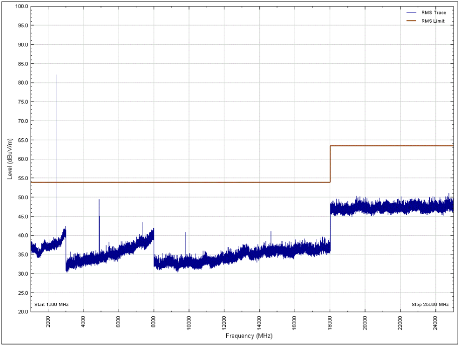
Figure 30 - 2440 MHz, 1 GHz to 25 GHz, Horizontal, X Orientation, Average
