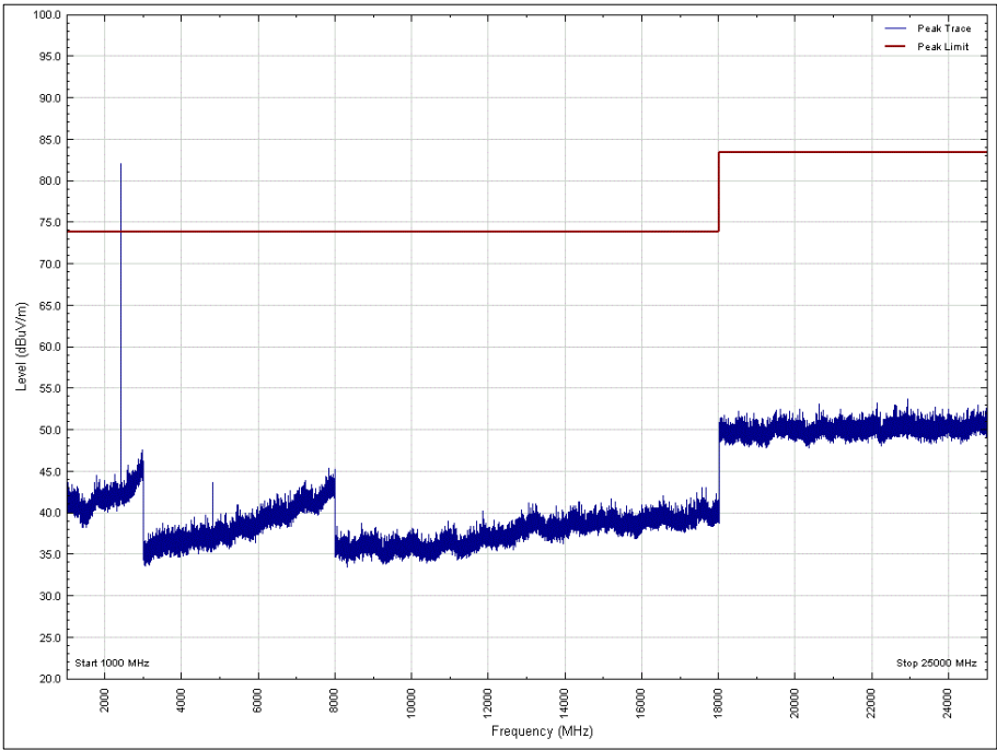
Figure 15 - 2402 MHz , 1 GHz to 25 GHz, Horizontal, Y Orientation, Peak
