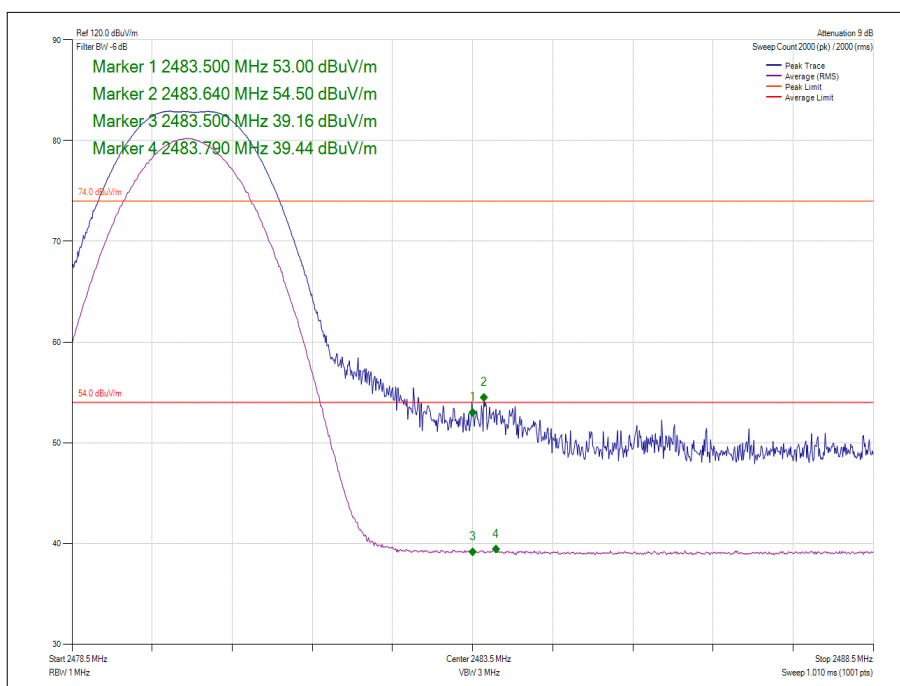
Figure 62 - GFSK - 2480 MHz - Measured Frequency 2483.5 MHz
