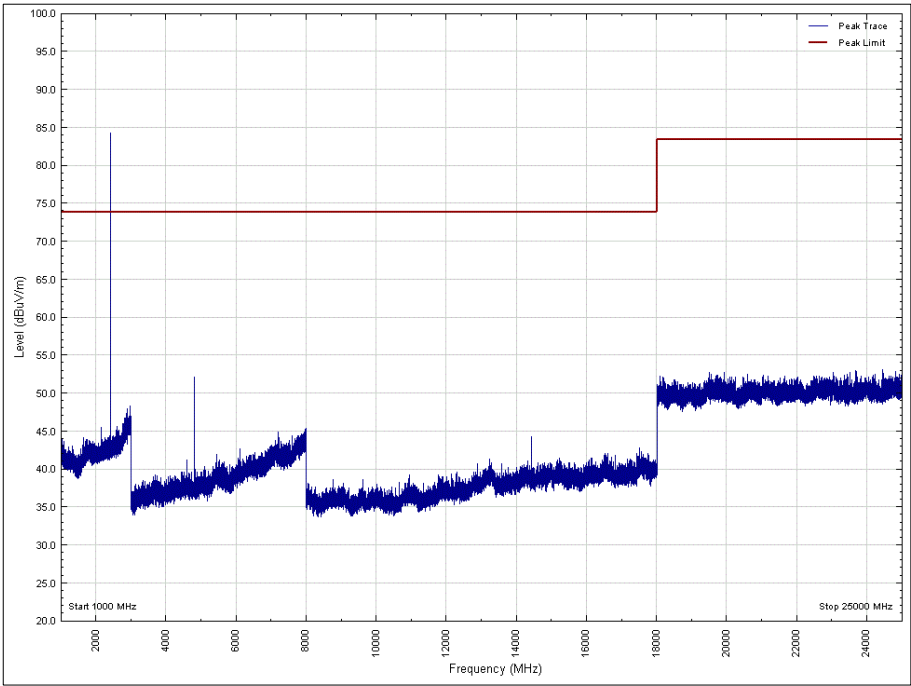
Figure 17 - 2402 MHz , 1 GHz to 25 GHz, Vertical, Z Orientation, Peak
