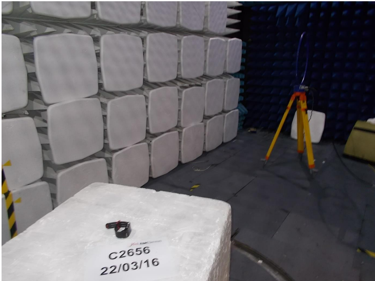
Chamber measurement 9kHz to 30MHz
