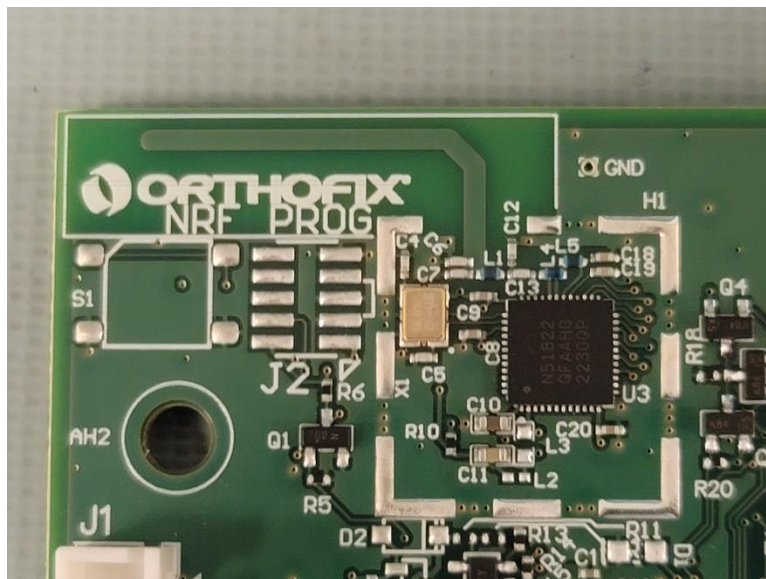
Figure 48 - 5314RCM PCA, Radio and Antenna
