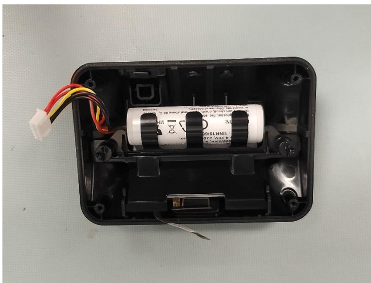
Figure 4 - 5212CM Control Module, PCA Removed
