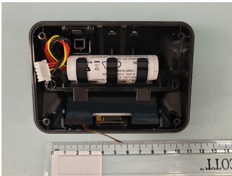
Figure 21 - 5302CM Control Module, All Components Removed
