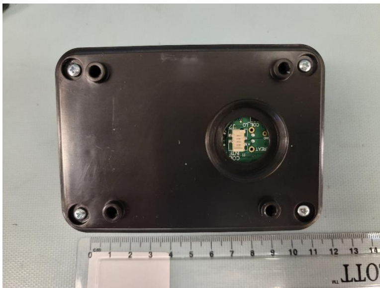
Figure 42 - 5314RCM Control Module, Rear
