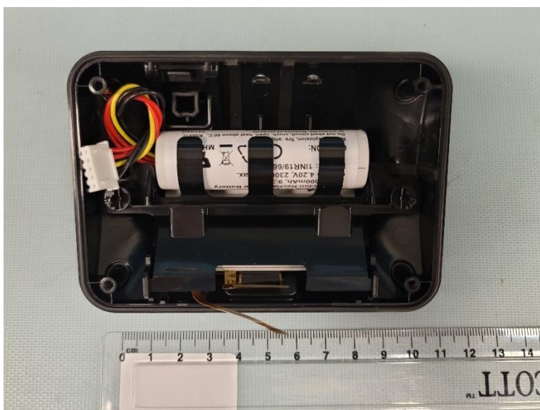
Figure 20 - 5302CM Control Module, PCA Removed
