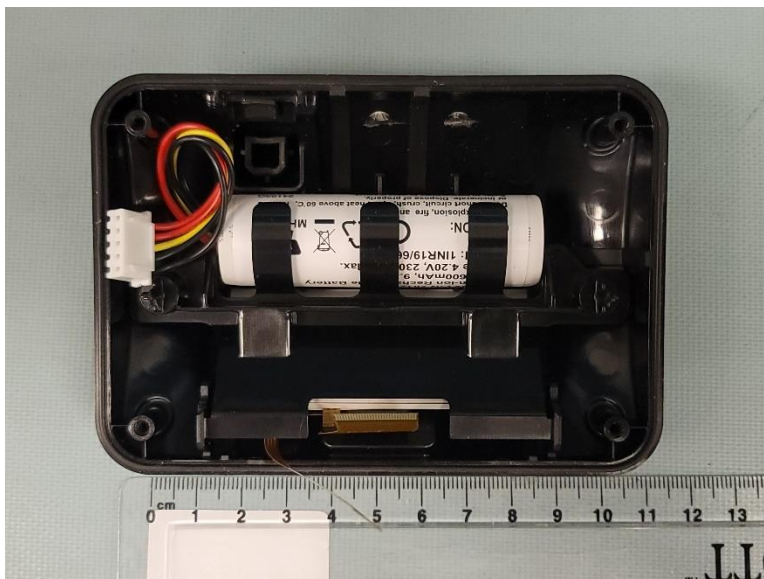
Figure 12 - 5505CM Control Module, PCA Removed
