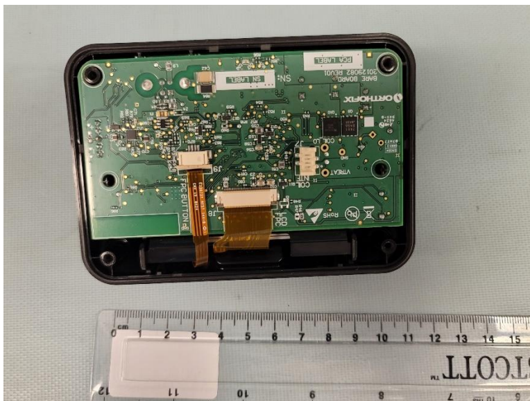
Figure 19 - 5302CM Control Module, Cover Removed
