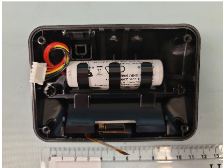
Figure 60 - 5315CM Control Module, PCA Removed
