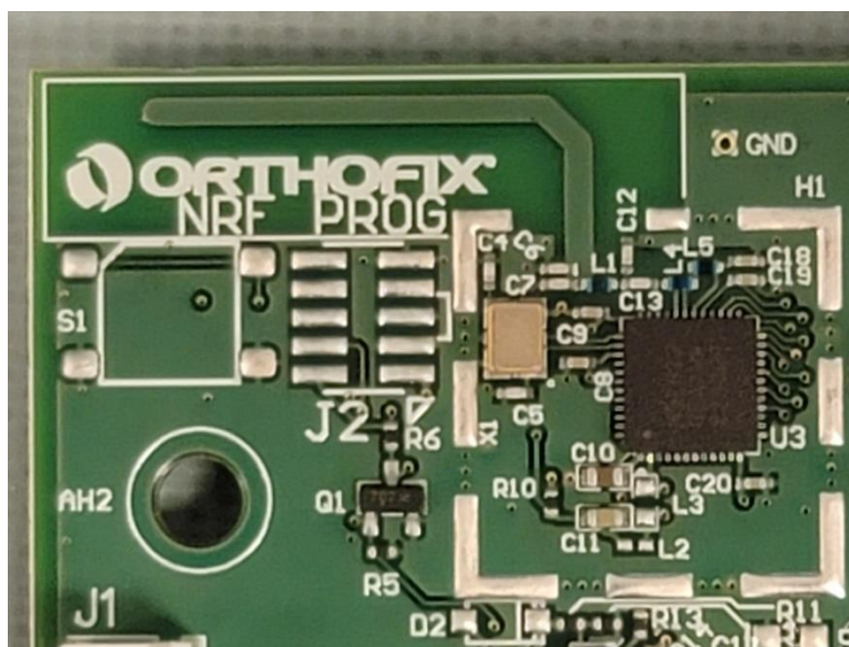
Figure 8 - 5212CM PCA, Radio and Antenna
