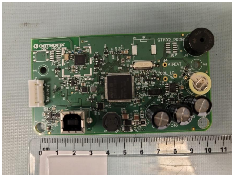
Figure 62 - 5315CM PCA Top
