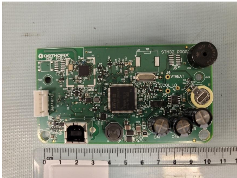
Figure 46 - 5314RCM PCA Top
