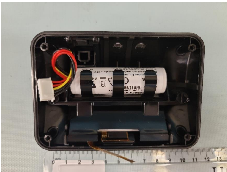
Figure 36 - 5313CM Control Module, PCA Removed
