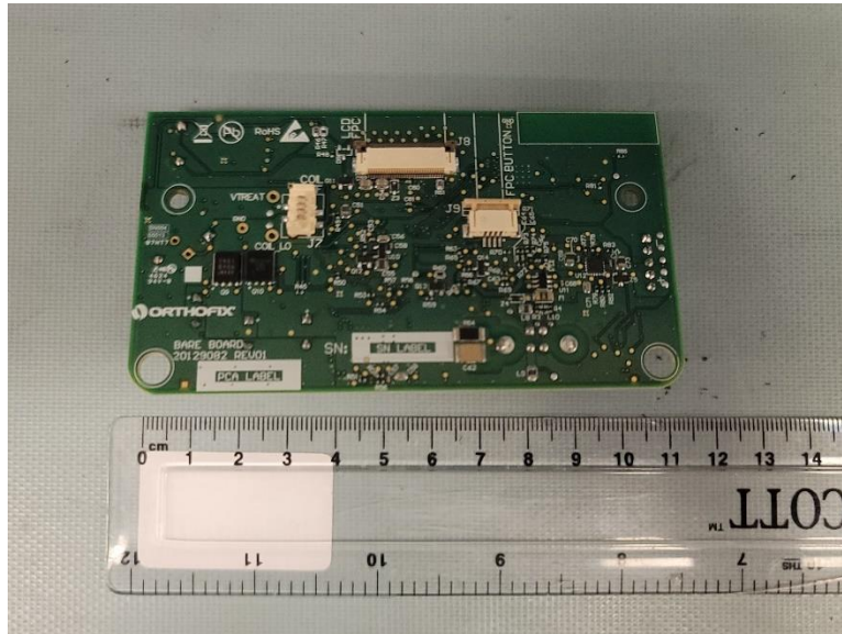
Figure 23 - 5302CM PCA Bottom
