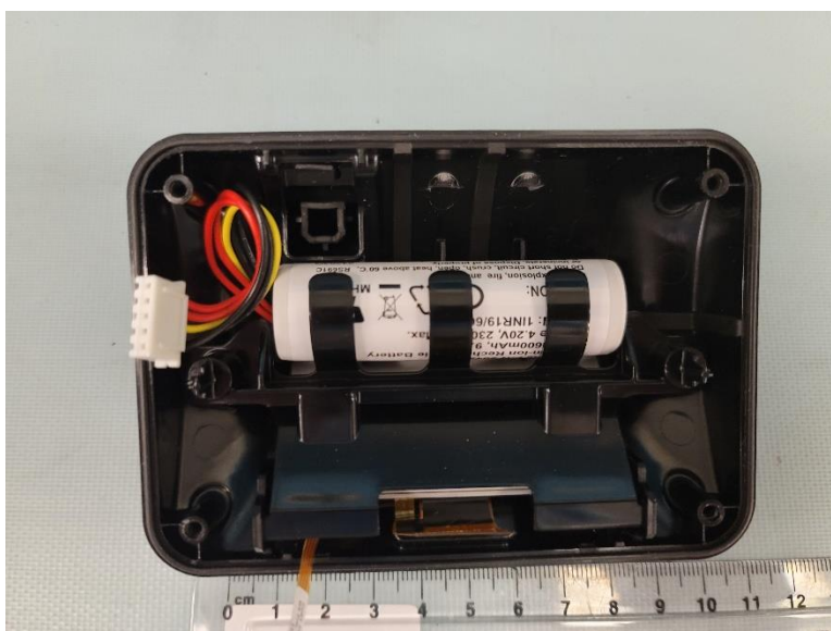
Figure 52 - 5314LCM Control Module, PCA Removed
