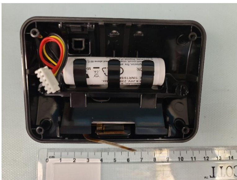
Figure 44 - 5314RCM Control Module, PCA Removed
