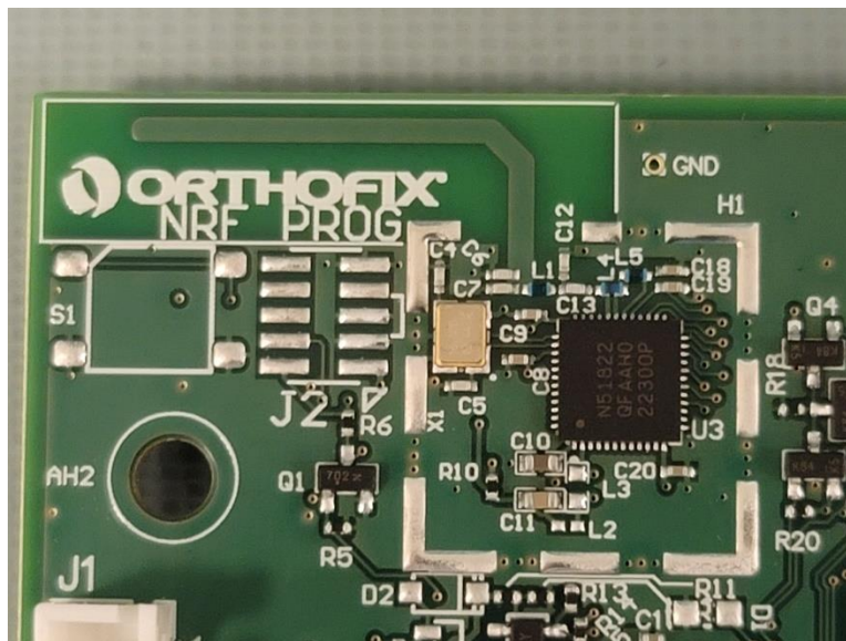
Figure 40 - 5313CM PCA, Radio and Antenna
