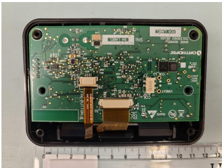
Figure 43 - 5314RCM Control Module, Cover Removed
