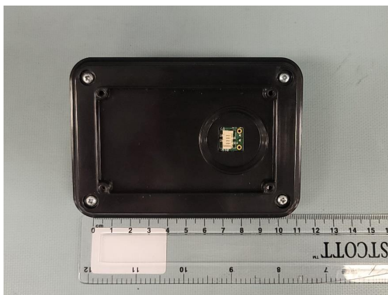
Figure 10 - 5505CM Control Module, Rear
