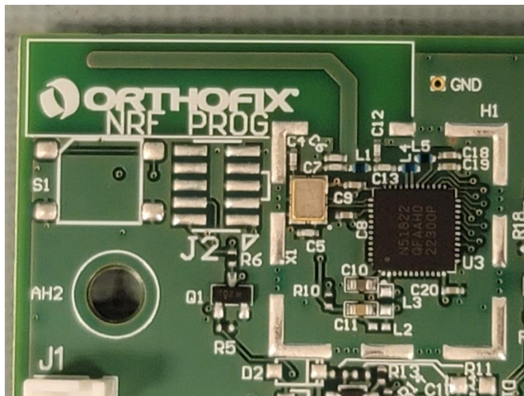
Figure 24 - 5302CM PCA, Radio and Antenna
