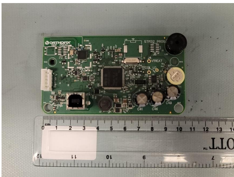
Figure 22 - 5302CM PCA Top
