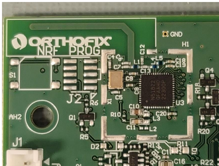
Figure 16 - 5505CM PCA, Radio and Antenna
