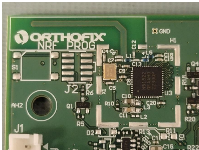
Figure 56 - 5314LCM PCA, Radio and Antenna
