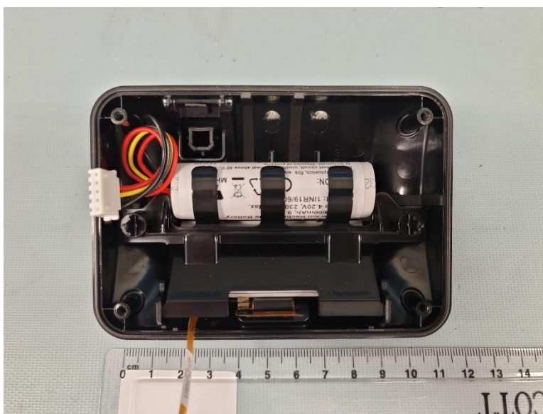
Figure 28 - 5303CM Control Module, PCA Removed
