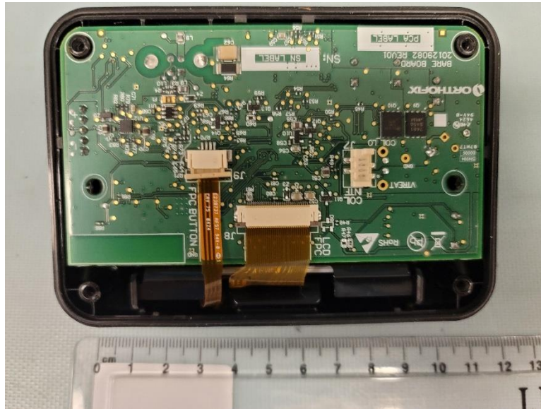
Figure 59 - 5315CM Control Module, Cover Removed
