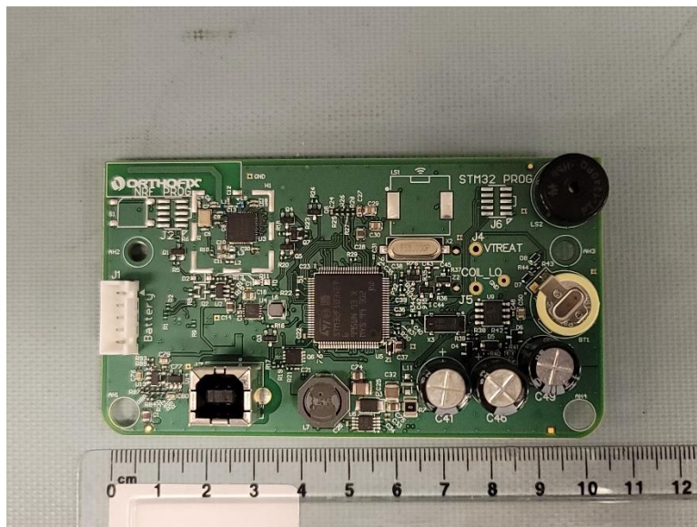
Figure 14 - 5505CM PCA Top
