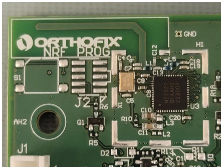
Figure 64 - 5315CM PCA, Radio and Antenna
