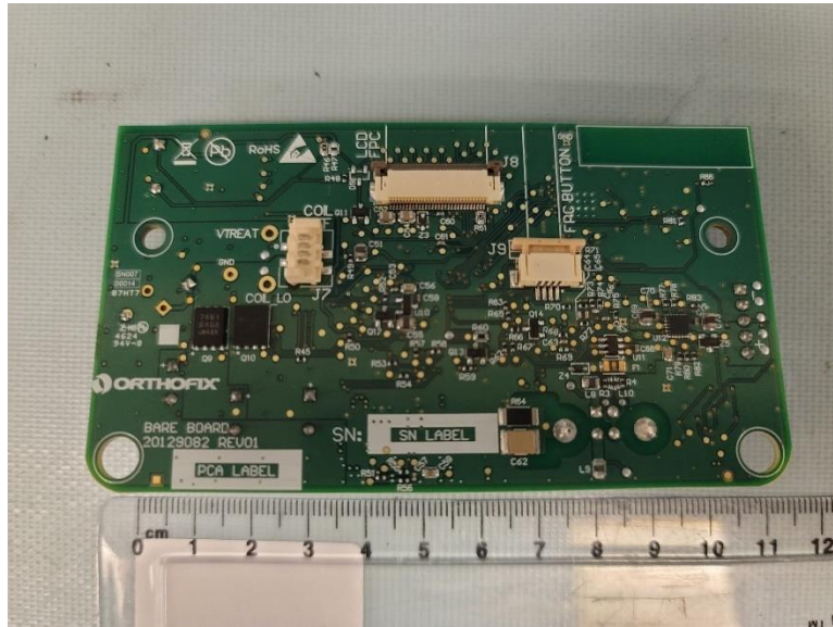
Figure 47 - 5314RCM PCA Bottom
