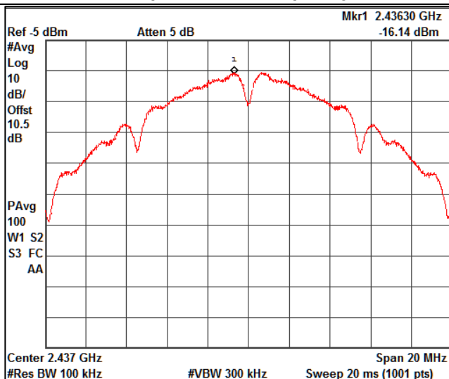
Data Rate: 2Mbps Channel Frequency: 2437MHz
