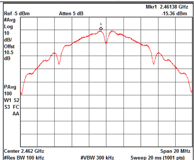
Data Rate: 2Mbps Channel Frequency: 2462MHz
