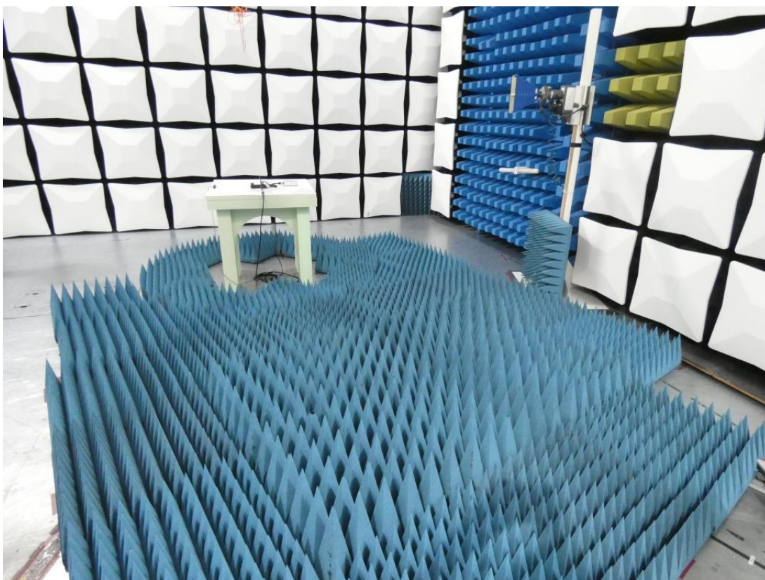
Photo 3: Test setup for radiated measurements (Enclosure, w/ absorber, 1-6 GHz intentional radiator §15)
