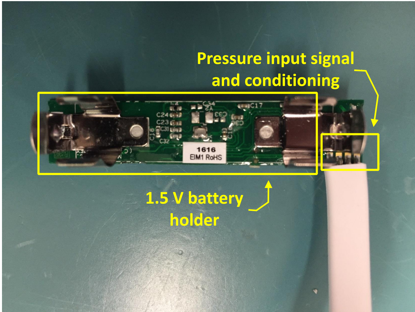
CMSW Pressure Module – Top View
