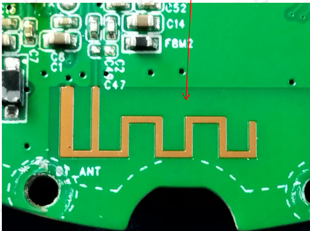
Bluetooth antenna
