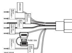
Wiring Harness
