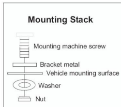
Regular Mounting
