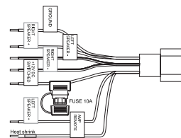
Wiring Harness
