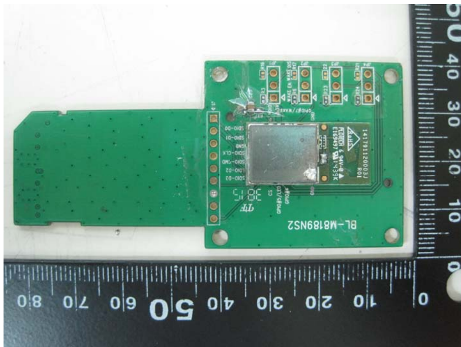
Top View of the test fixture with EUT attached
