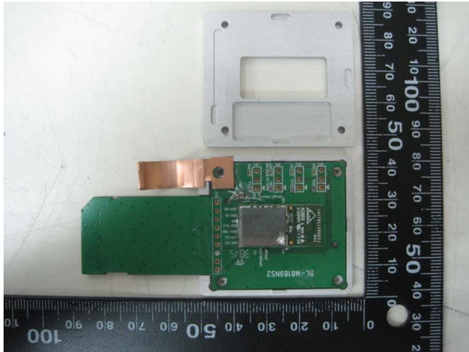
Top View of the EUT on the test fixture (without metal cover & Clip)
