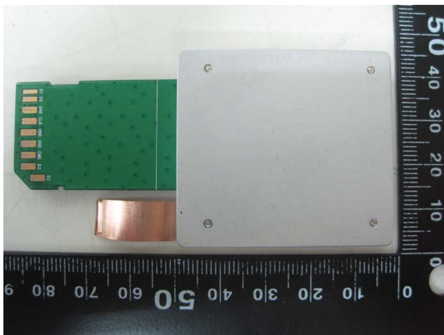
Top View of the EUT on the test fixture (with metal cover & Clip)
