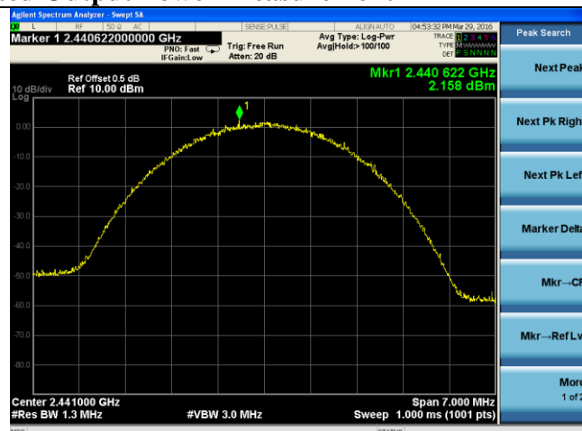
Test frequency: 2441MHz(3Mbps)
