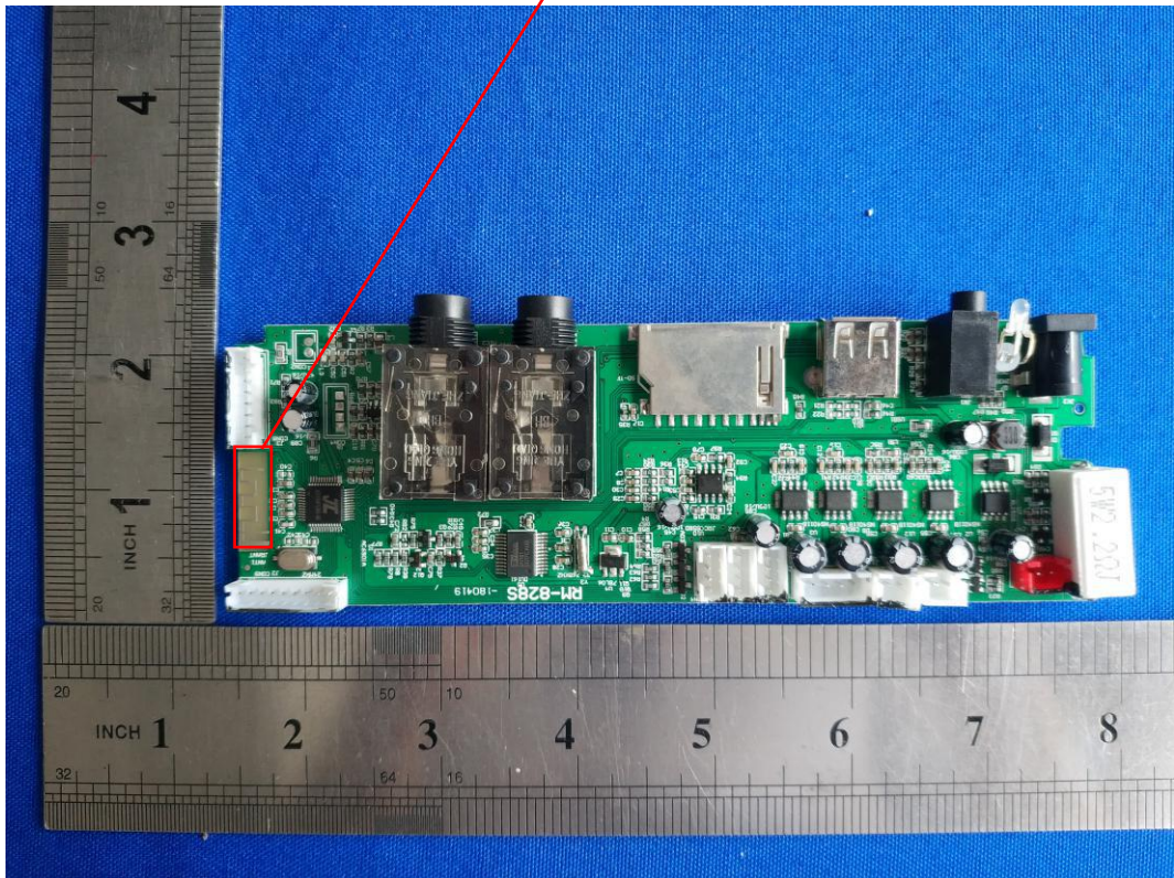
BT:PCB antenna
