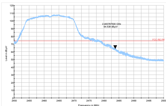
802.11g-Channel 11 Peak
