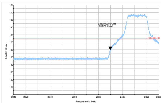
802.11g-Channel 1 Peak
