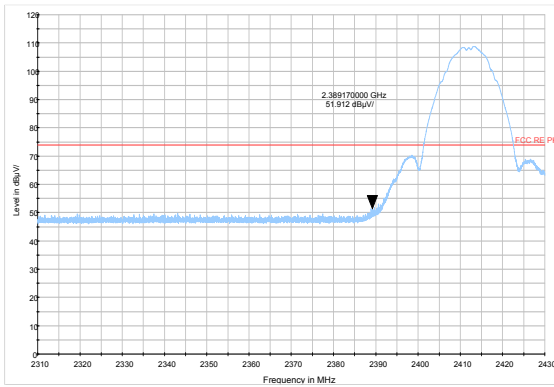
802.11b-Channel 1 Peak
