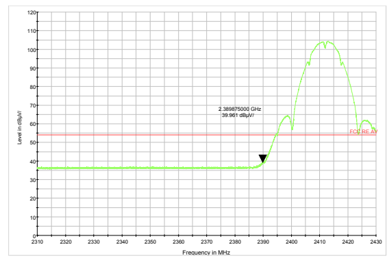
802.11b-Channel 1 Average
