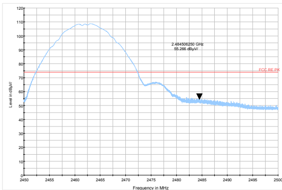
802.11b-Channel 11 Peak
