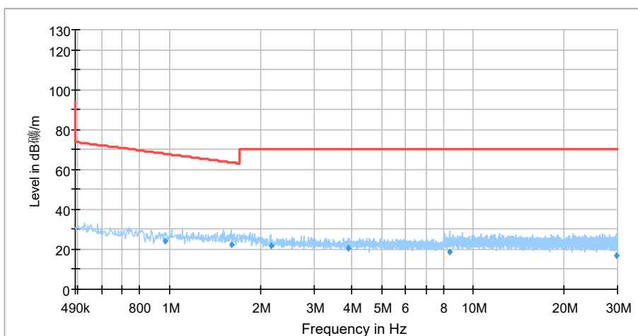
Radiates Emission from 490KHz to 30MHz
