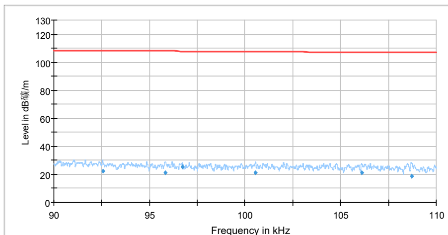
Radiates Emission from 90KHz to 110KHz
