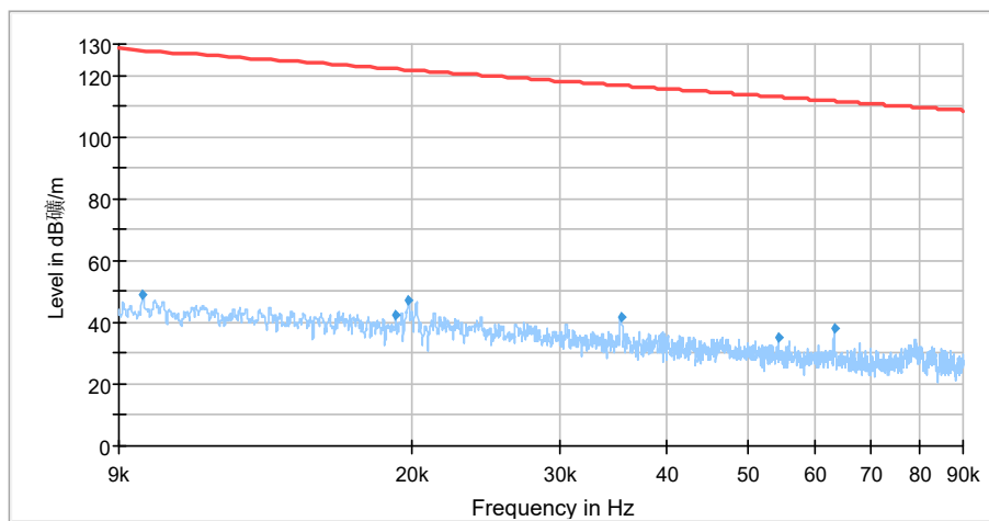
Radiates Emission from 9KHz to 90KHz
