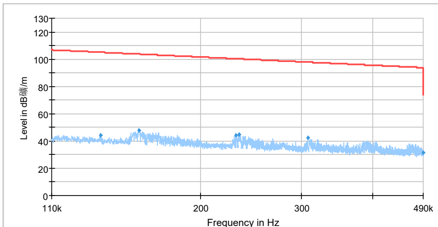
Radiates Emission from 110KHz to 490KHz
