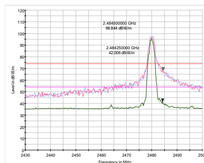
Bluetooth LE (1M) Channel 39 Peak+Average
