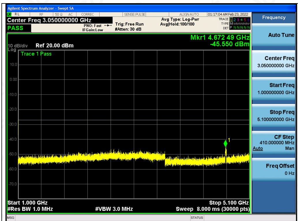
Test_Graph_802.11a_ANT2_5320_6Mbps_Frequency Band 2
