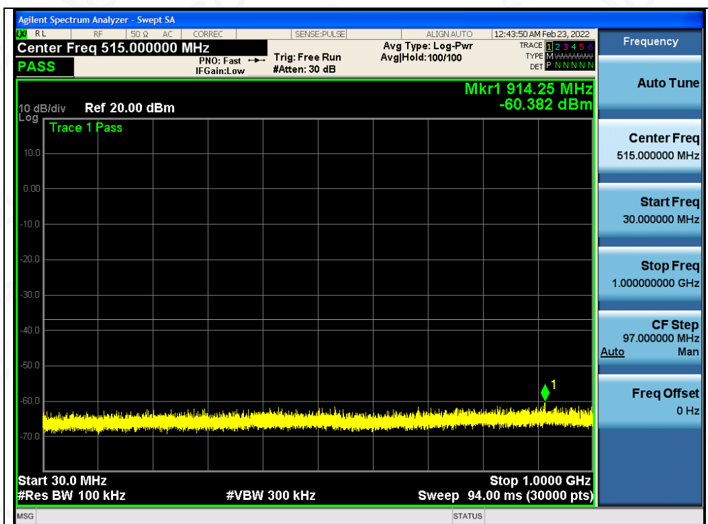
Test_Graph_802.11n40_ANT2_5190_MCS0_Frequency Band 1
