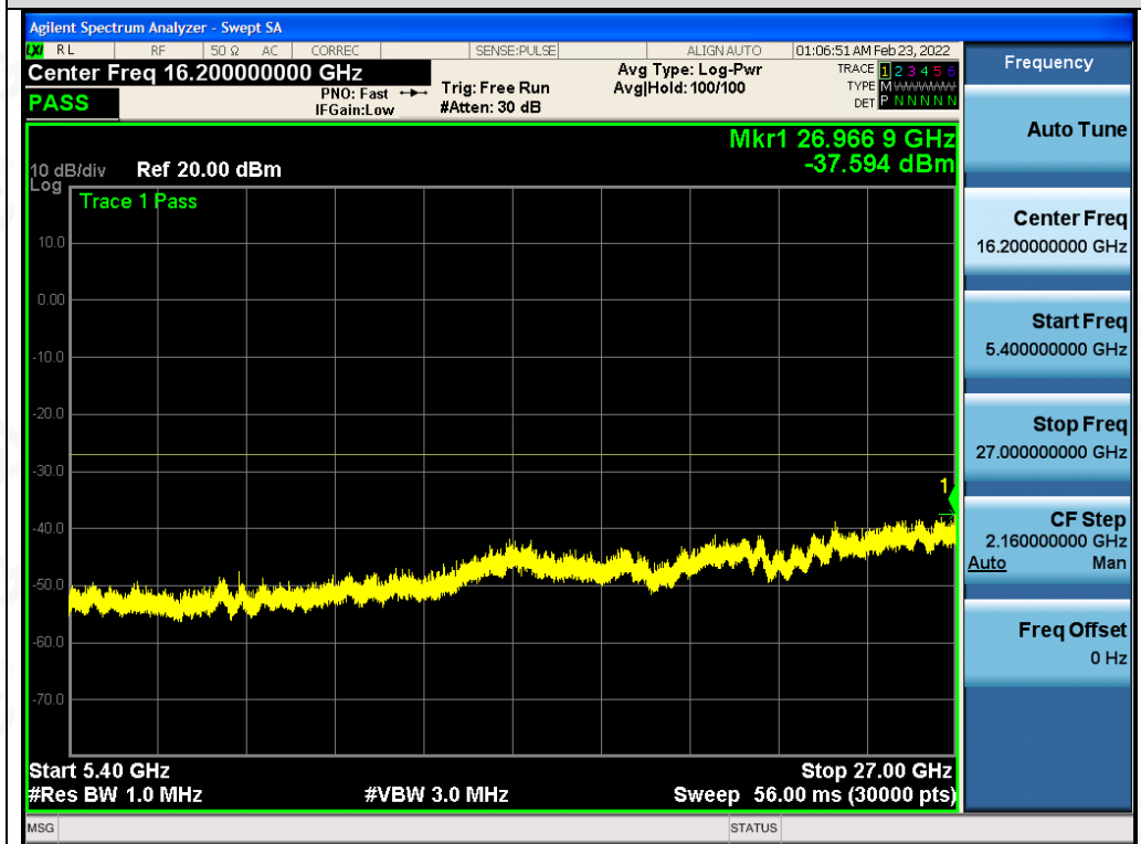
Test_Graph_802.11ac80_ANT2_5210_MCS9_Frequency Band 4
