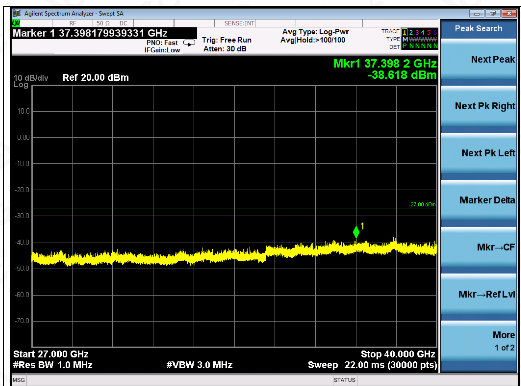
Test_Graph_802.11n40_ANT2_5190_MCS0_Frequency Band 5
