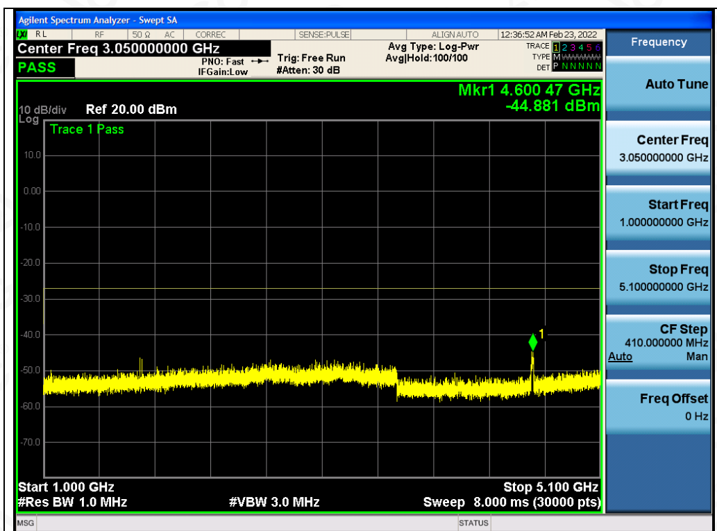
Test_Graph_802.11a_ANT2_5240_6Mbps_Frequency Band 2
