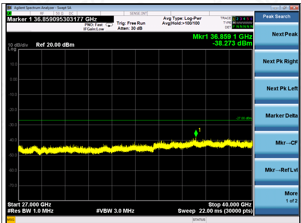
Test_Graph_802.11ac80_ANT1_5610_MCS9_Frequency Band 5
