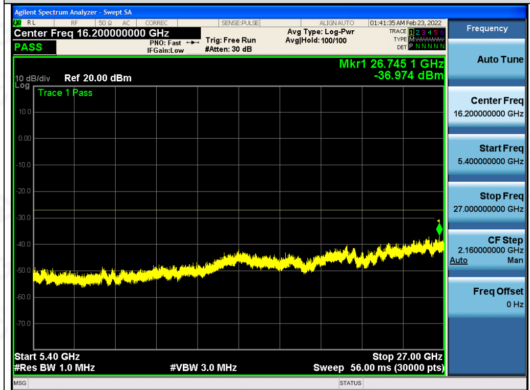
Test_Graph_802.11ac80_ANT2_5290_MCS9_Frequency Band 4
