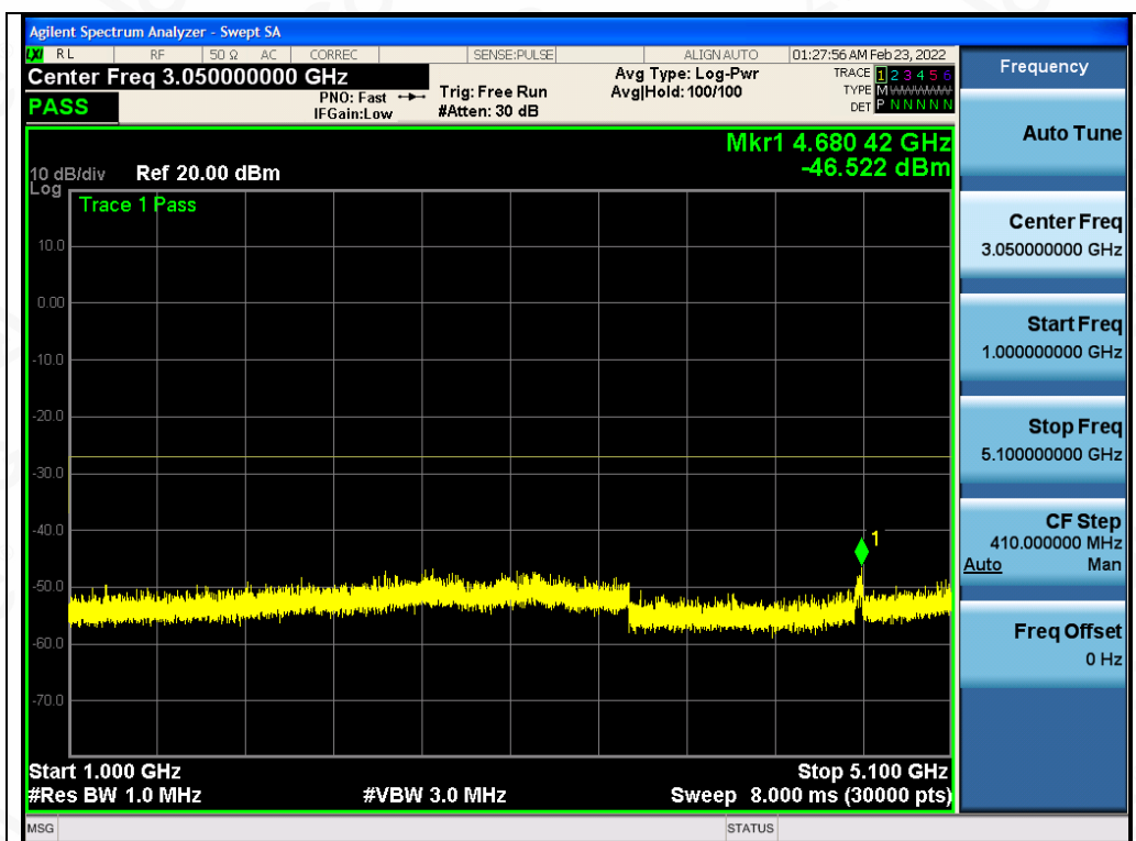
Test_Graph_802.11n40_ANT2_5310_MCS0_Frequency Band 2
