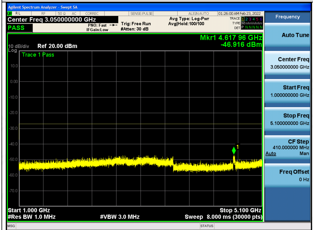
Test_Graph_802.11n40_ANT2_5270_MCS0_Frequency Band 2
