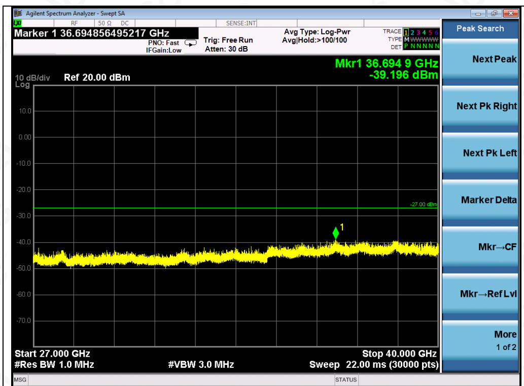
Test_Graph_802.11a_ANT2_5180_6Mbps_Frequency Band 5
