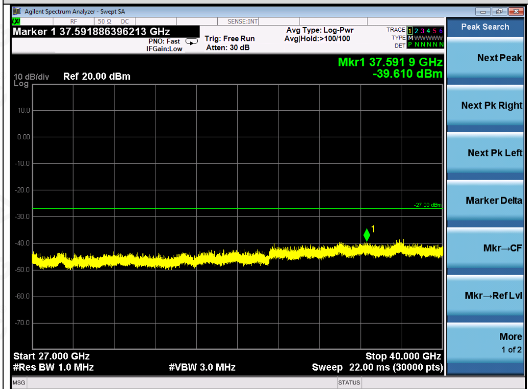
Test_Graph_802.11n40_ANT2_5230_MCS0_Frequency Band 5
