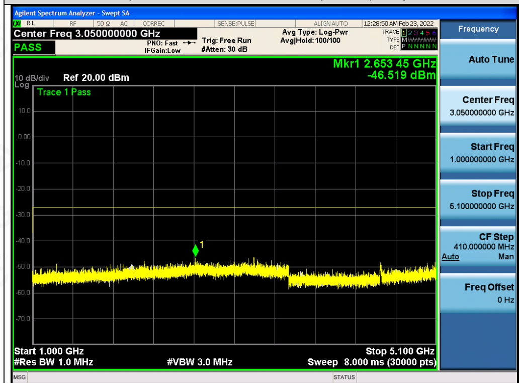
Test_Graph_802.11a_ANT2_5180_6Mbps_Frequency Band 2
