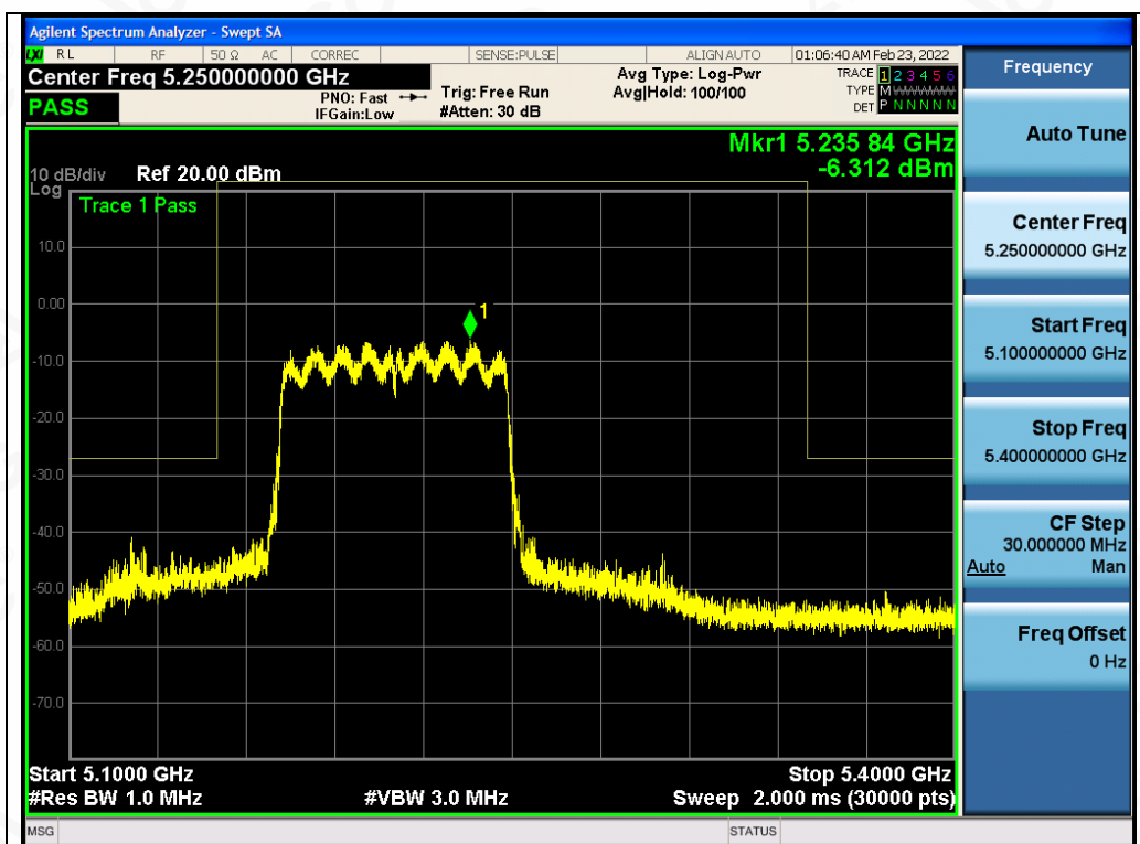
Test_Graph_802.11ac80_ANT2_5210_MCS9_Frequency Band 3
