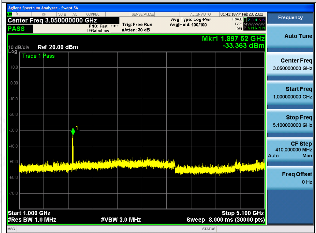
Test_Graph_802.11ac80_ANT2_5290_MCS9_Frequency Band 2
