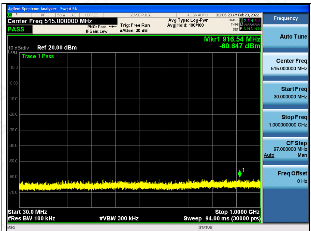
Test_Graph_802.11ac80_ANT2_5210_MCS9_Frequency Band 1
