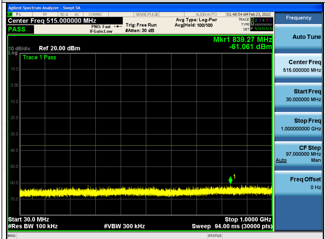
Test_Graph_802.11a_ANT2_5500_6Mbps_Frequency Band 1
