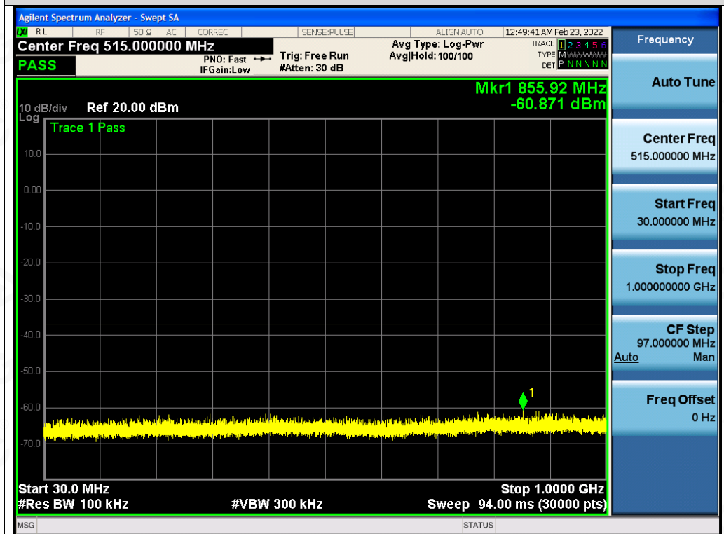
Test_Graph_802.11n40_ANT2_5230_MCS0_Frequency Band 1
