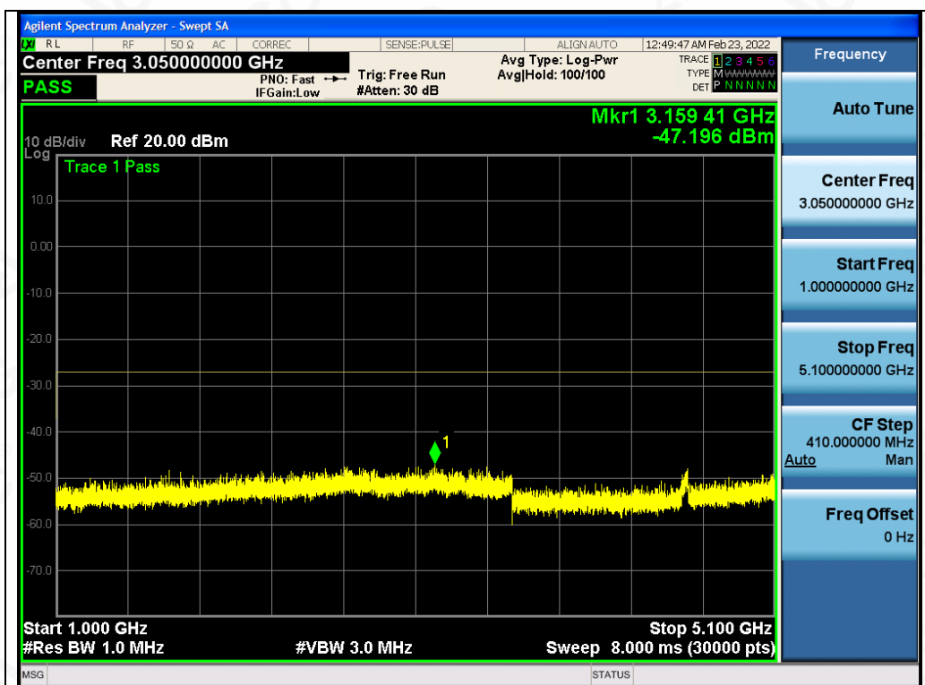
Test_Graph_802.11n40_ANT2_5230_MCS0_Frequency Band 2
