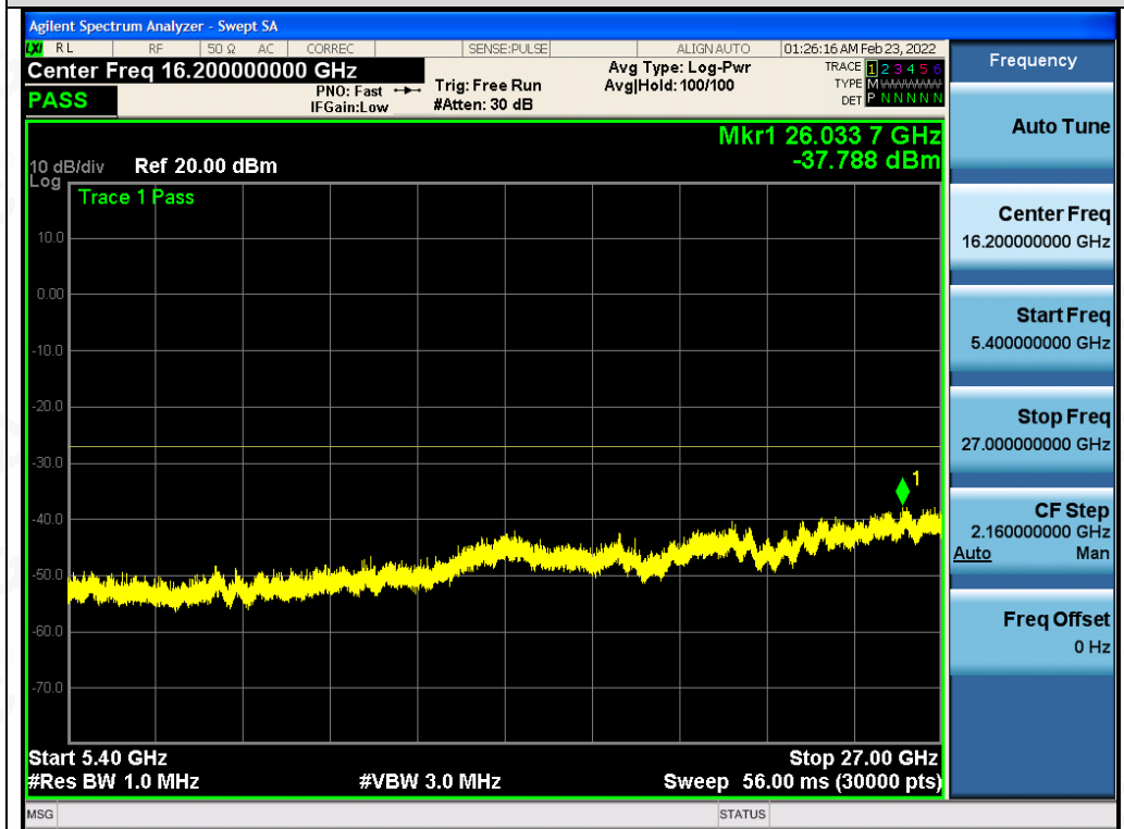
Test_Graph_802.11n40_ANT2_5270_MCS0_Frequency Band 4
