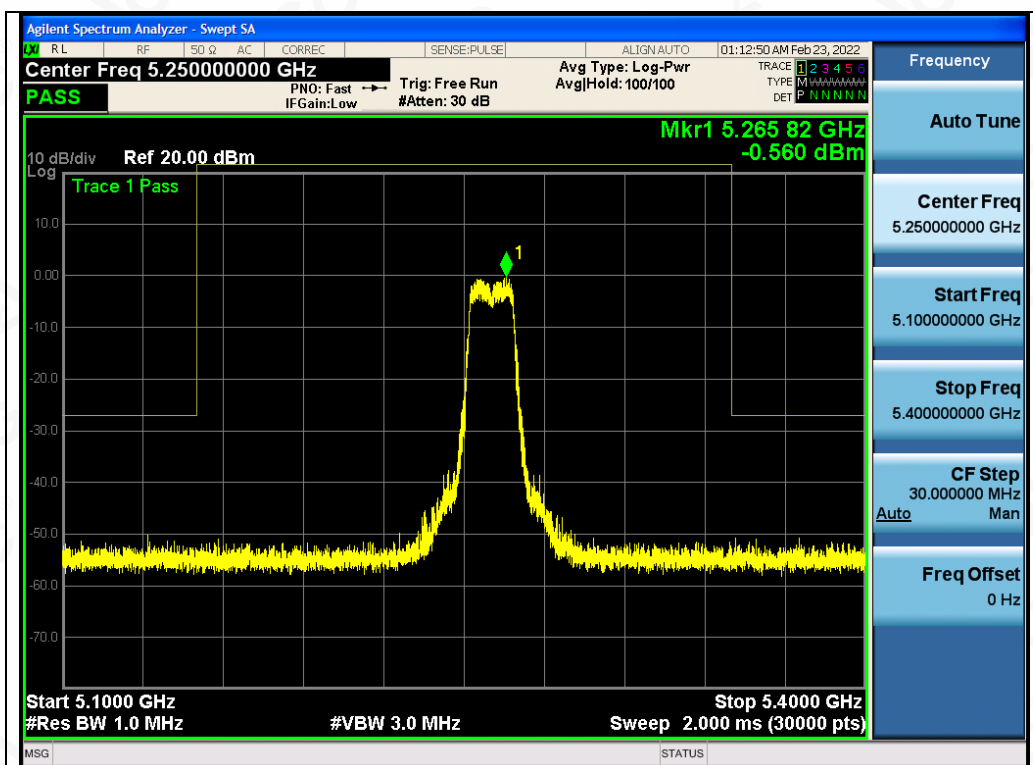
Test_Graph_802.11a_ANT2_5260_6Mbps_Frequency Band 3
