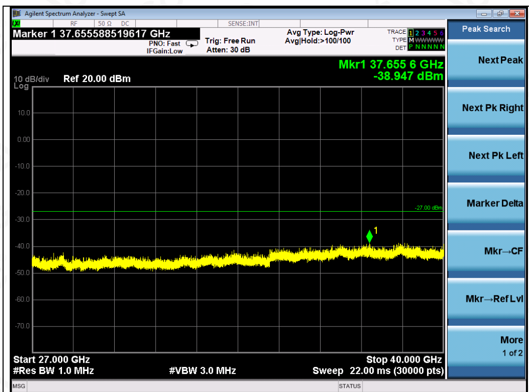
Test_Graph_802.11n40_ANT2_5270_MCS0_Frequency Band 5
