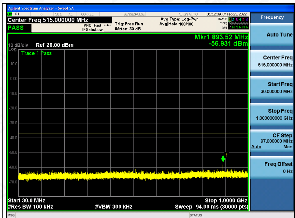
Test_Graph_802.11a_ANT2_5260_6Mbps_Frequency Band 1
