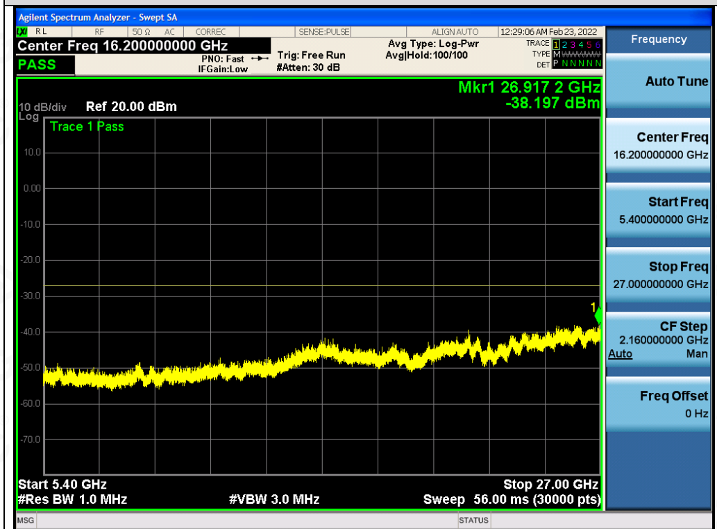
Test_Graph_802.11a_ANT2_5180_6Mbps_Frequency Band 4
