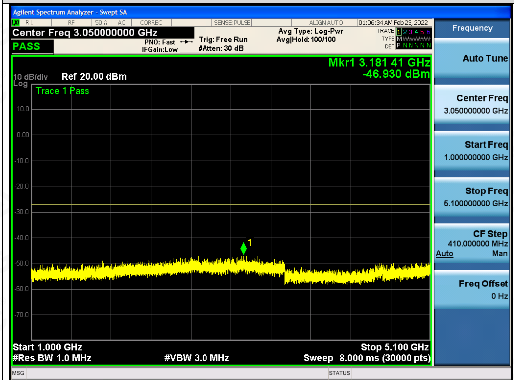
Test_Graph_802.11ac80_ANT2_5210_MCS9_Frequency Band 2
