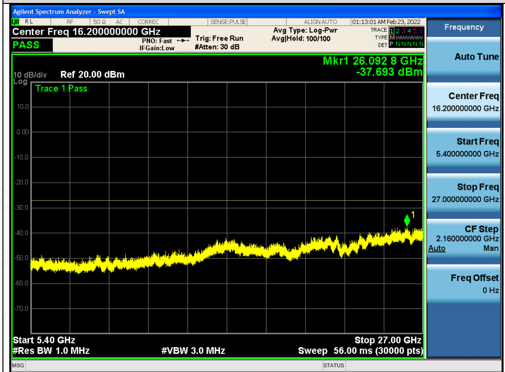
Test_Graph_802.11a_ANT2_5260_6Mbps_Frequency Band 4
