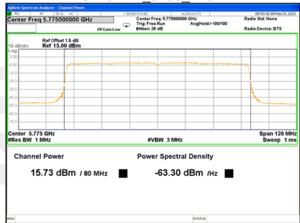
5775MHz_ax80_Ant A
