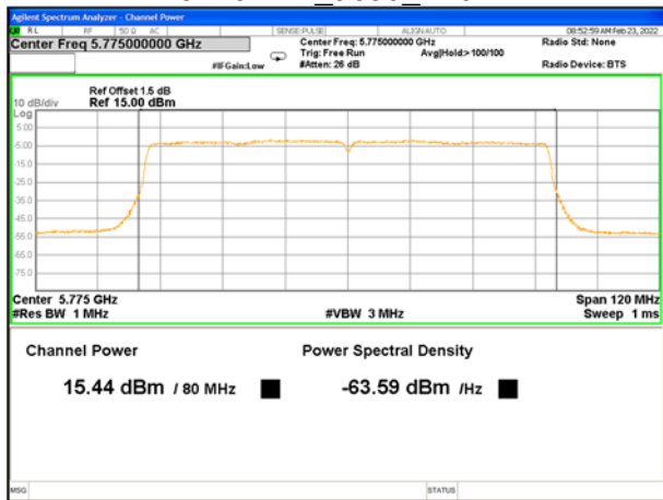
5775MHz_ac80_Ant A
