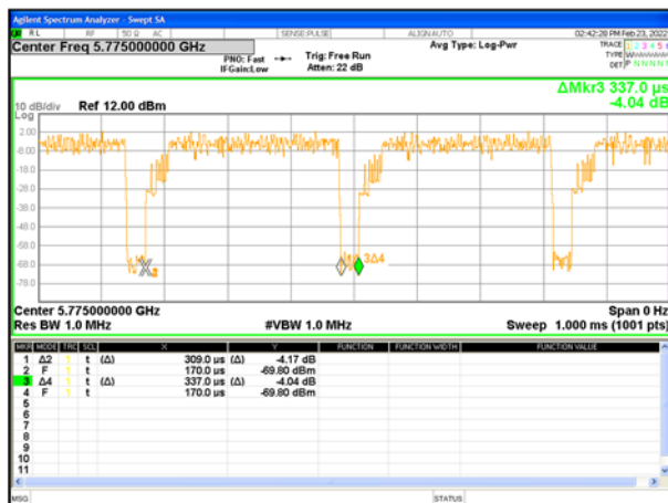
Band 4-ax80
