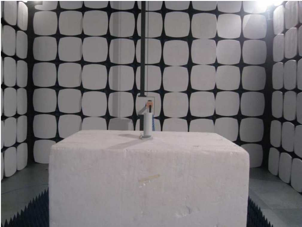
Radiated Measurement Photos (18GHz-26.5GHz)
