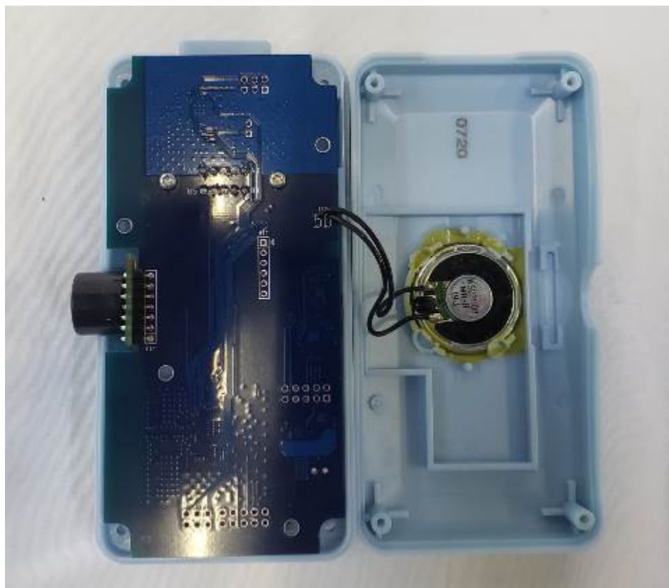
Figure 3. Back Cover Removed
