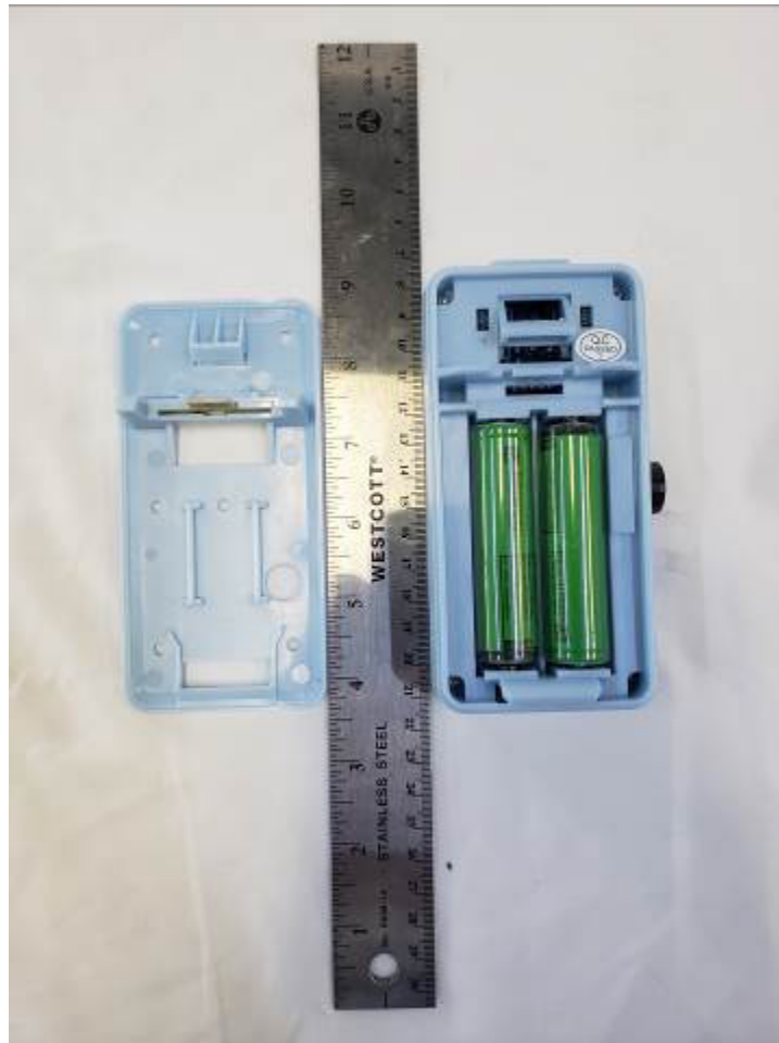
Figure 1. Mounting wall plate removed (Back of EUT exposed)
