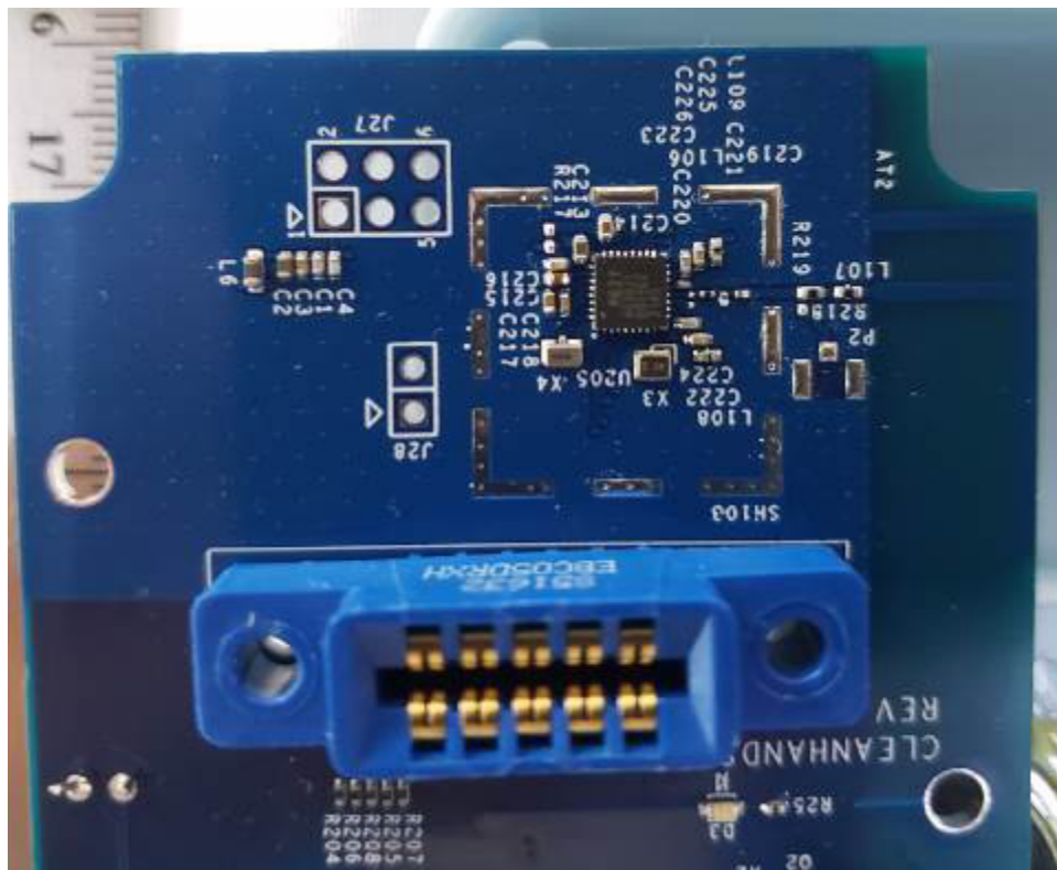
Figure 7. Close up of Bluetooth Module
