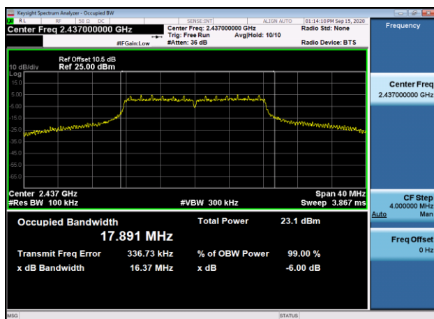
6dB Bandwidth-802.11g,2437MHz
