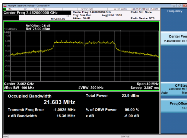
6dB Bandwidth-802.11g,2462MHz
