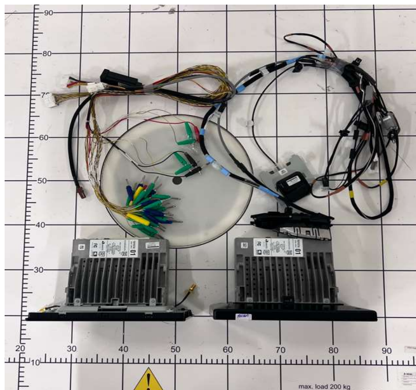
Figure B4. DUT's with Accessories
