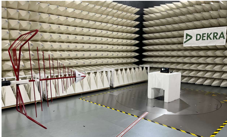
Figure B5. Low Range Radiated Emission test setup
