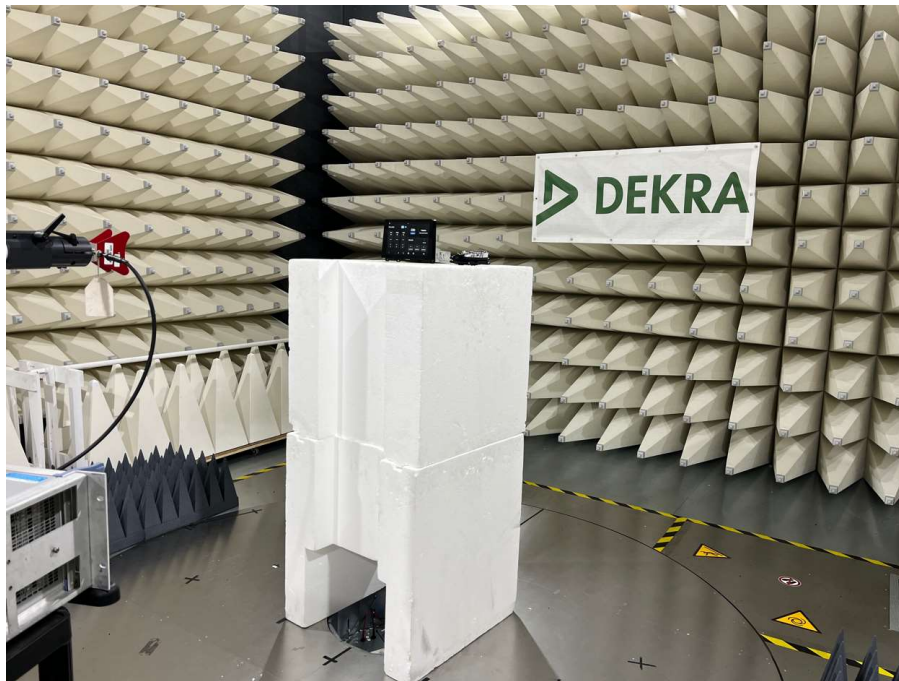
Figure B7. High Range Radiated Emission test setup 18-40 GHz
