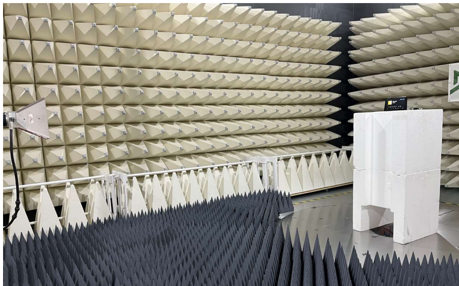
Figure B6. High Range Radiated Emission test setup 1-18 GHz
