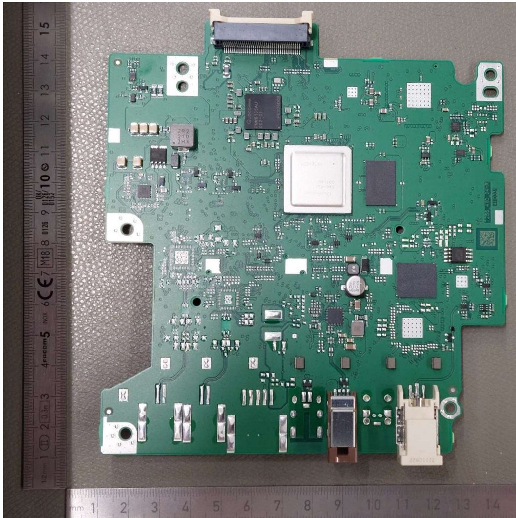
PCB 2 – Top
