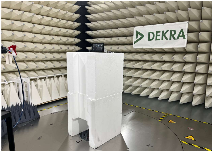
Figure B7. High Range Radiated Emission test setup 18-40 GHz
