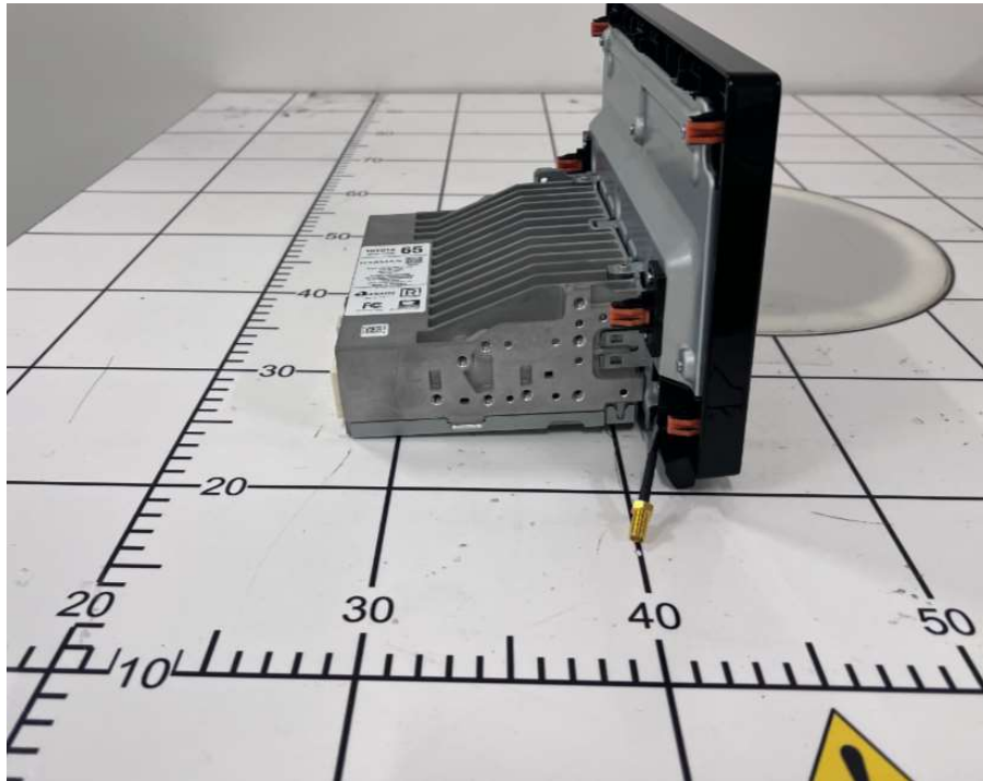
Figure B3. Side View of DUT
