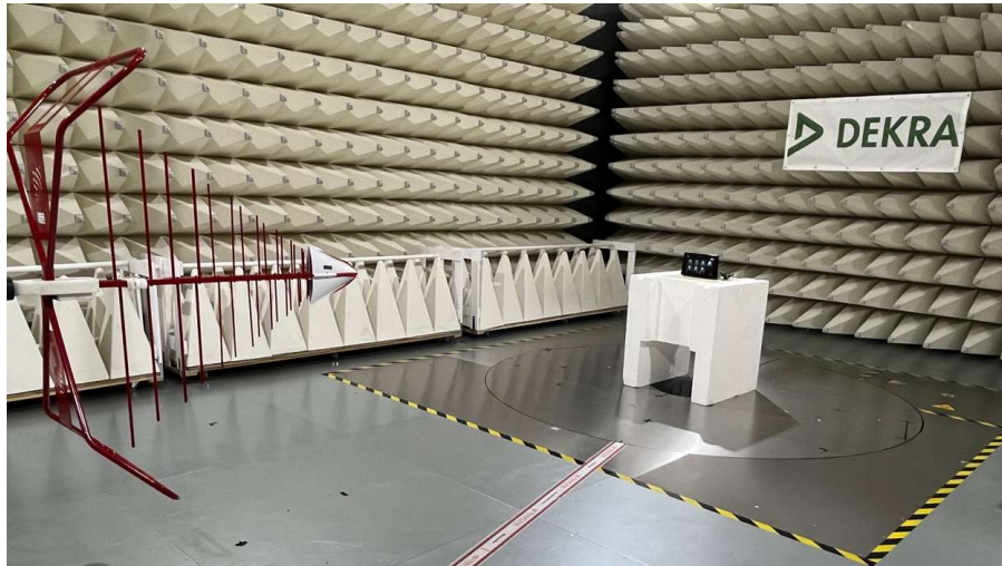
Figure B5. Low Range Radiated Emission test setup
