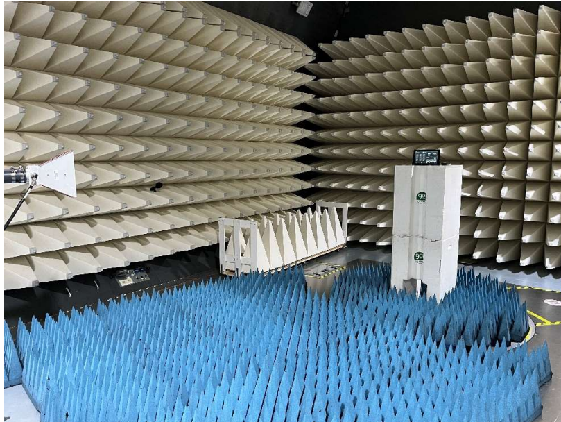
Figure B6. High Range Radiated Emission test setup 1-18GHz
