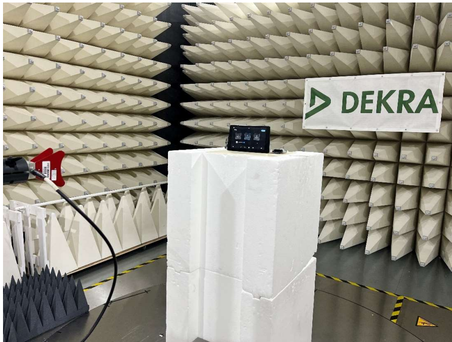
Figure B7. High Range Radiated Emission test setup 18-26GHz
