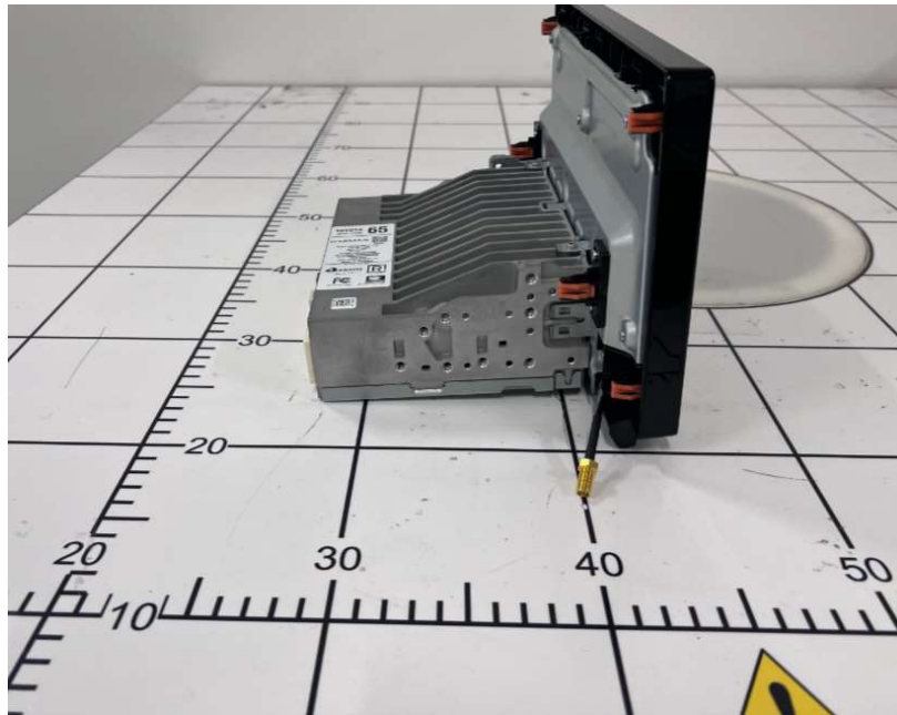
Figure C3. Side View of DUT
