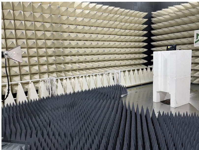
Figure C6. High Range Radiated Emission test setup 1-18GHz
