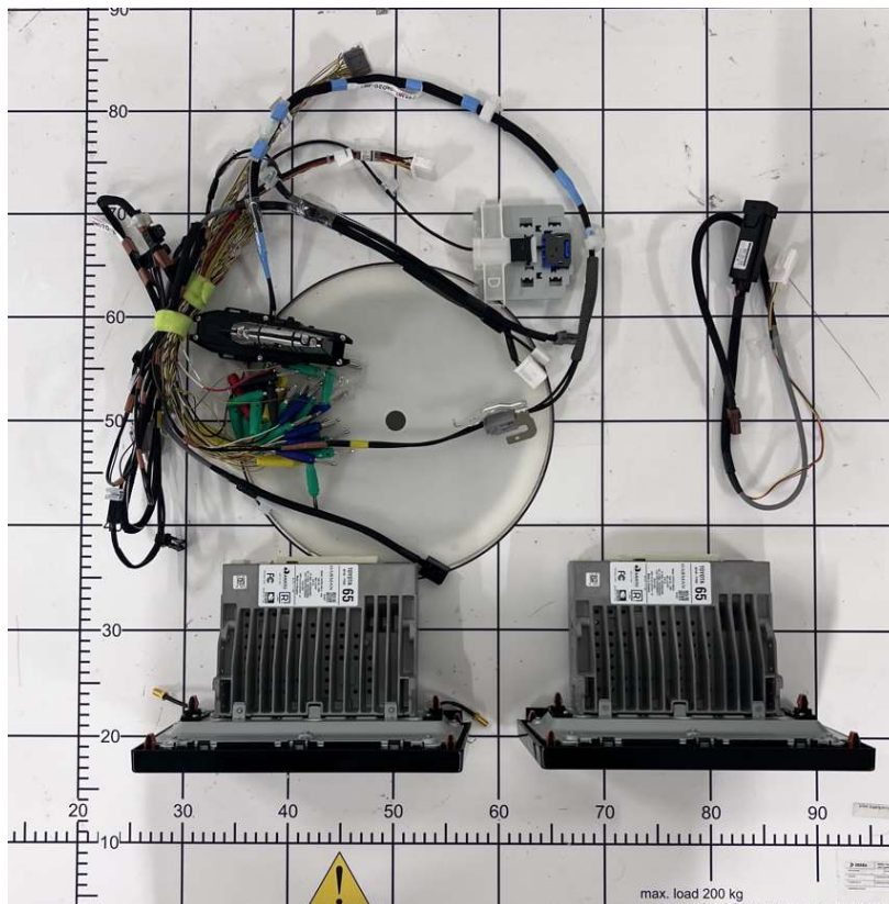
Figure C4. Front View of Conducted and Radiated samples with Accessories
