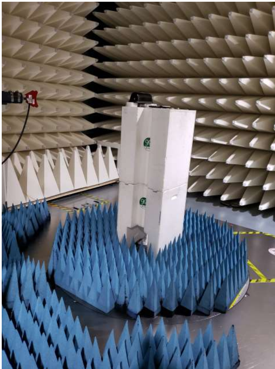
9. High Range Radiated Emission test setup
