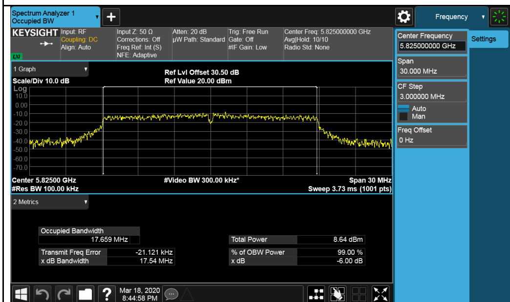
802.11n-HT20-5825MHz
