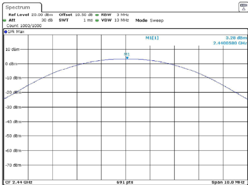
BLE_1M_Middle_Channel
