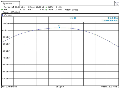
BLE_1M_Low_Channel
