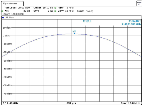
BLE_1M_High_Channel
